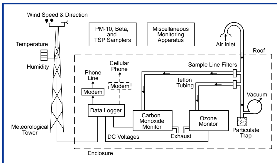
Figure 4. Block diagram of an ambient air monitoring station
