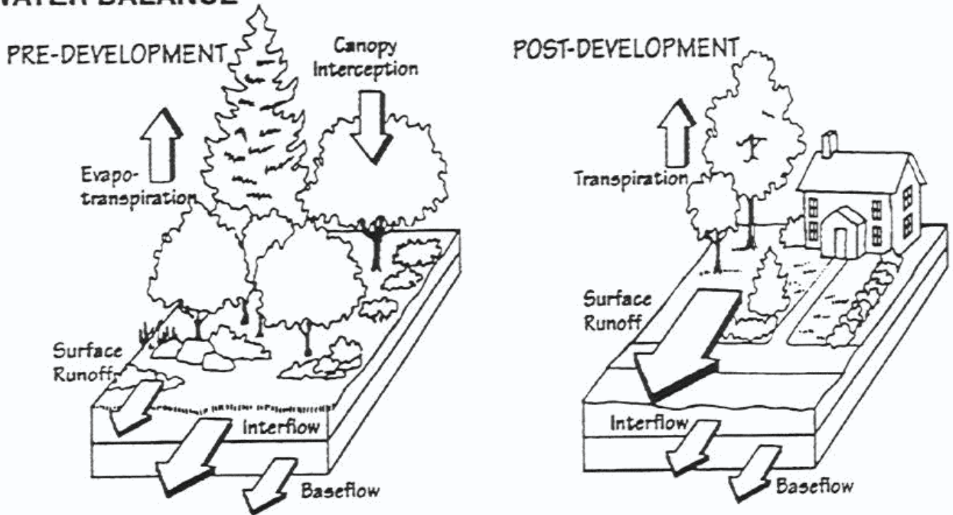
Figure 2-2 Water Balance at a Developed and Undeveloped Site (Source: Maryland Department of the Environment [MDE], 2000)
