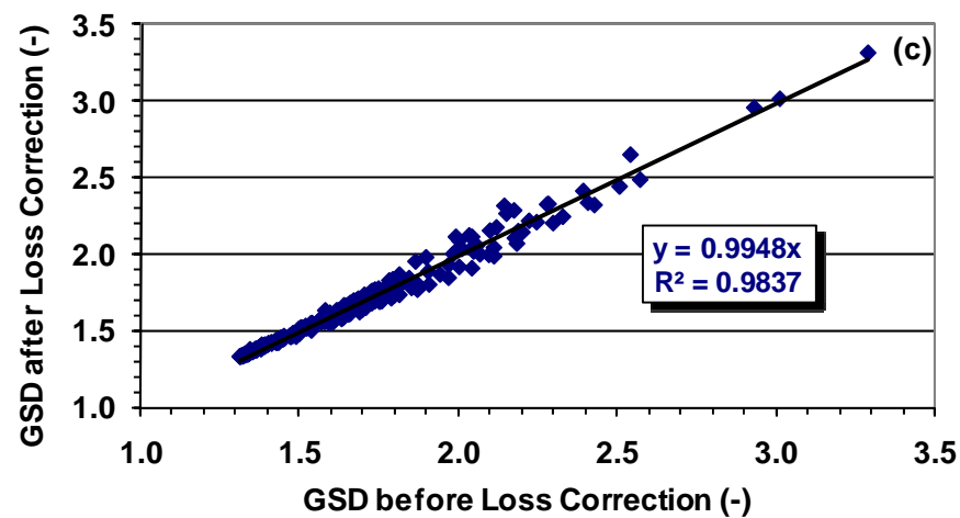
Figure 10-26. Comparison of total particle number, GMD and GSD before and after loss correction for all tests conducted based on: (a) total particle concentration and (b) GMD and (c) GSD.
