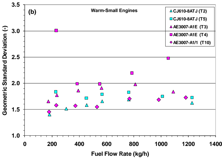
Figure 10-33. The (a) GMD and (b) GSD of the PM emissions measured for the small engines during APEX-3 as a function of fuel flow. Engines operated during the warm portion of the test cycle.
