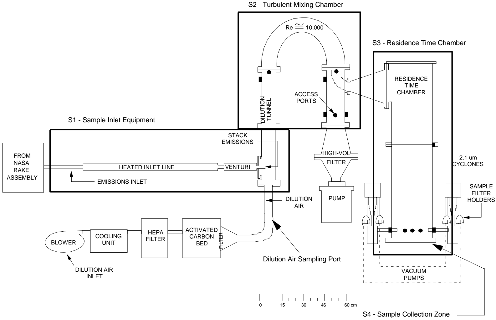
Figure A-2. APEX 1- Schematic Diagram of the Dilution Sampling Unit and its Major Components
