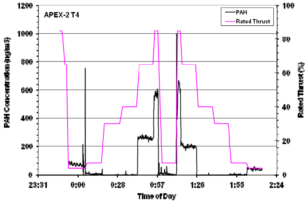
Figure 11-24. Time-series PAH concentration data for tests T1 and T4 of APEX-2 campaign for the CFM56-7B24 engine.
