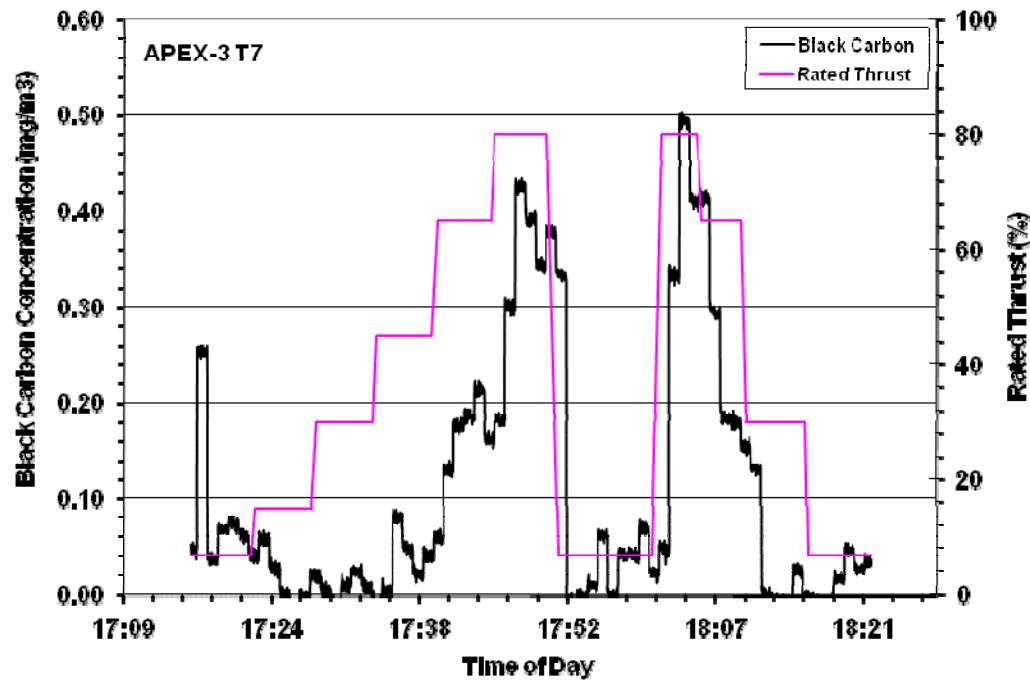
Figure 11-7. Time-series black carbon concentration data for the APEX-3 T6 and T7 for the P&W 4158 engine.
