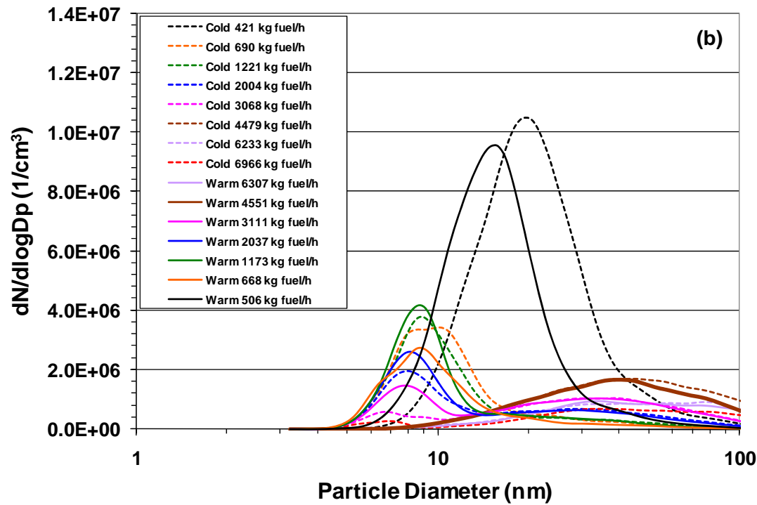
Figure 10-22. Average PSD for a RB211-535E4B engine measured by the Nano-SMPS during APEX-3, Test T9, (a) with line loss correction; and (b) without line loss correction.
