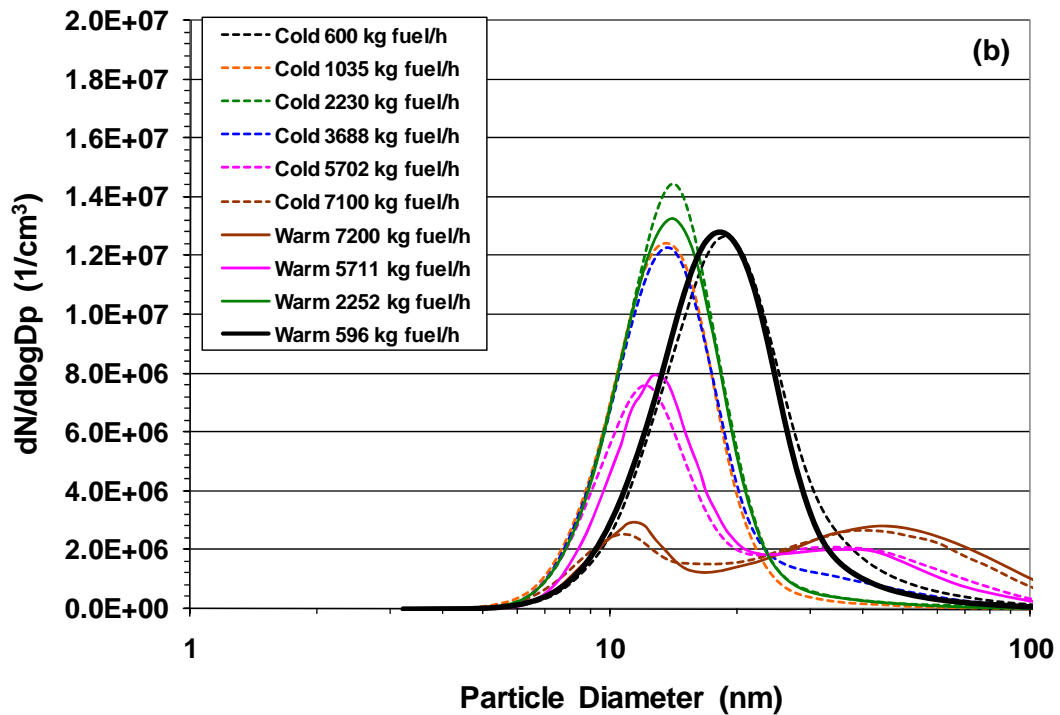
Figure 10-20. Average PSD for a PW4158 engine measured by the Nano-SMPS during APEX-3, Test T7, (a) with line loss correction; and (b) without line loss correction.
