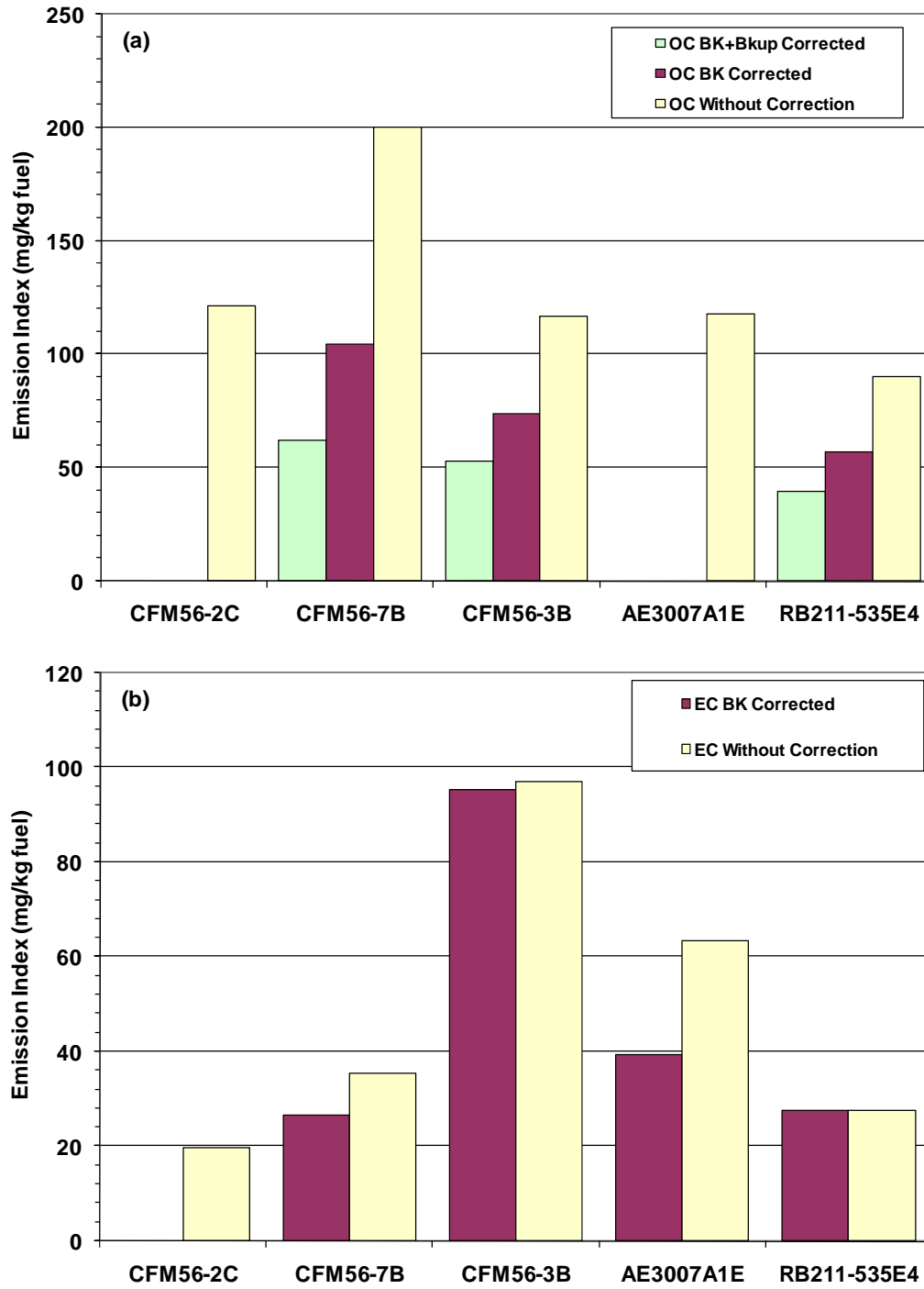
Figure 13-7. Comparison of OC and EC emission indices for: (a) organic carbon; and (b) elemental carbon.
