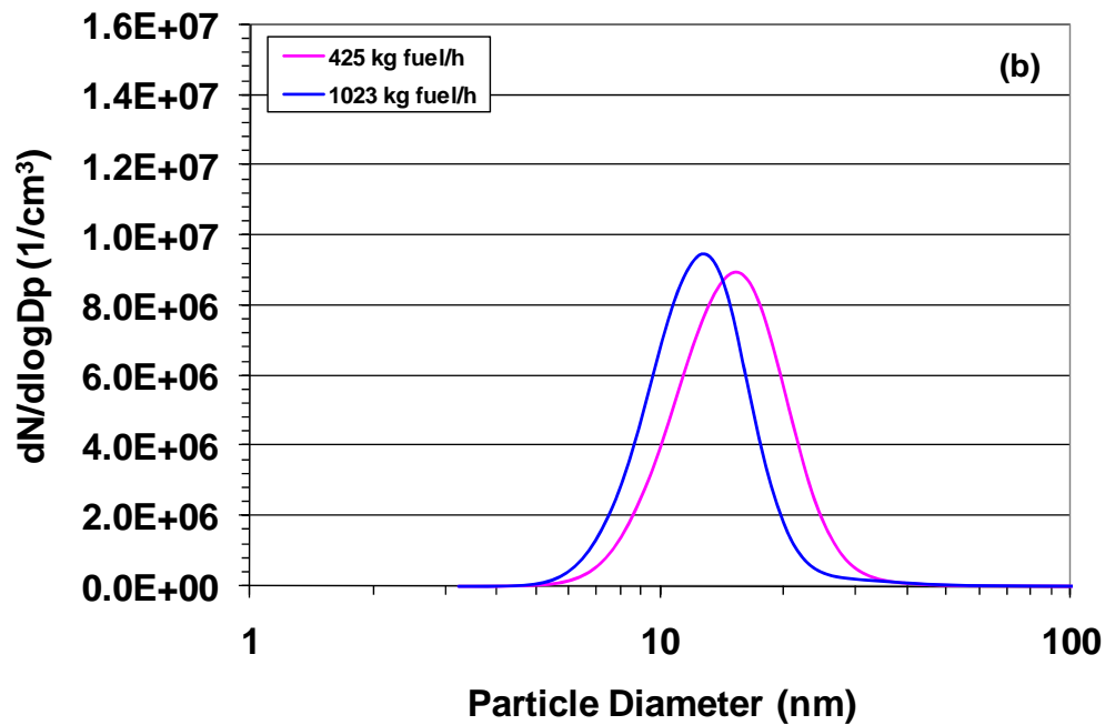
Figure 10-2. Average PSD measured by the Nano-SMPS during APEX-1, Test EPA-2, (a) with line loss correction; and (b) without line loss correction.
