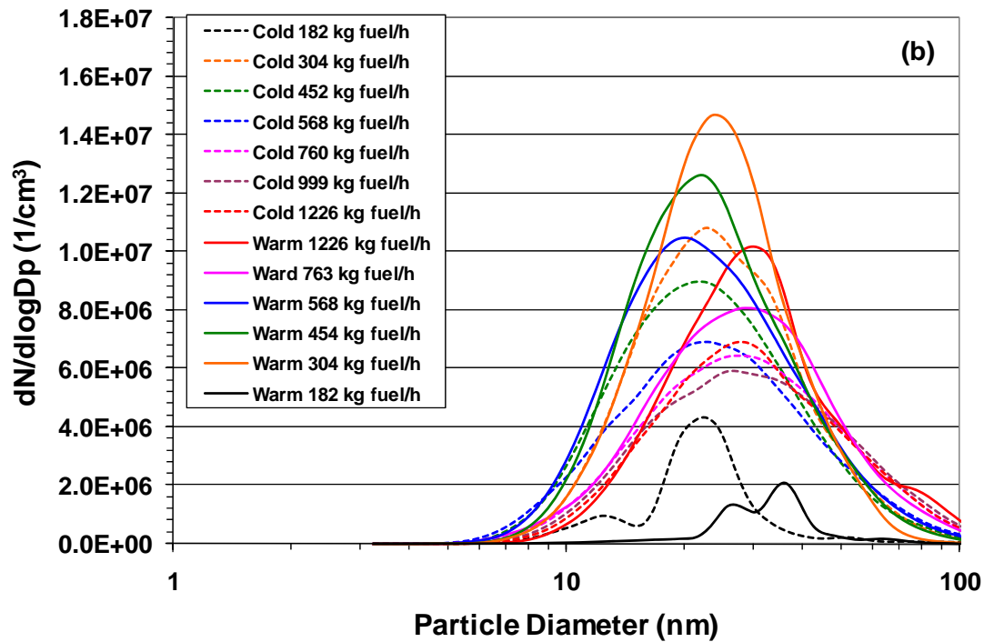
Figure 10-15. Average PSD for a CJ610-8ATJ turbojet engine measured by the Nano-SMPS during APEX-3, Test T2, (a) with line loss correction; and (b) without line loss correction.
