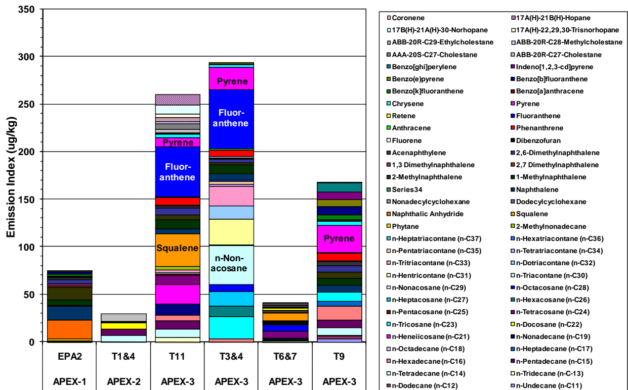
Figure 13-8. Relative contribution of individual organic compounds to the total speciated particle-phase EI.
