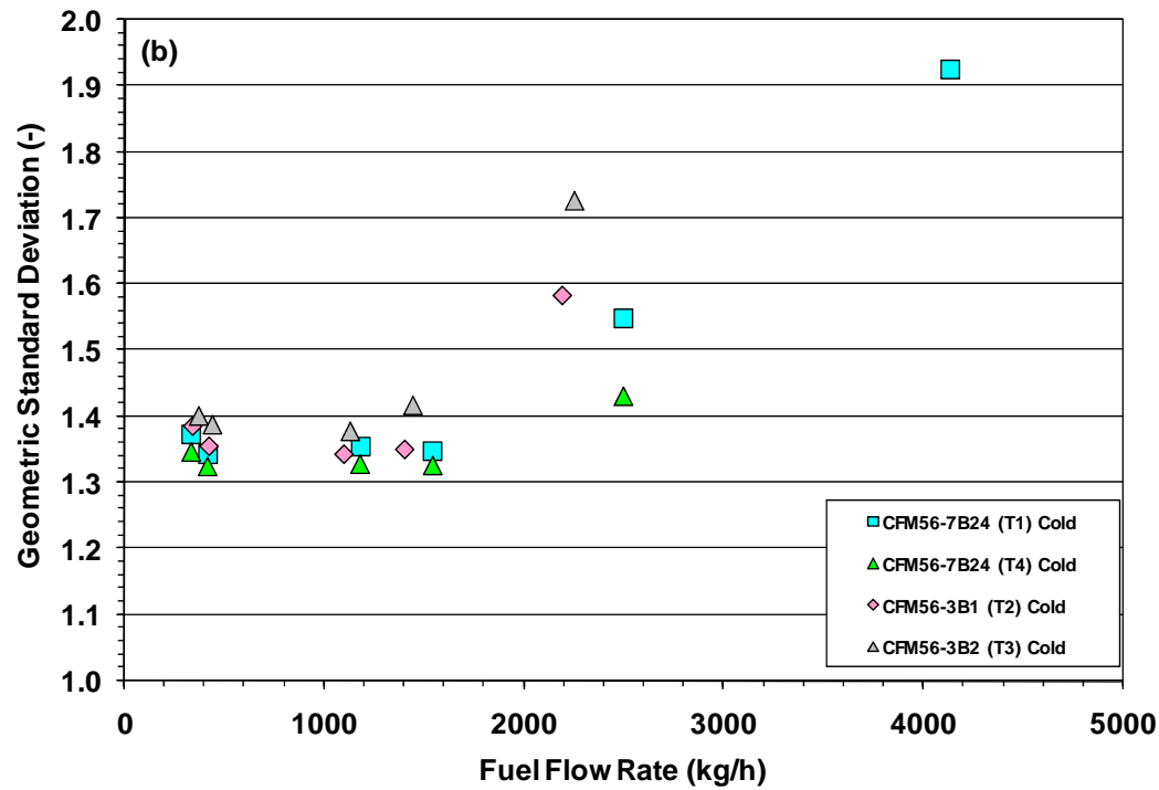
Figure 10-29. The (a) GMD and (b) GSD of the PM emissions measured for three derivatives of the CFM56 engine during APEX-2 as a function of fuel flow. Engines operated during cold portion of test cycle.
