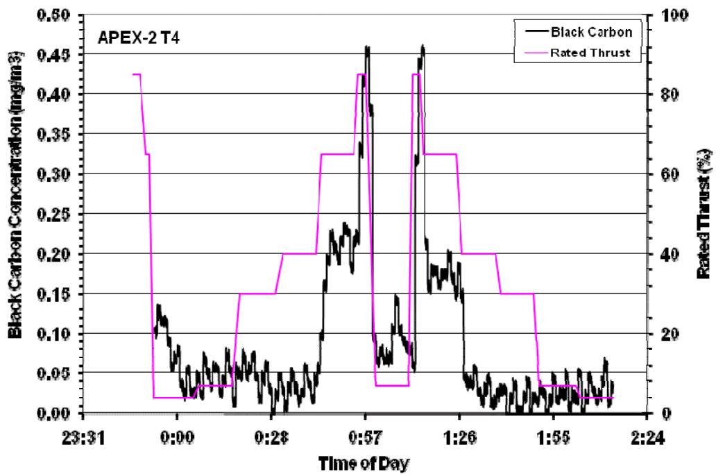
Figure 11-3. Time-series black carbon concentration data for the tests T1 and T4 of APEX-2 campaign for the CFM56-7B24 engine.
