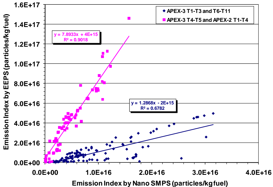
Figure 9-14. Comparison of particle number emission indices as obtained from the Nano-SMPS and EEPS instruments.
