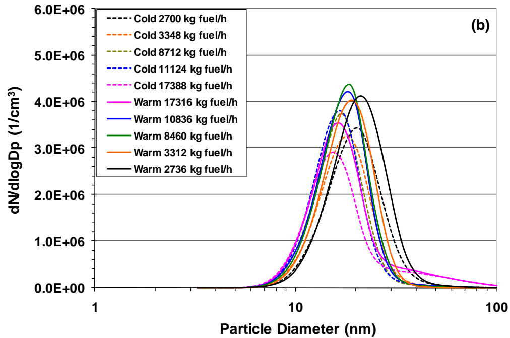
Figure 10-11. Average PSD for a CFM56-3B1 engine measured by the Nano-SMPS during APEX-2, Test T2, (a) with line loss correction; and (b) without line loss correction.
