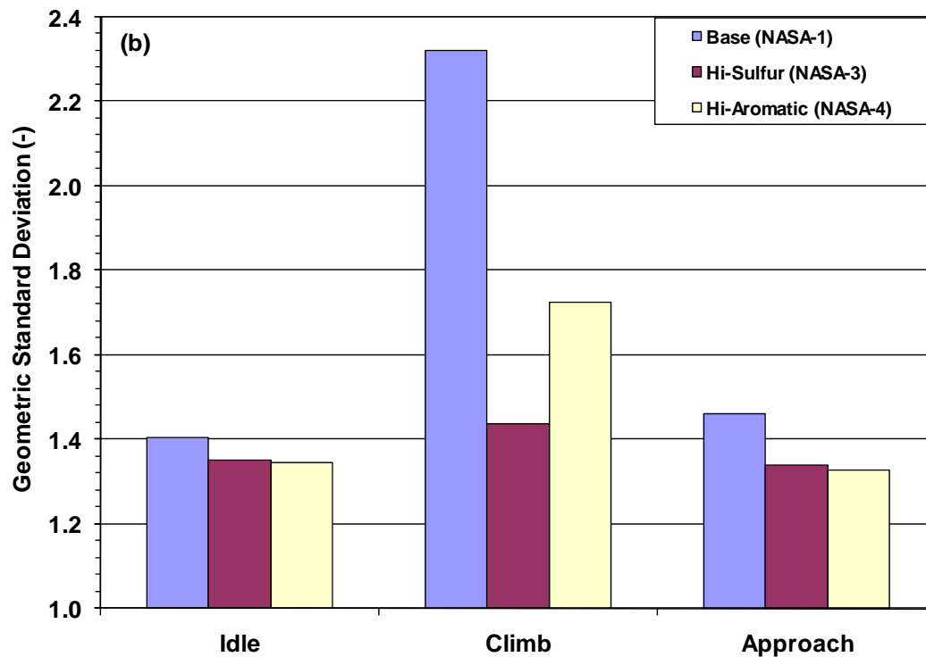
Figure 10-37. Comparison of the loss-corrected: (a) GMDs; and (b) GSDs for different power conditions and fuels during APEX-1.
