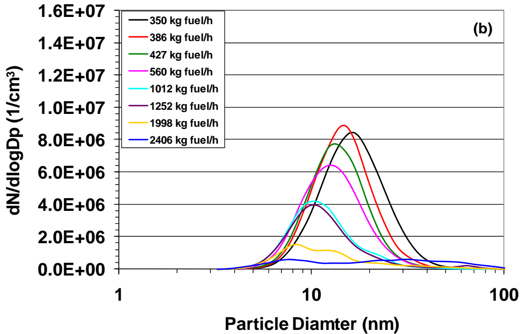
Figure 10-4. Average PSD measured by the Nano-SMPS during APEX-1, Test NASA-1, (a) with line loss correction; and (b) without line loss correction.
