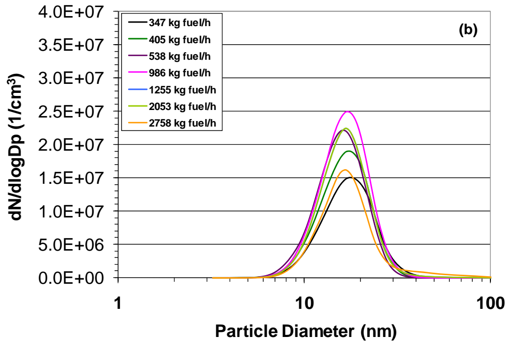
Figure 10-7. Average PSD measured by the Nano-SMPS during APEX-1, Test NASA-3, (a) with line loss correction; and (b) without line loss correction.
