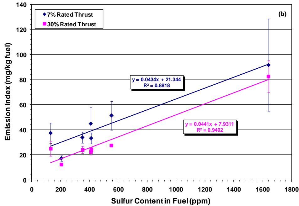
Figure 8-11. Effects of fuel type on: (a) mass emission index (CFM56-2C1) and (b) mass EI as a function of fuel sulfur (all CFM56 derivatives). Based on Nano-SMPS loss-corrected results.
