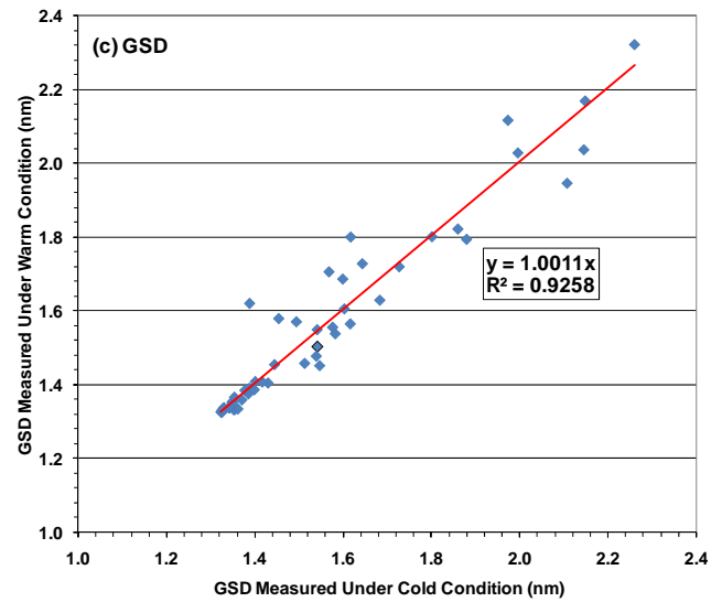
Figure 10-42. Effect of engine operating temperature on: (a) PM number concentration; (b) GMD; and (c) GSD.
