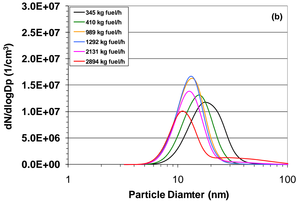
Figure 10-9. Average PSD measured by the Nano-SMPS during APEX-1, Test NASA-5, (a) with line loss correction; and (b) without line loss correction.
