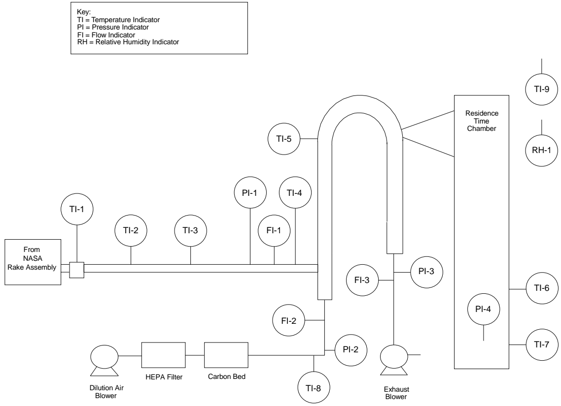
Figure A-3. APEX 1 - Instrumentation for Control of the DSS
