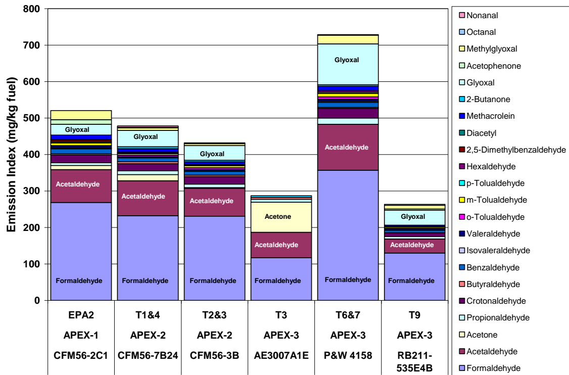
Figure 12-2. Mass EIs of individual carbonyl compounds from DNP cartridge sampling.
