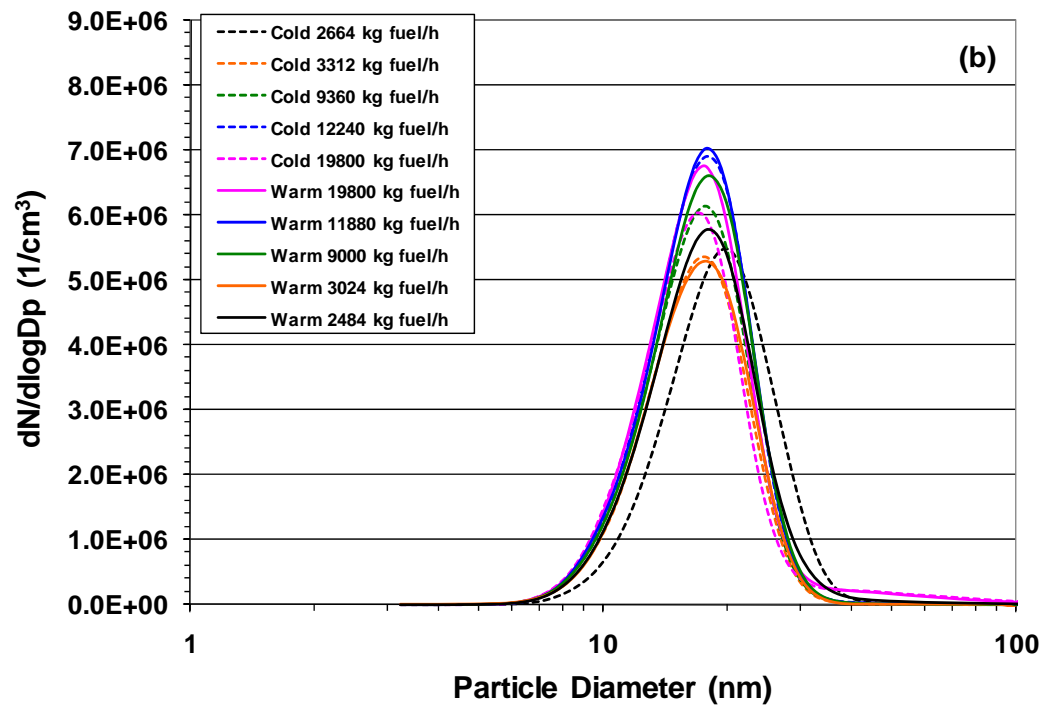
Figure 10-13. Average PSD for a CFM56-7B24 engine measured by the Nano-SMPS during APEX-2, Test T4, (a) with line loss correction; and (b) without line loss correction.
