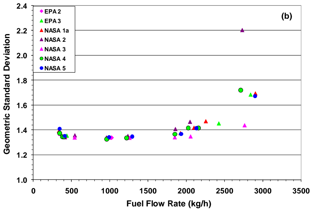
Figure 10-28. The (a) GMD and (b) GSD of the PM emissions measured during APEX-1 for a CFM56-2C1 engine as a function of fuel flow.
