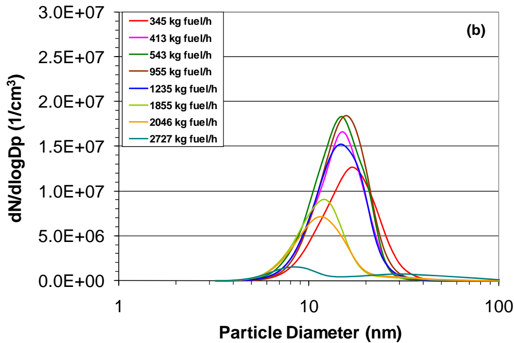
Figure 10-6. Average PSD measured by the Nano-SMPS during APEX-1, Test NASA-2, (a) with line loss correction; and (b) without line loss correction.
