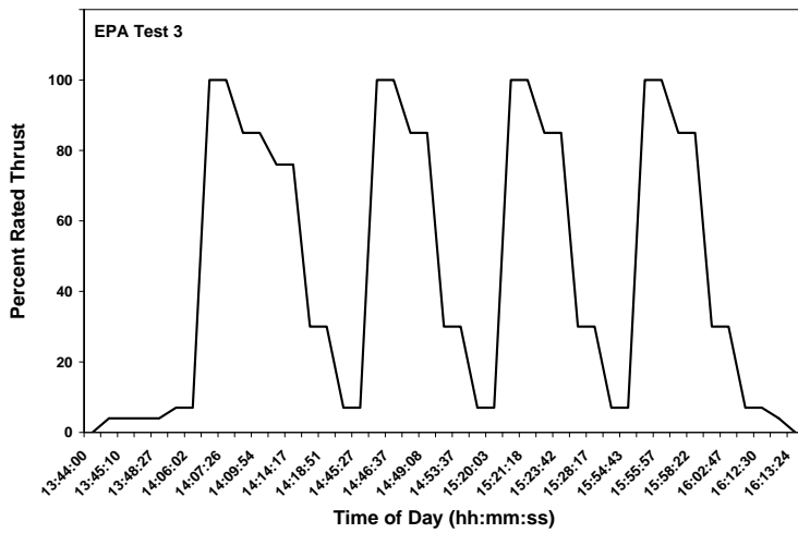
Figure 6-2. Engine operating cycles for the EPA tests during APEX-1.
