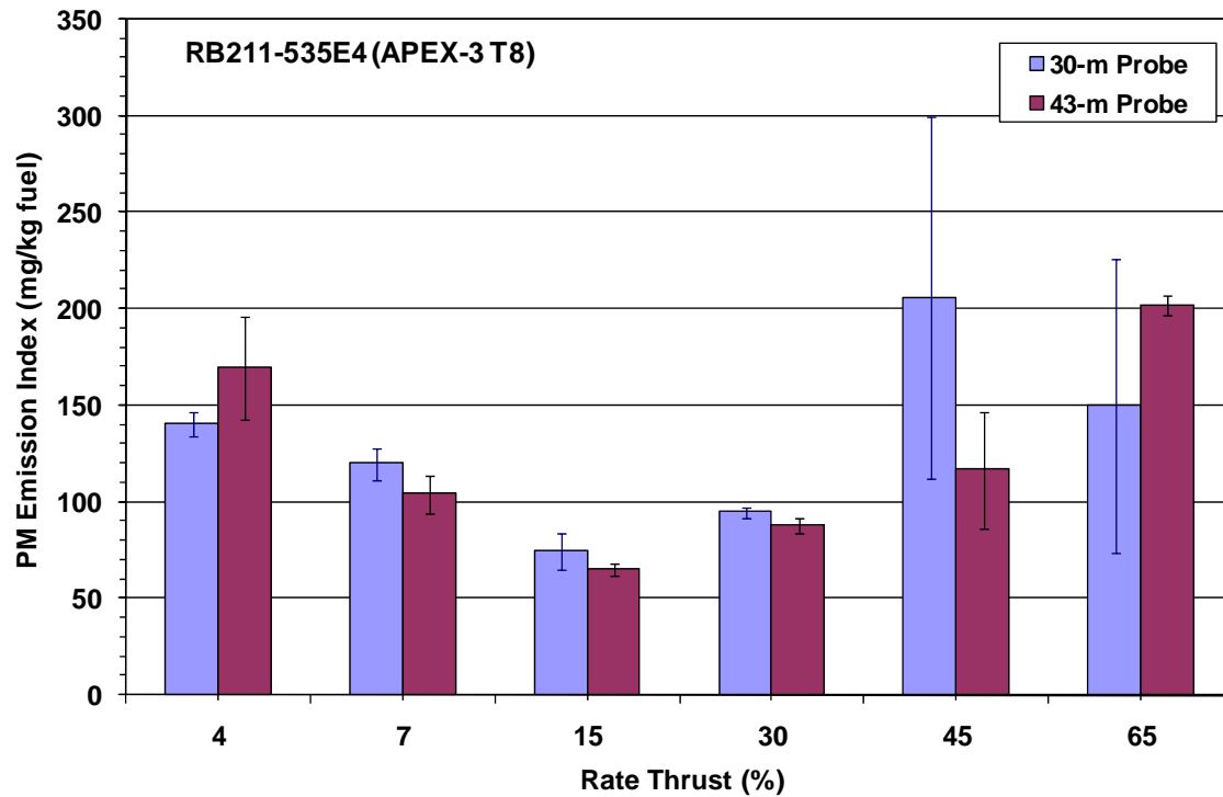
Figure 10-46. Effects of probe position on particle mass emission indices for a: CJ610-8ATJ turbojet; and RB211-535E4B turbofan engine.
