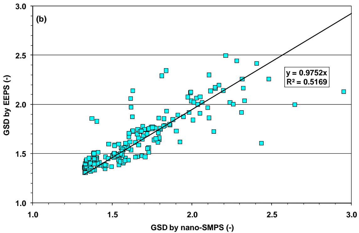
Figure 10-47. Comparison of the GMD and GSD as obtained from Nano-SMPS and EEPS measurements during all tests conducted during APEX-2 and -3.
