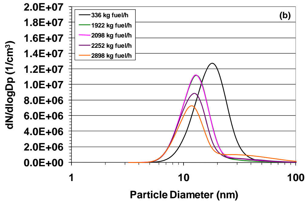
Figure 10-5. Average PSD measured by the Nano-SMPS during APEX-1, Test NASA-1a, (a) with line loss correction; and (b) without line loss correction.
