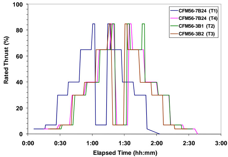
Figure 6-5. Engine operating cycles for APEX-2.
