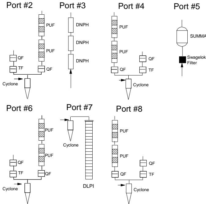
Figure A-4. APEX 1, DSS Sampling Array Configuration for Speciated Testing, Engine Exit Plane
