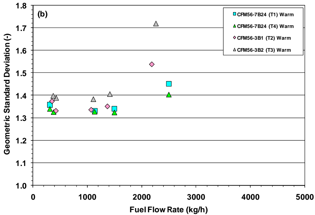
Figure 10-30. The (a) GMD and (b) GSD of the PM emissions measured for three derivatives of the CFM56 engine during APEX-2 as a function of fuel flow. Engines operated during warm portion of test cycle.
