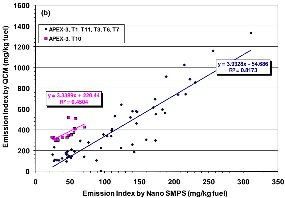
Figure 8-16. Comparison of the mass emissions indices between the Nano-SMPS and QCM for: (a) APEX-2 tests and (b) APEX-3 tests.
