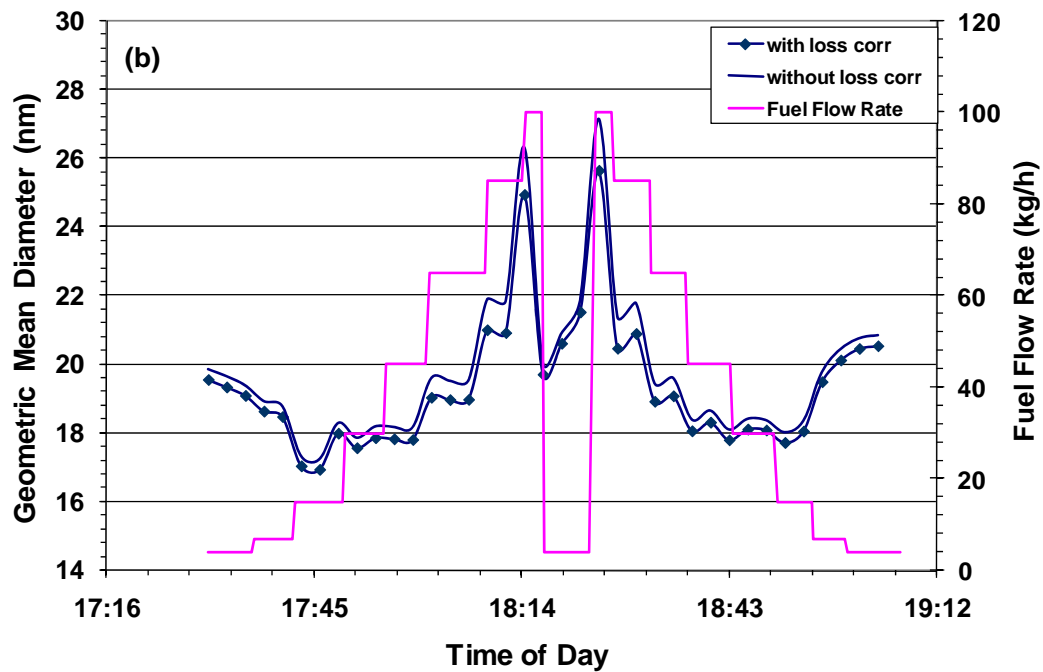
Figure 10-27. Two typical results of GMD as a function of fuel flow rate for (a) a CFM56-2C1 engine during APEX-1, Test EPA-2; and (b) for a CFM56-3B1 engine during APEX-3, Test T1.
