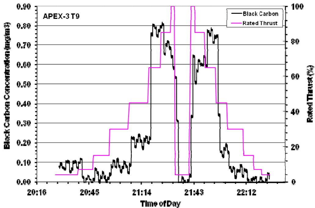
Figure 11-8. Time-series black carbon concentration data for the APEX-3 T8 and T9 for the RB211-535E4-B engine.
