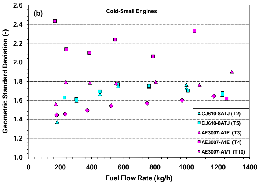
Figure 10-31. The (a) GMD and (b) GSD of the PM emissions measured for the small engines during APEX-3 as a function of fuel flow. Engines operated during the cold portion of the test cycle.
