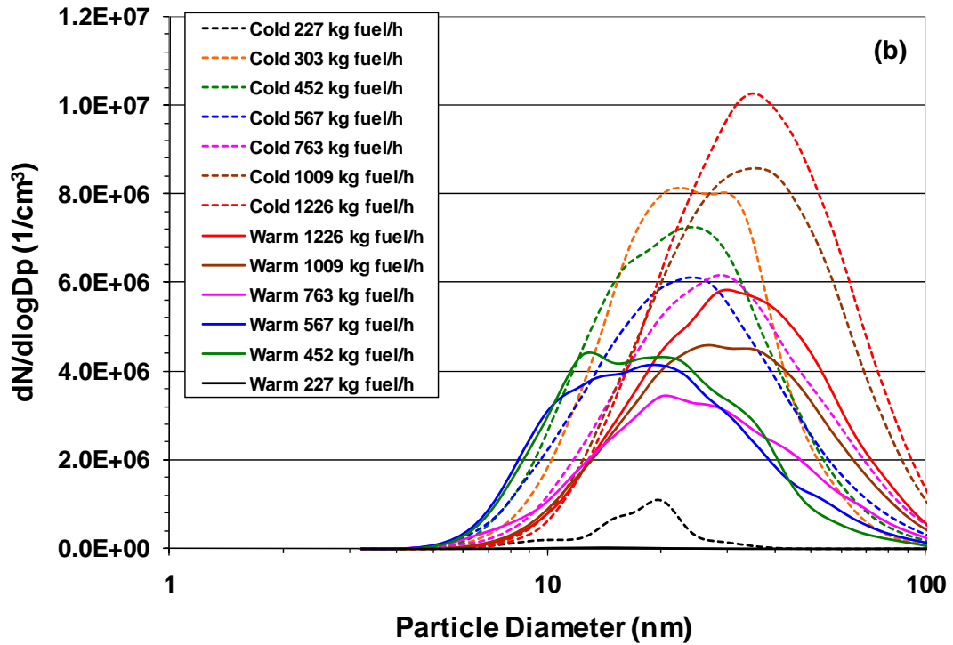
Figure 10-18. Average PSD for a CJ610-8ATJ turbojet engine measured by the Nano-SMPS during APEX-3, Test T5, (a) with line loss correction; and (b) without line loss correction.
