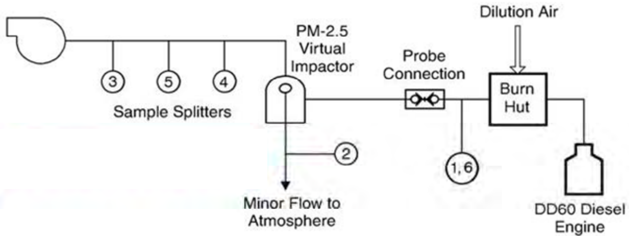
Figure 4-3. Sampling locations for particle line loss experiments.
