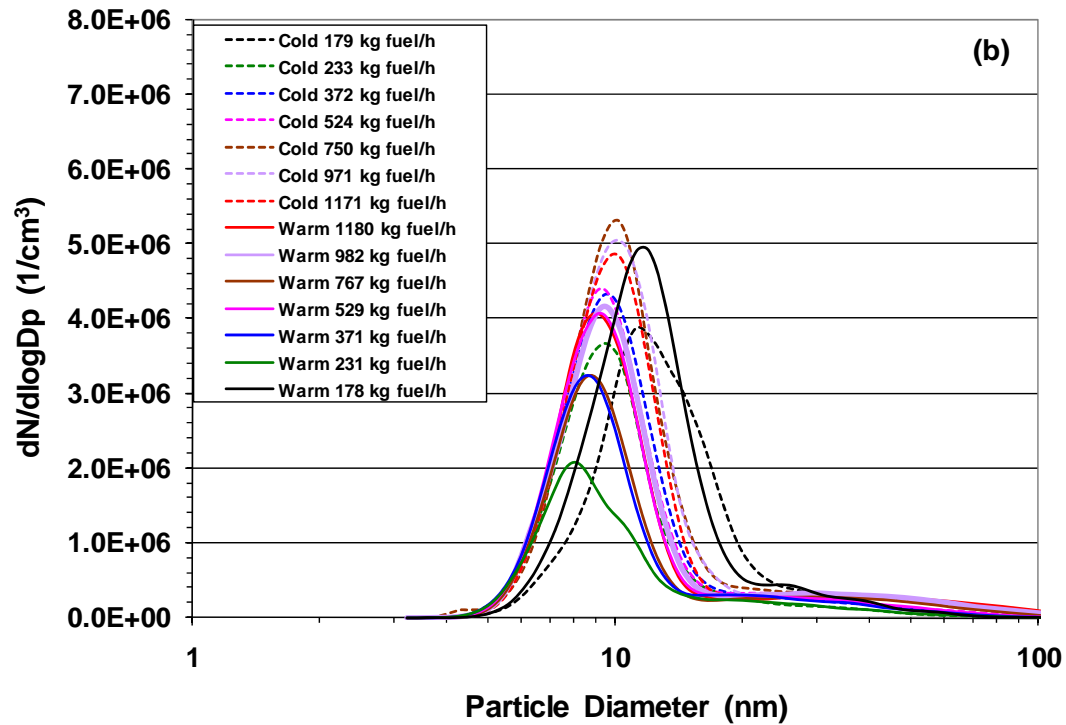
Figure 10-23. Average PSD for an AE3007-A1/1 engine measured by the Nano-SMPS during APEX-3, Test T10, (a) with line loss correction; and (b) without line loss correction.
