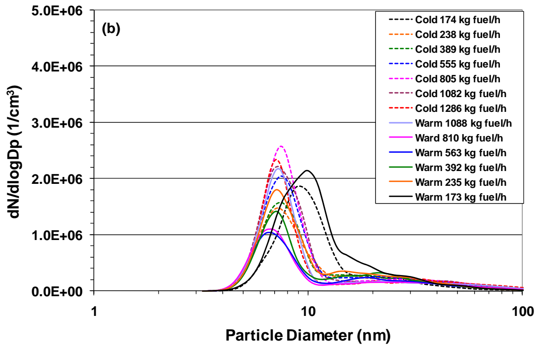
Figure 10-16. Average PSD for an AE3007-A1E engine measured by the Nano-SMPS during APEX-3, Test T3, (a) with line loss correction; and (b) without line loss correction.
