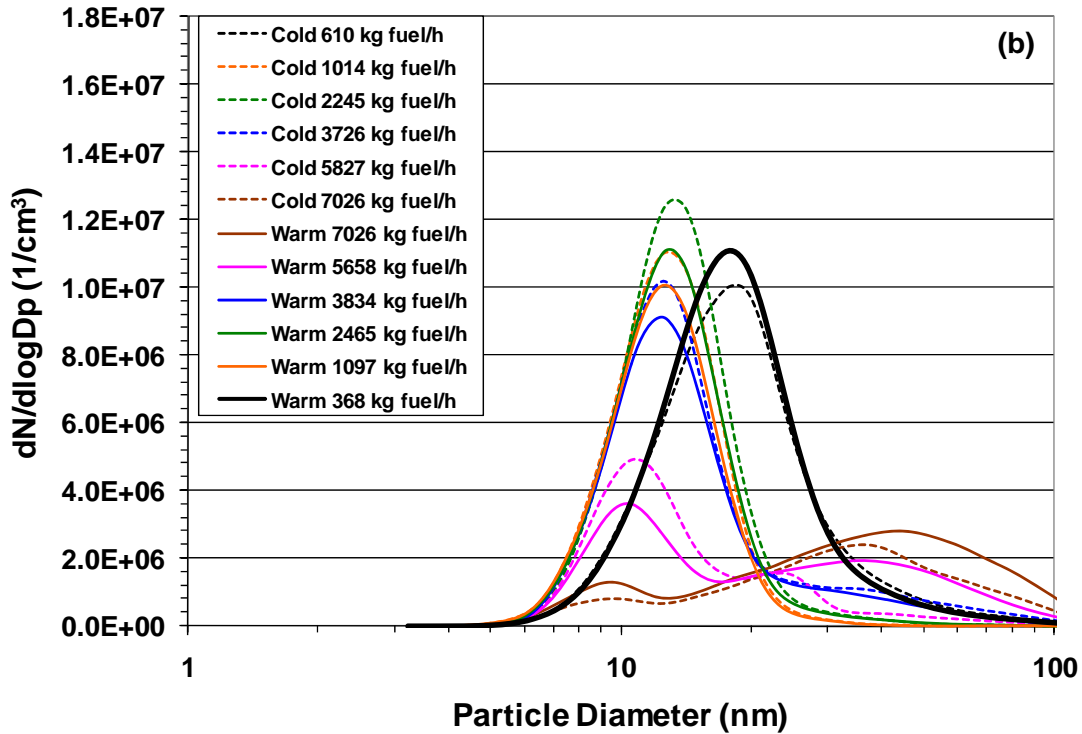
Figure 10-19. Average PSD for a PW4158 engine measured by the Nano-SMPS during APEX-3, Test T6, (a) with line loss correction; and (b) without line loss correction.
