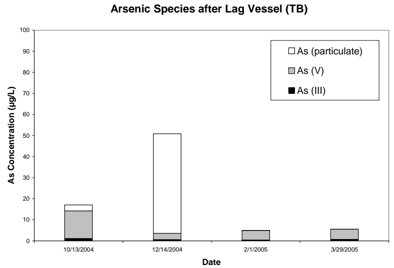
Figure 4-8. Concentration of Arsenic Species at the IN, AP, TA, and TB Sampling Locations
