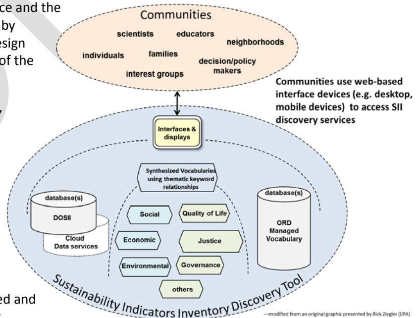
Figure 4-1: Conceptual Architectural Overview for Sustainability Indicators Inventory Discovery Tool
