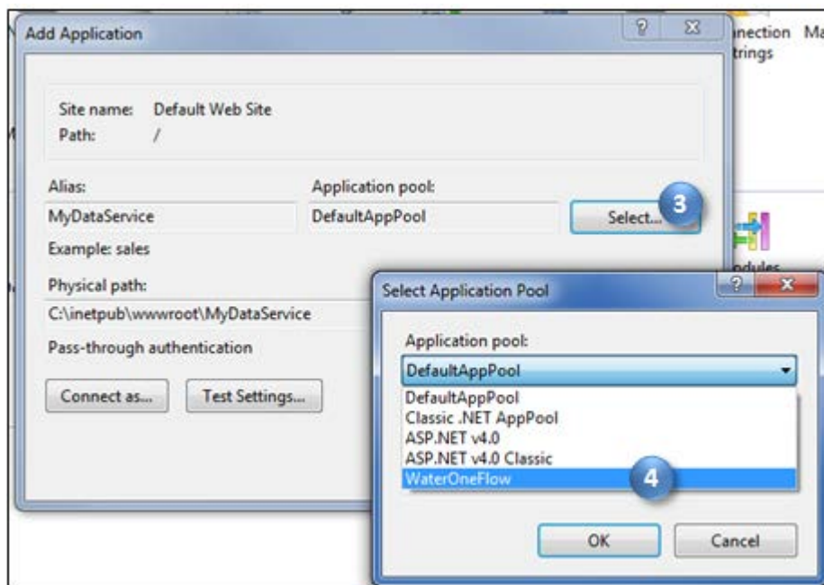
Figure 0-7 Selecting the WaterOneFlow application pool
