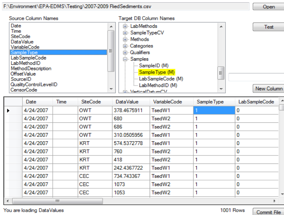
Figure 3-11. Modified Data Loader
