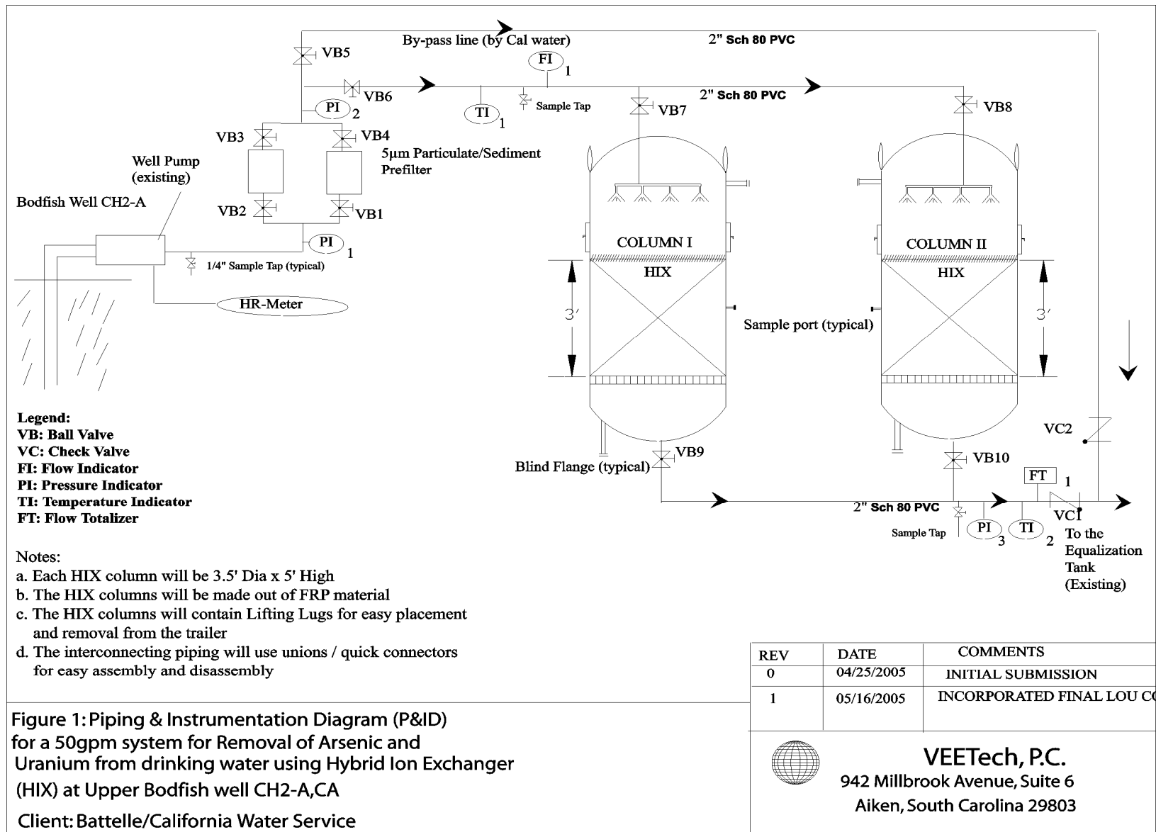
Figure 4-3. P&ID of HIX Treatment System (Provided by VEETech)
