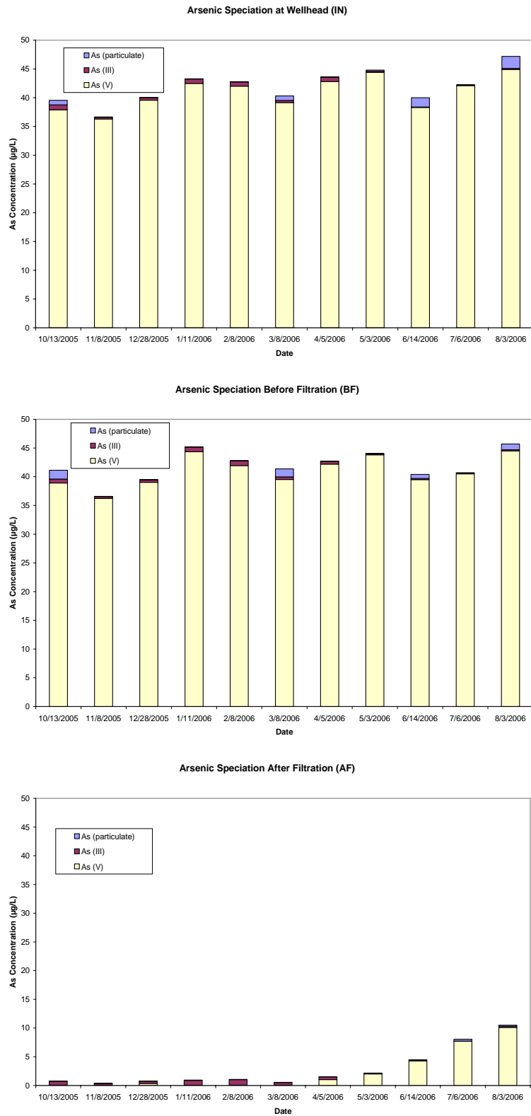
Figure 4-8. Concentrations of Various Arsenic Species at IN, BF, and AF Sampling Locations
