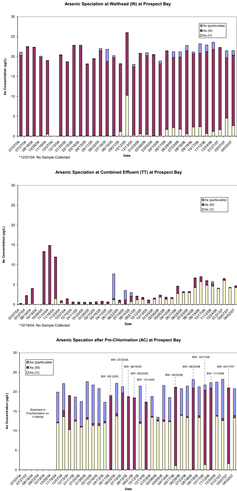
Figure 4-13. Concentration of Arsenic Species at IN, AC, and TT Sample Locations
