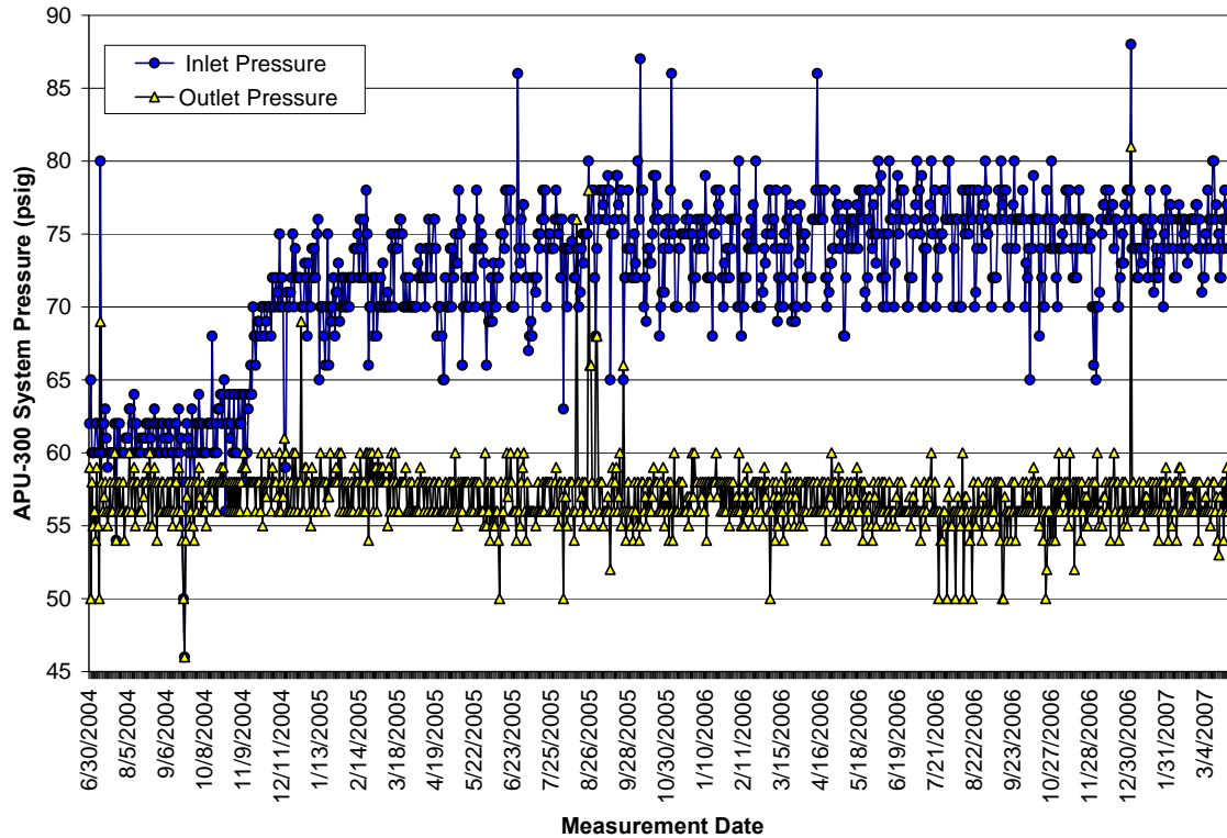
Figure 4-10. APU-300 Treatment System Inlet and Outlet Pressure
