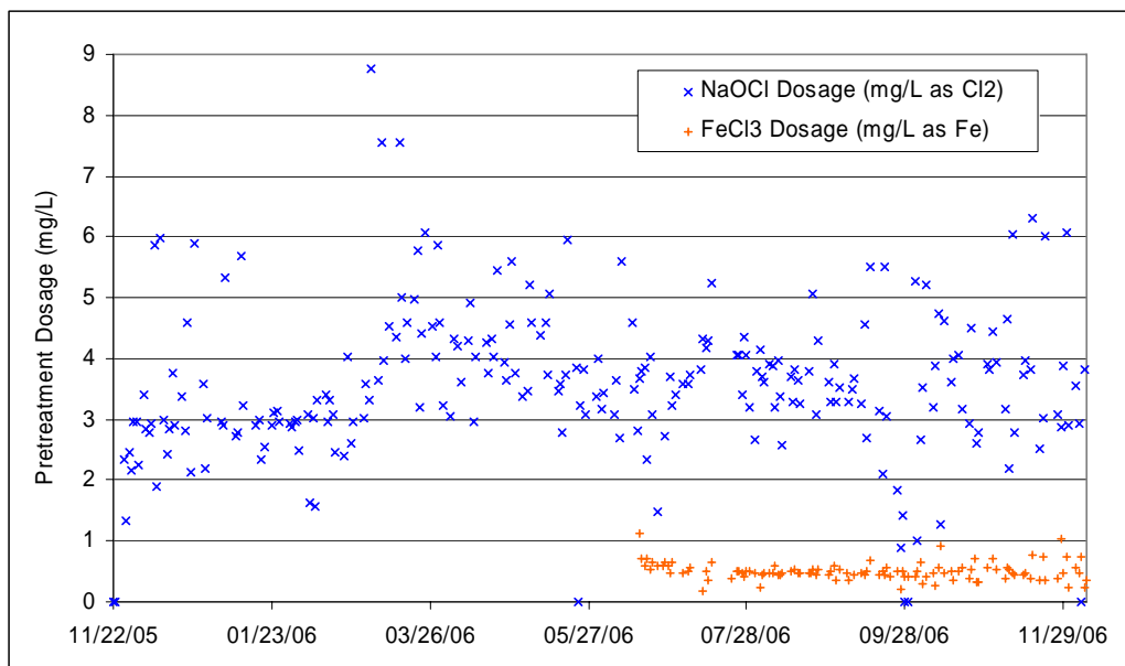
Figure 4-8. Chlorine and Ferric Chloride Dosages of Over Time
