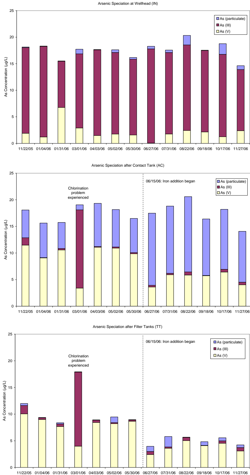
Figure 4-10. Arsenic Speciation Results
