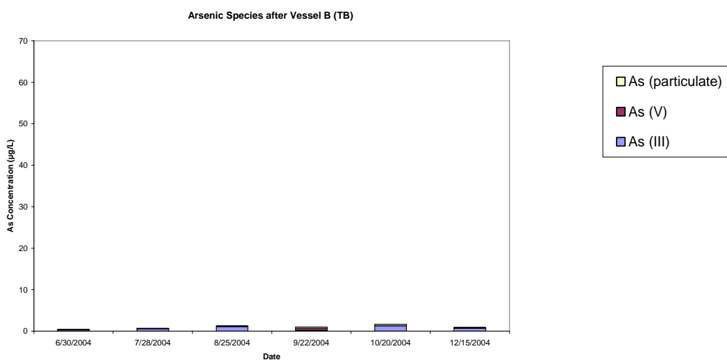
Figure 4-7. Concentration of Arsenic Species at the Inlet, after Vessel A, and after Vessel B
