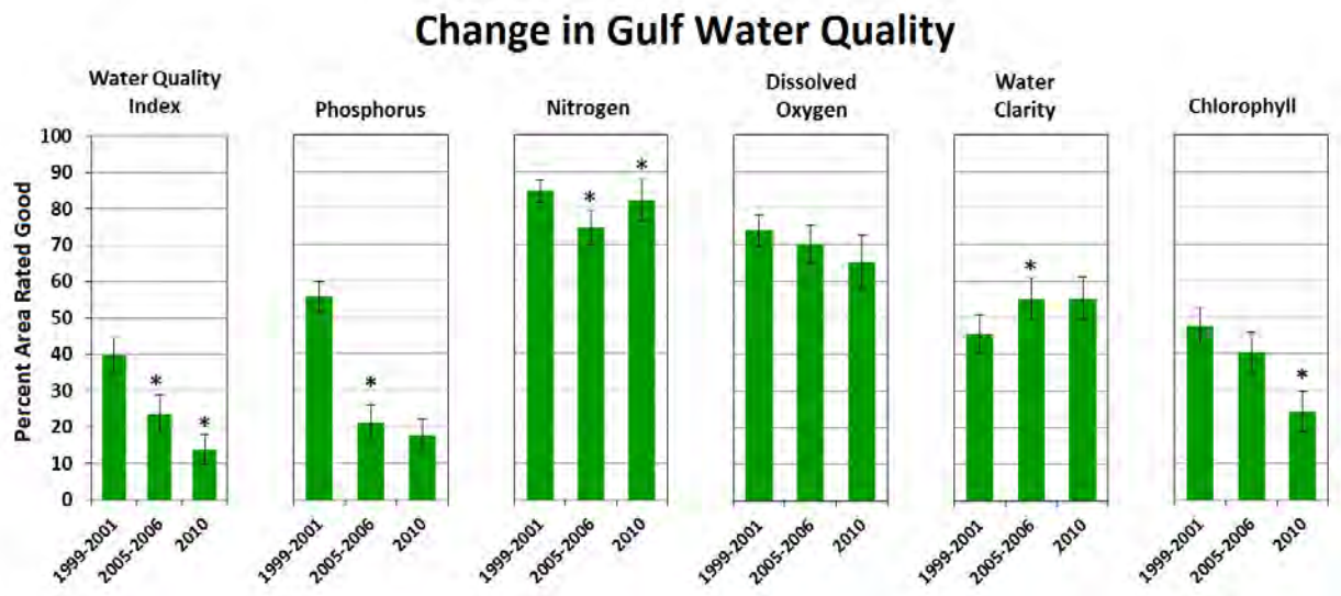
Figure 4-12. Comparison of the percent area rated good for Gulf Coast water quality indicators over three periods. Note: Asterisks indicate statistically significant change between periods.
