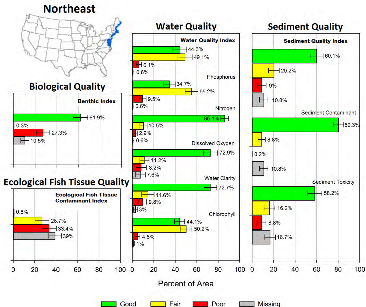
Figure 4-5. NCCA findings for the Northeast Coast. Bars show the percentage of coastal area within a condition class for a given indicator. Error bars represent 95% confidence levels. Note: The sum of percent of area for each indicator may not add up to 100% due to rounding.
