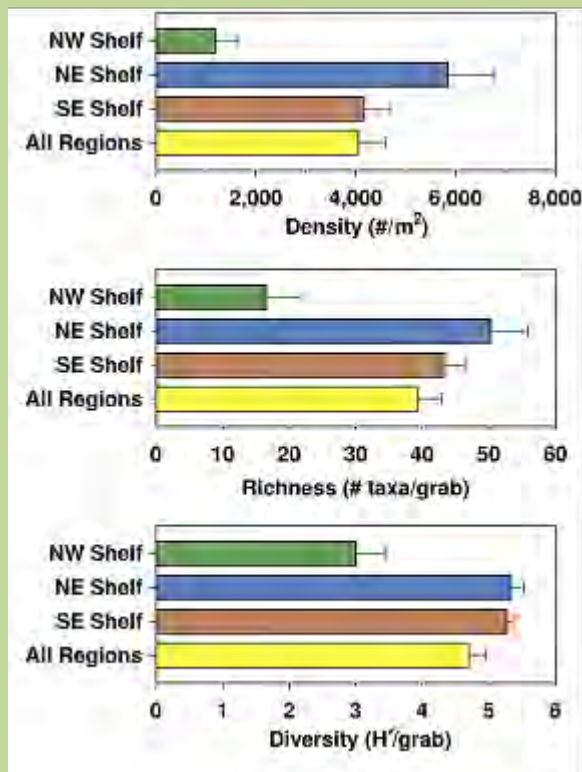
Figure 3-14. Species density, richness, and diversity data from the Gulf.
