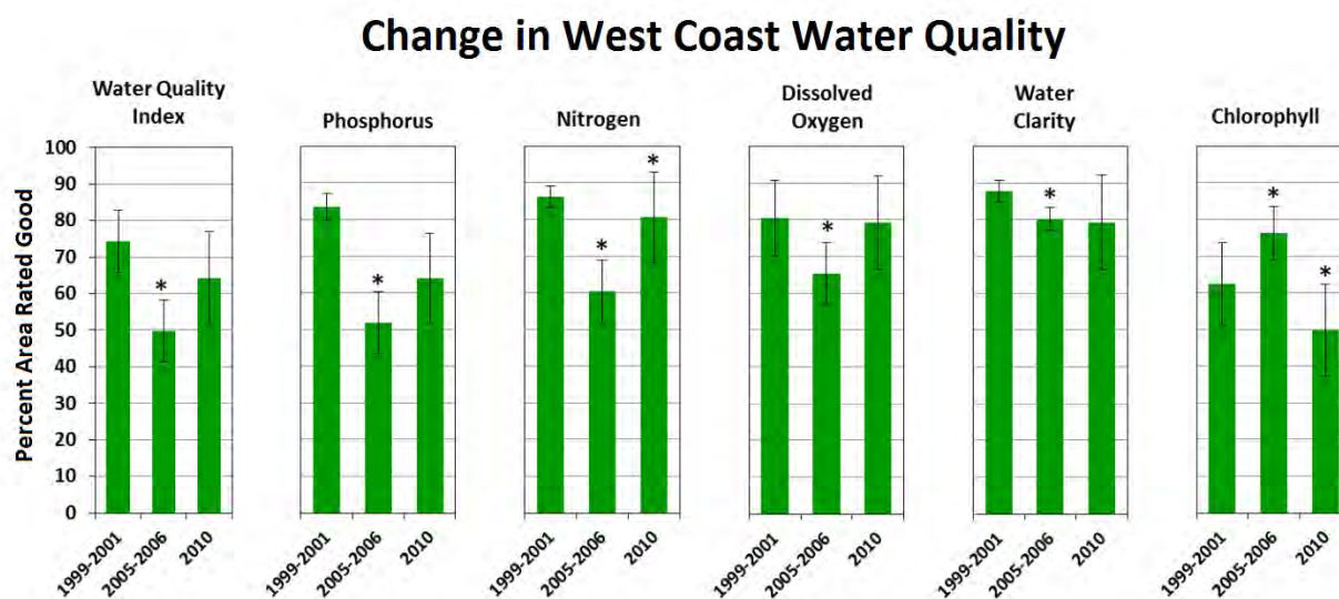
Figure 4-17. Comparison of the percent area rated good for West Coast water quality indicators over three periods. Note: Asterisks indicate statistically significant change between periods.
