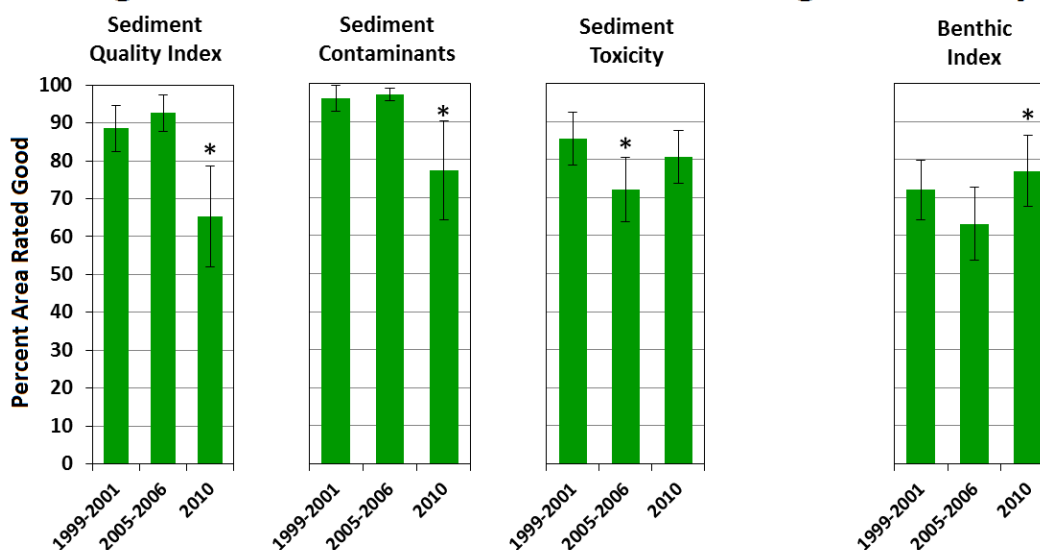
Figure 4-10. Comparison of the percent area rated good for sediment and biological quality over three periods in the Southeast. Note: Asterisks indicate statistically significant change between periods.
