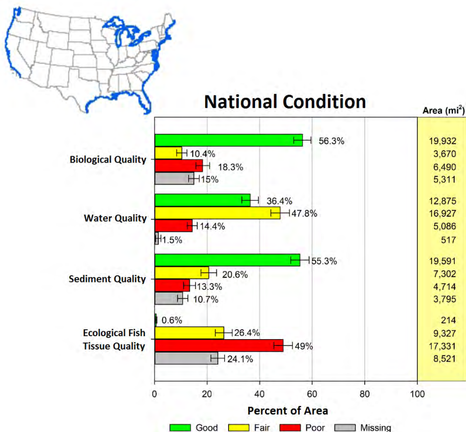
Figure ES-1. Condition of the nation's coastal waters for each of the four NCCA indices (U.S. EPA/NCCA 2010). Note: Percentages may not add up to 100% due to rounding.
