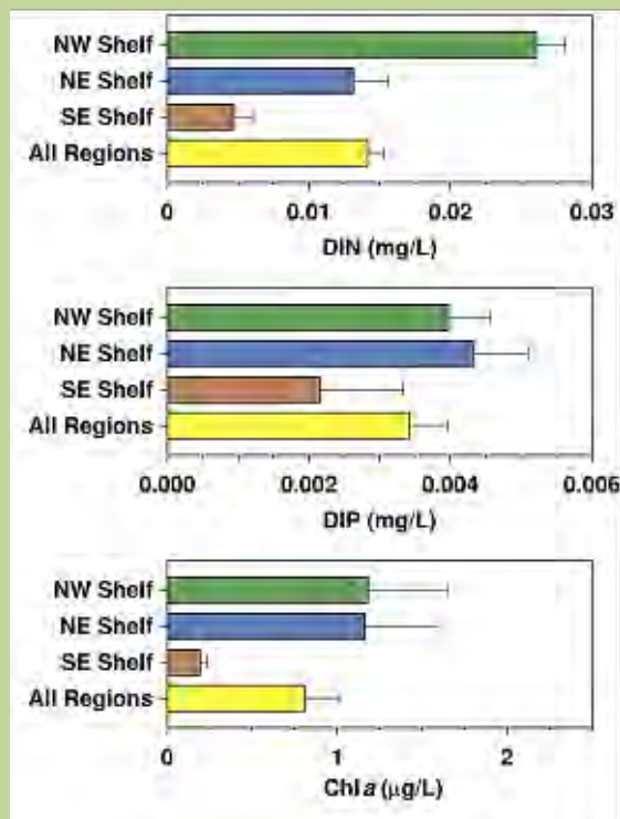
Figure 3-11. Mean concentrations of nitrogen, phosphorus, and chlorophyll a in Gulf surface waters (NOAA).
