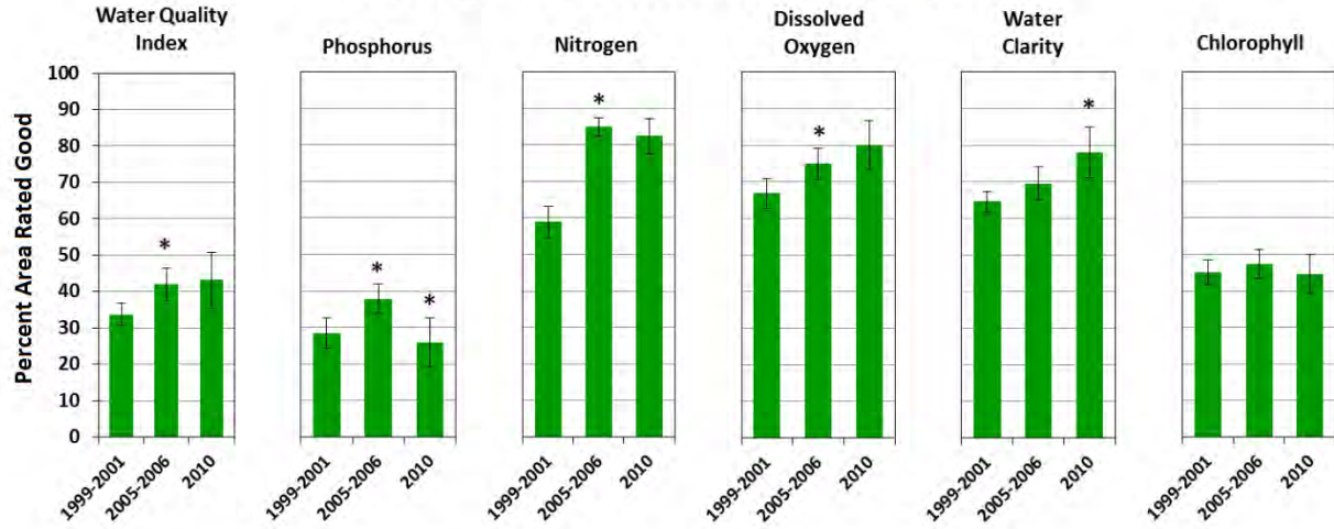
Figure 4-6. Comparison of the percent area rated good for water quality indicators over three periods in the Northeast Coast. Note: Asterisks indicate statistically significant change between periods.
