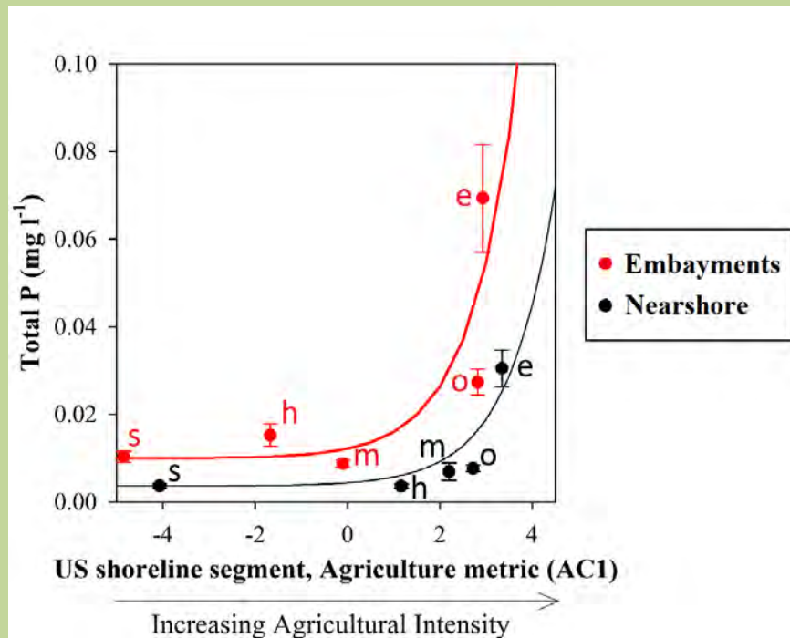
Figure 2-3. Total phosphorus as a function of increasing agricultural intensity shows that embayments have higher levels of TP than nearshore areas. Mean and 95% confidence intervals are shown for NCCA 2010 results by lake (identified by first letter of lake name) for nearshore (in black) and embayment populations (in red). From Kelly et al., 2015.
