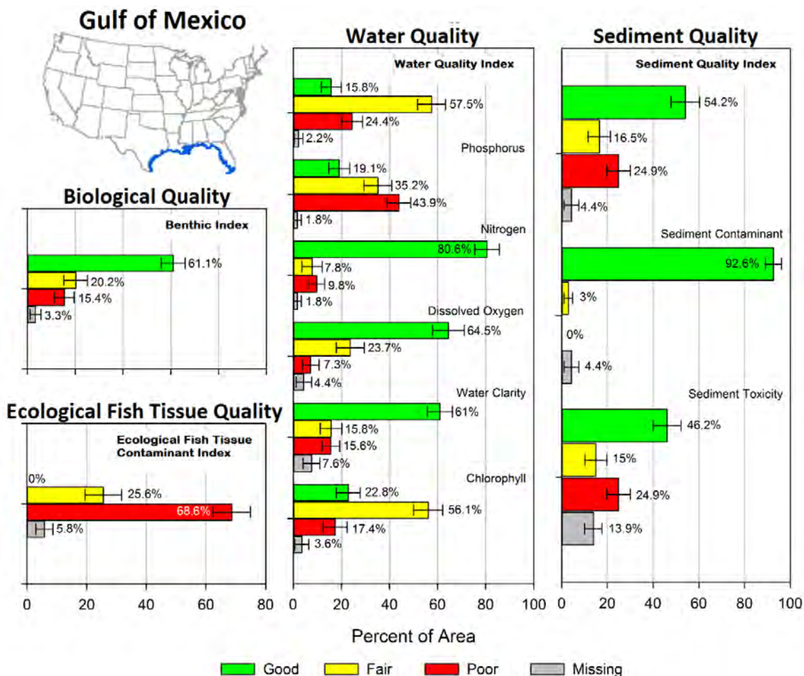
Figure 4-11. NCCA findings for the Gulf Coast. Bars show the percentage of coastal area within a condition class for a given indicator. Error bars represent 95% confidence levels. Note: The sum of percent of area for each indicator may not add up to 100% due to rounding.
