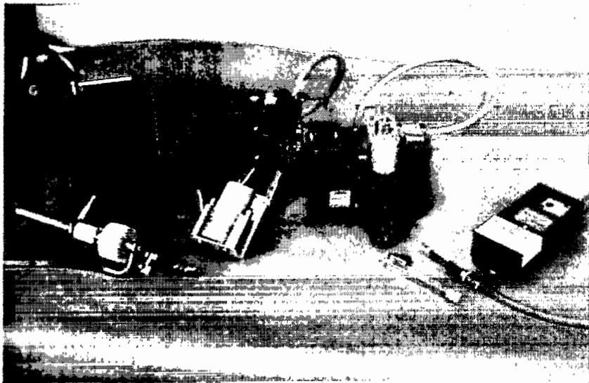
A vacuum pump with attachments for sampling with a filter, a sorbent tube, and an impinger. Use in a non-industrial setting may require a larger volume of air. Consult with qualified industrial hygienists and chemists if adapting sampling methods.
