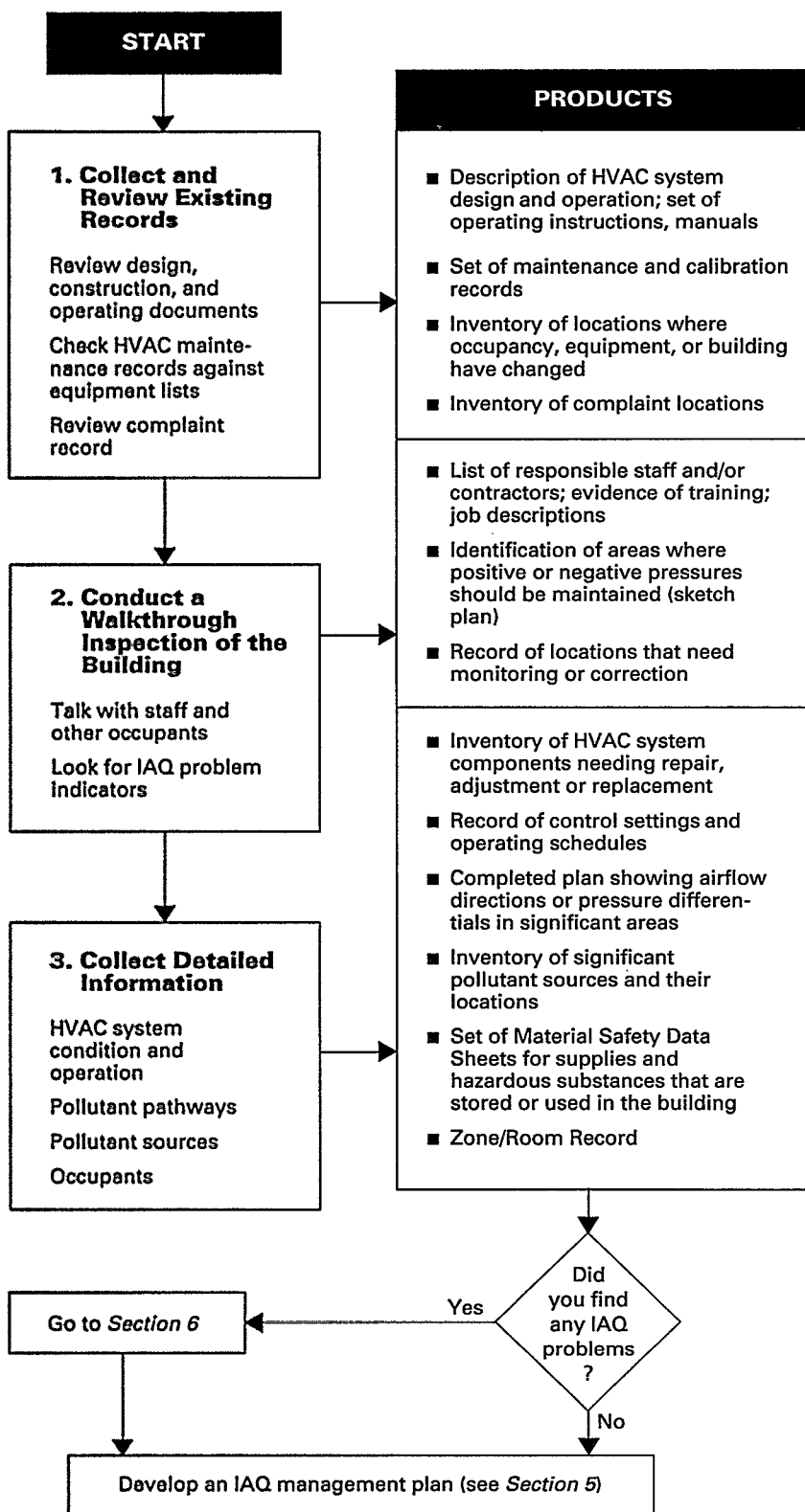
FIGURE 4-1: Developing an IAQ Profile
