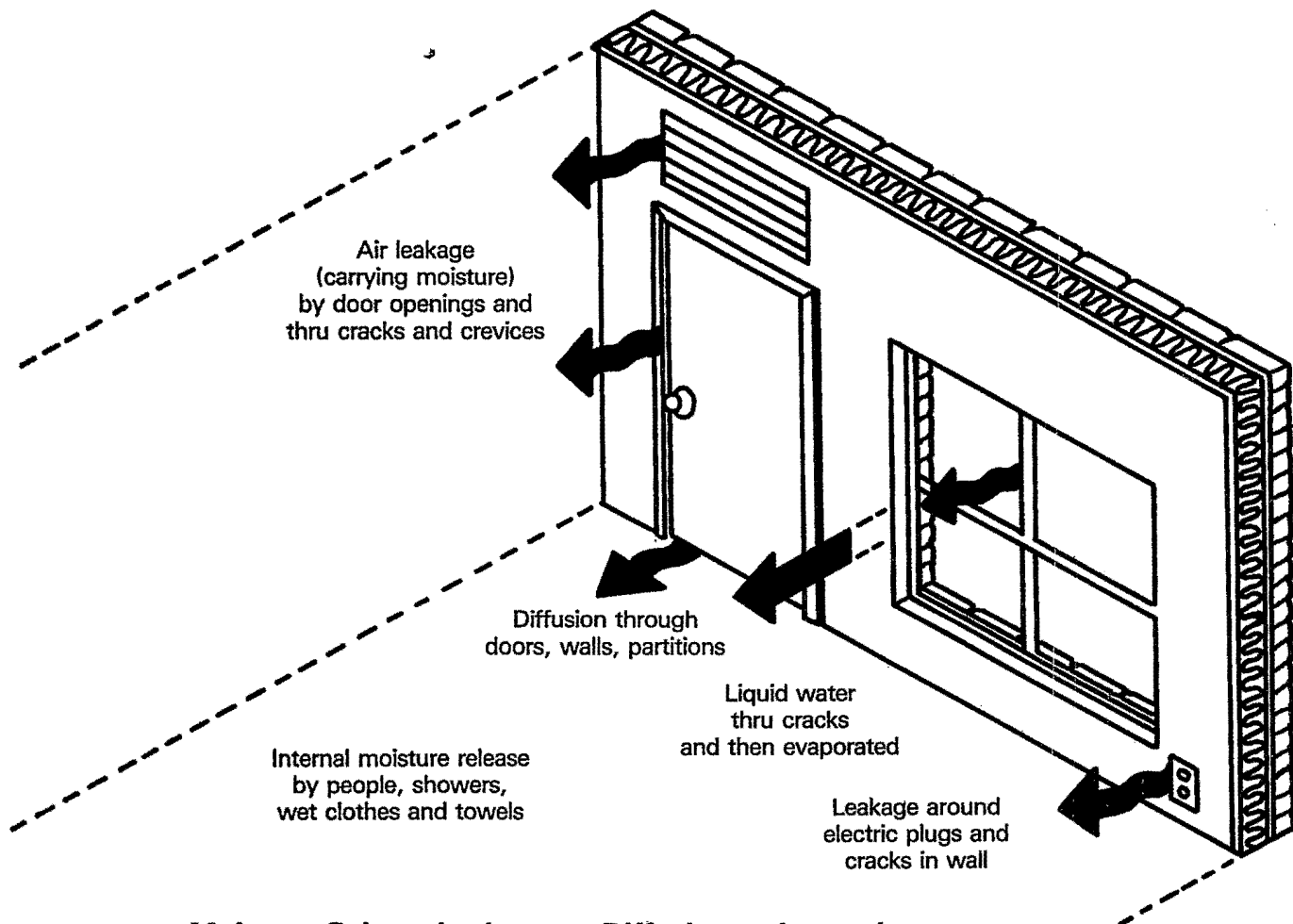
FIGURE C-1: Moisture Gain in a Building
