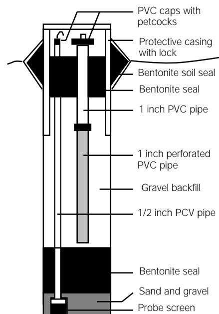
Figure 9-16 Example of a Gas Monitoring Probe
