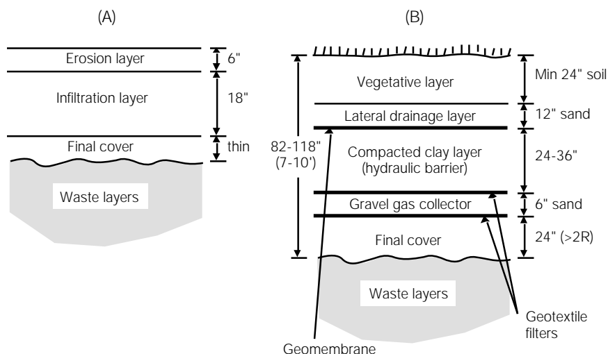
Figure 9-20 Examples of Final Covers
