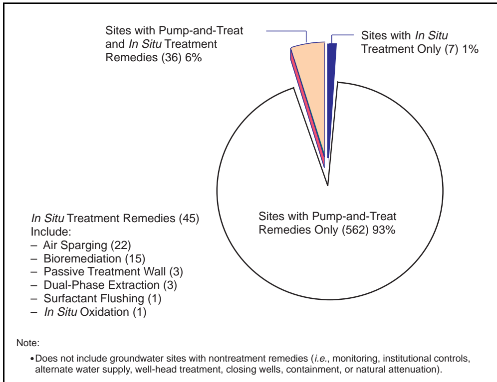
Exhibit 1-7: Groundwater Treatment Remedies at NPL Sites Through FY 1995
