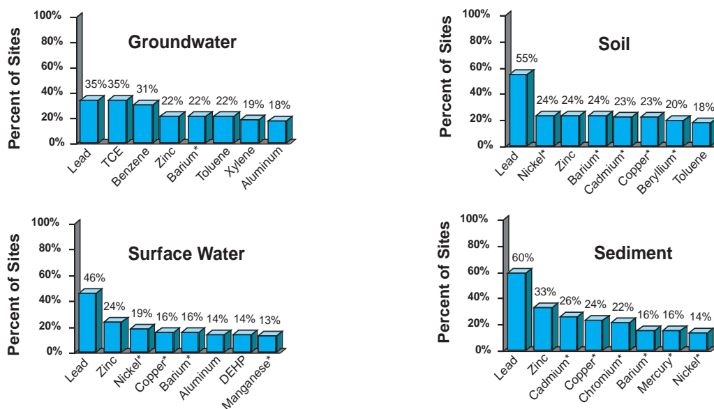
Exhibit 6-10: Frequency of the Most Common Contaminants by Matrix at DOD Sites Needing Cleanup
