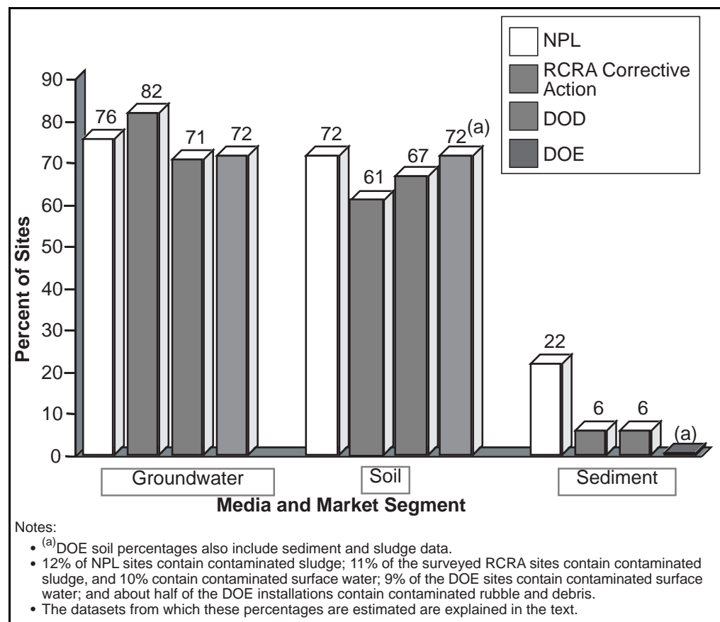
Exhibit 1-3: Media to be Remediated
