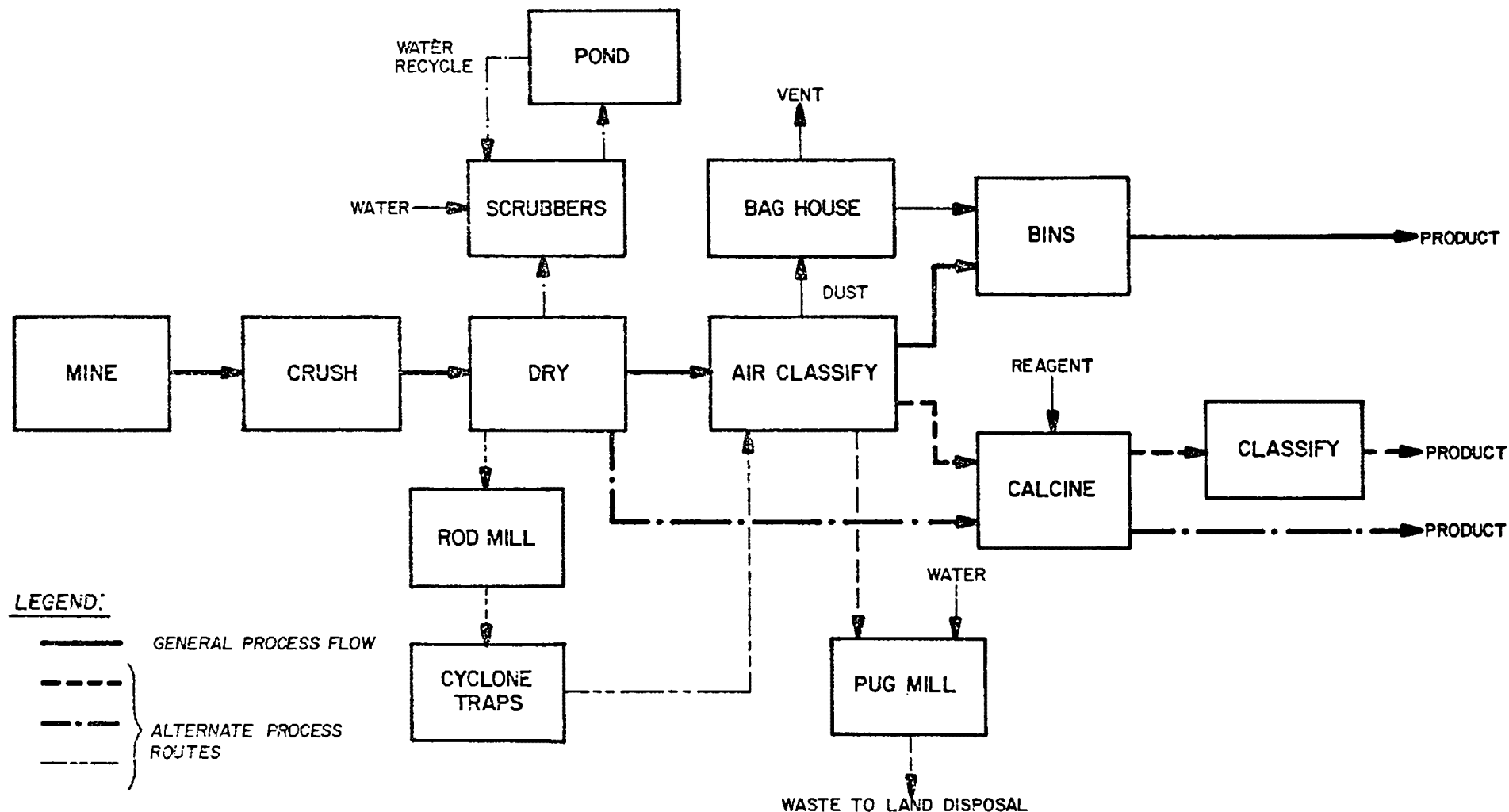
FIGURE 28. DIATOMITE MINING AND PROCESSING
