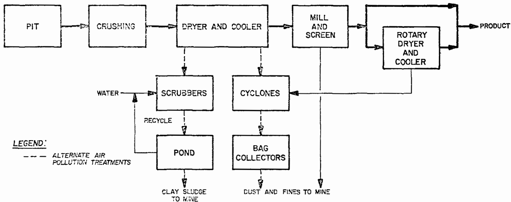
FIGURE 10. FULLER'S EARTH MINING AND PROCESSING (MONTMORILLONITE)
