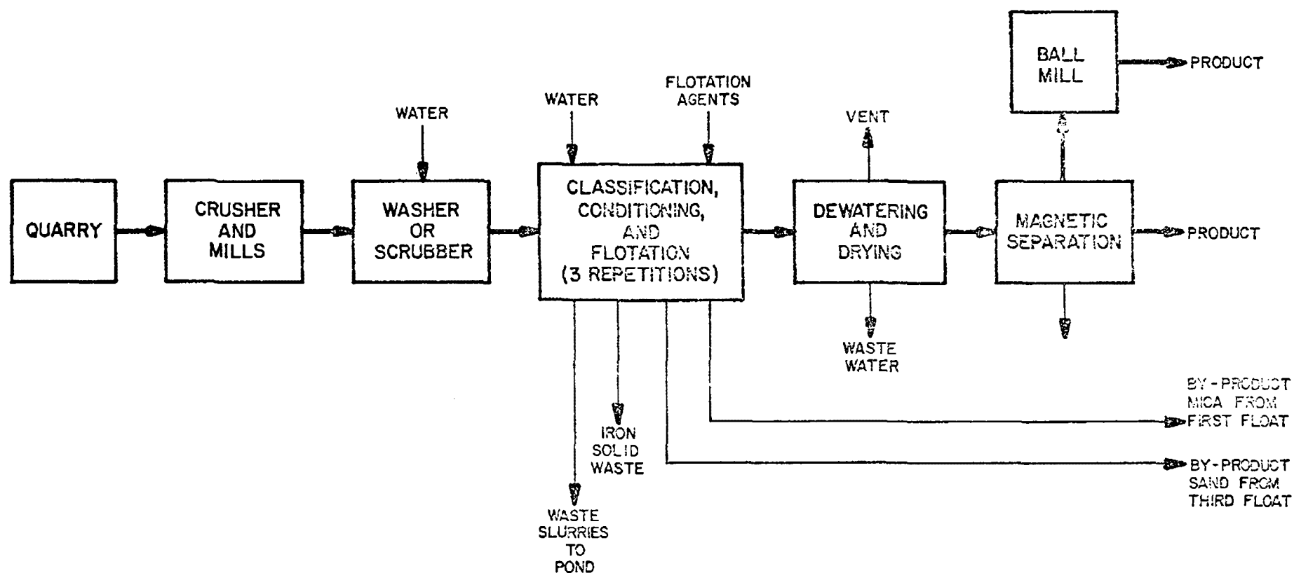
FIGURE 14. FELDSPAR MINING AND PROCESSING (WET)
