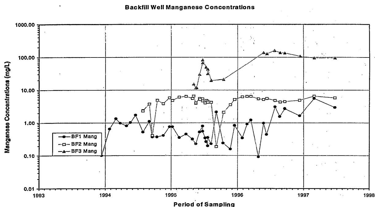
Figure 2.2.3b: Water Quality Before and After Mining at the Case Study 2 Site
