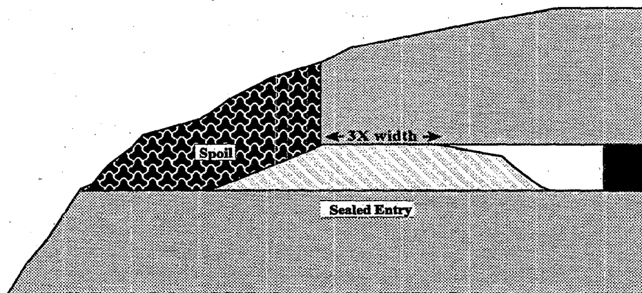
Schematic Drawing of a Sealed Mine Entry
