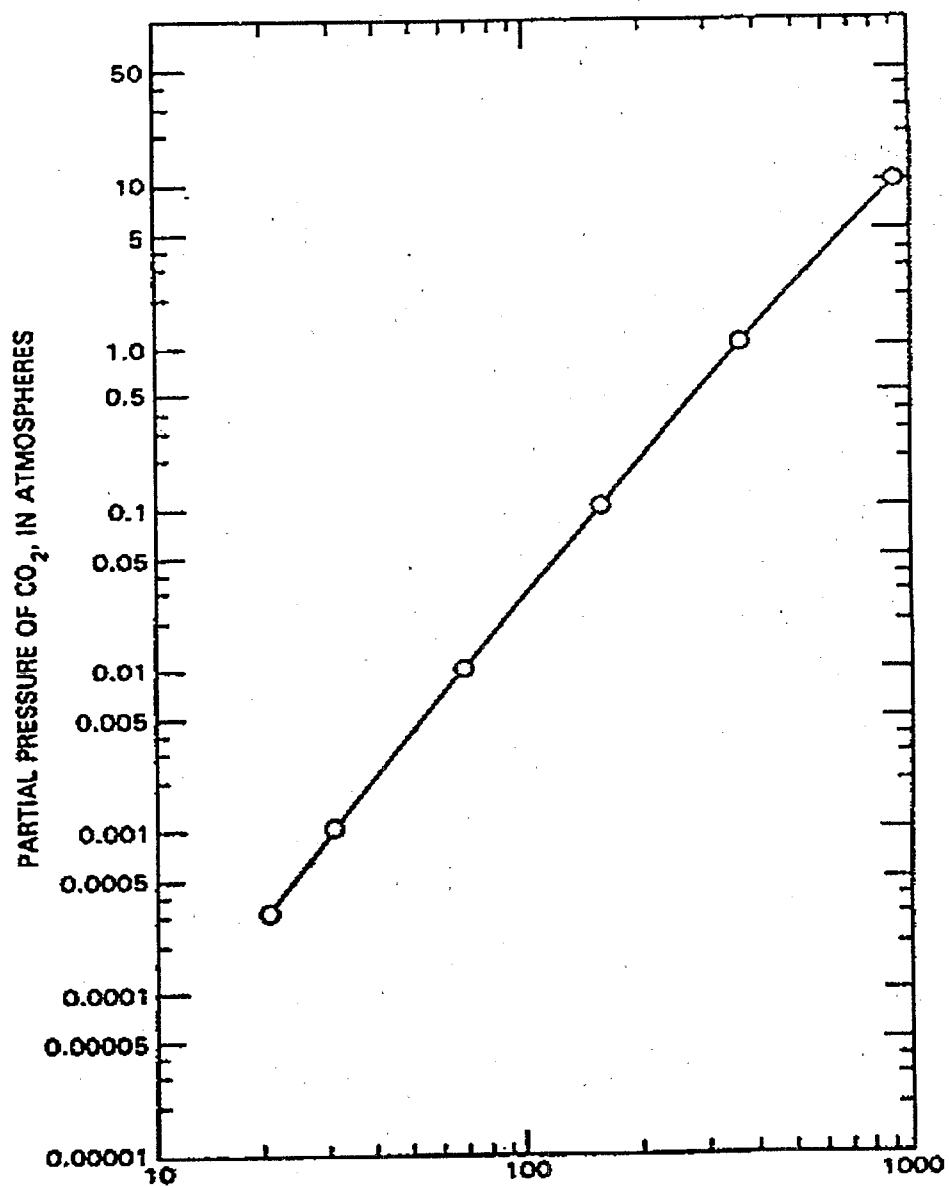
Figure 2.2a: Solubility of Calcium Carbonate (Calcite) in Water at 25°C as a Function of Partial Pressure of CO 2 (Hem, 1985)
