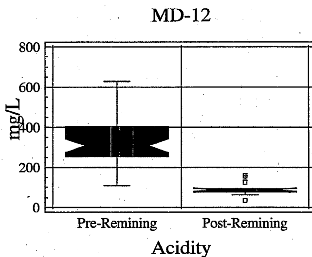
Figure 1.1.3b: Acidity Load at Discharge Point MD-12 Before and After Remining
