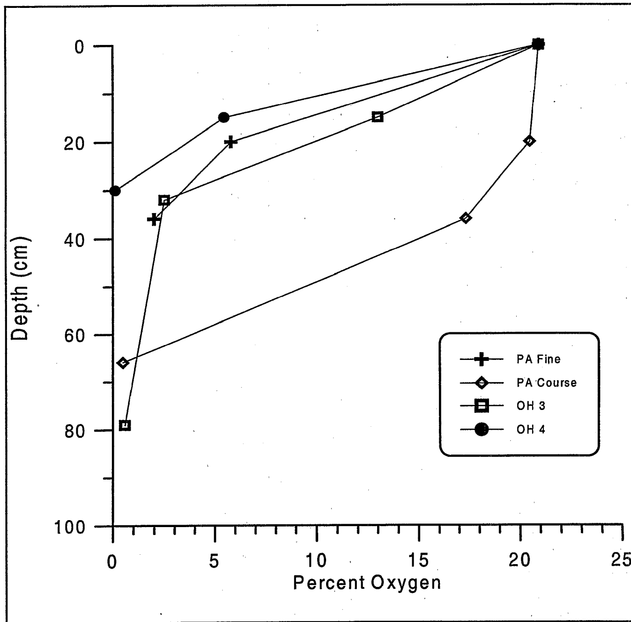
Figure 2.5.3c: Oxygen Concentration with Depth in Coal Refuse in Pennsylvania and Ohio.
