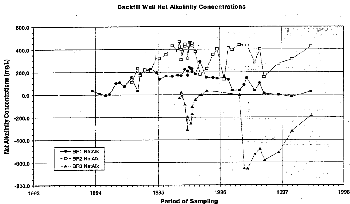
Figure 2.2.3c: Water Quality at the Case Study 3 Site
