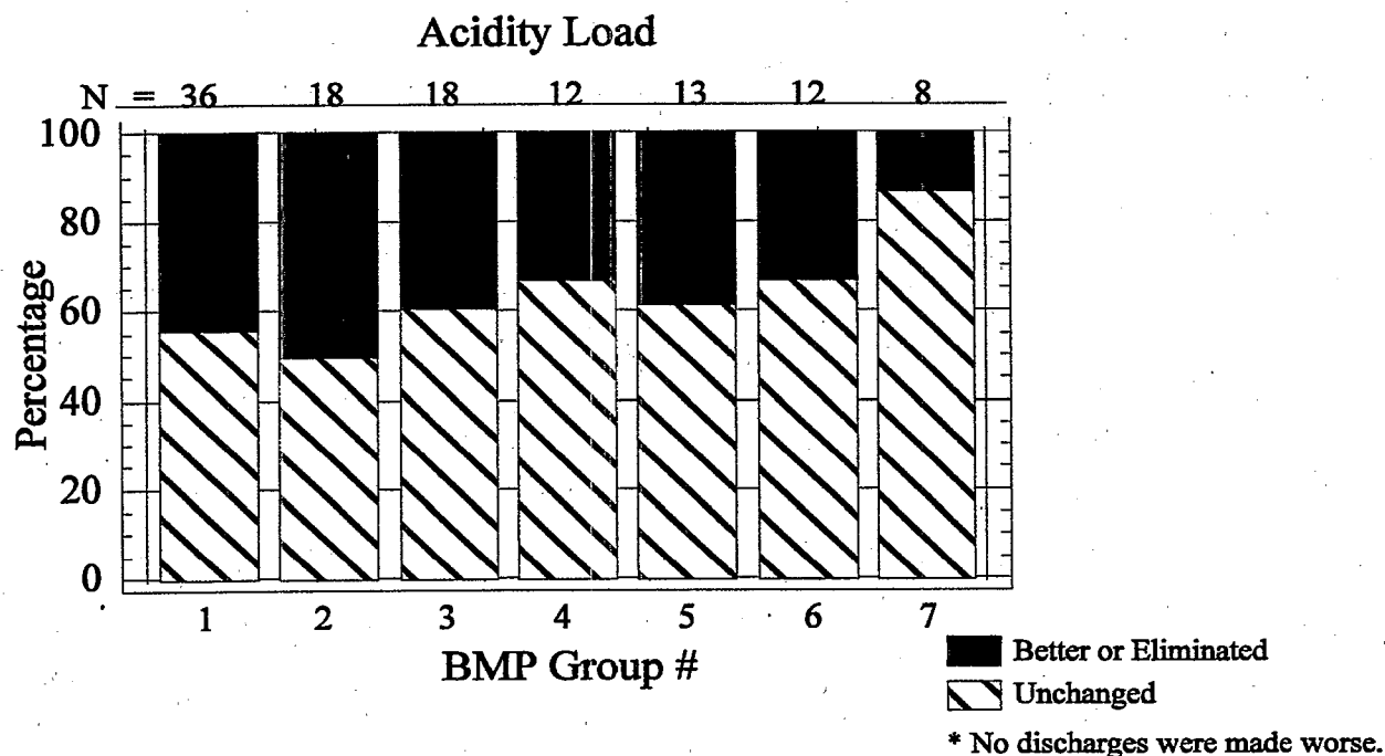
Figure 6.4a: Impacts of BMP Combinations on Acidity Loading
