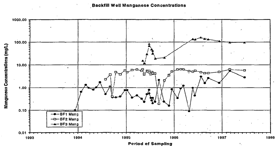
Figure 2.2.3c: Water Quality at the Case Study 3 Site (continued)
