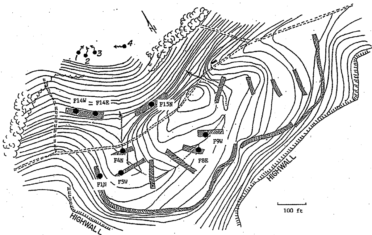
Figure 2.3.3a: Topography, Location of Recharge Trenches and Funnels, and Locations of Seeps (Case Study 1, Upshur County, WV) (Caruccio and Geidel, 1984).
