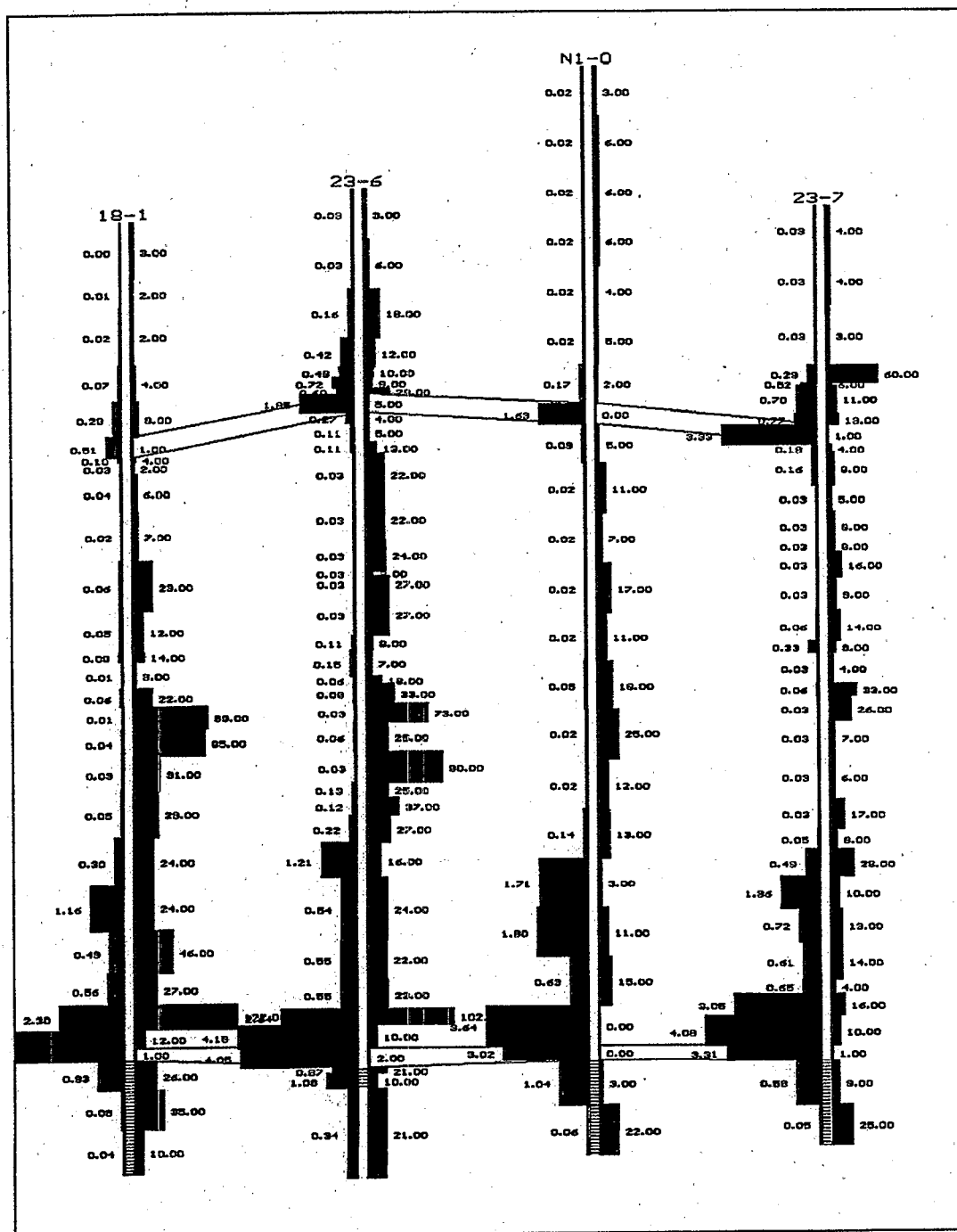
Figure 2.4.3a: Distribution of Sulfur and Neutralization Potential for Bedrock at the Special Handling Site in Clarion County, PA. (Drill logs are to scale. Most sample intervals for N1-0 are five feet.)
