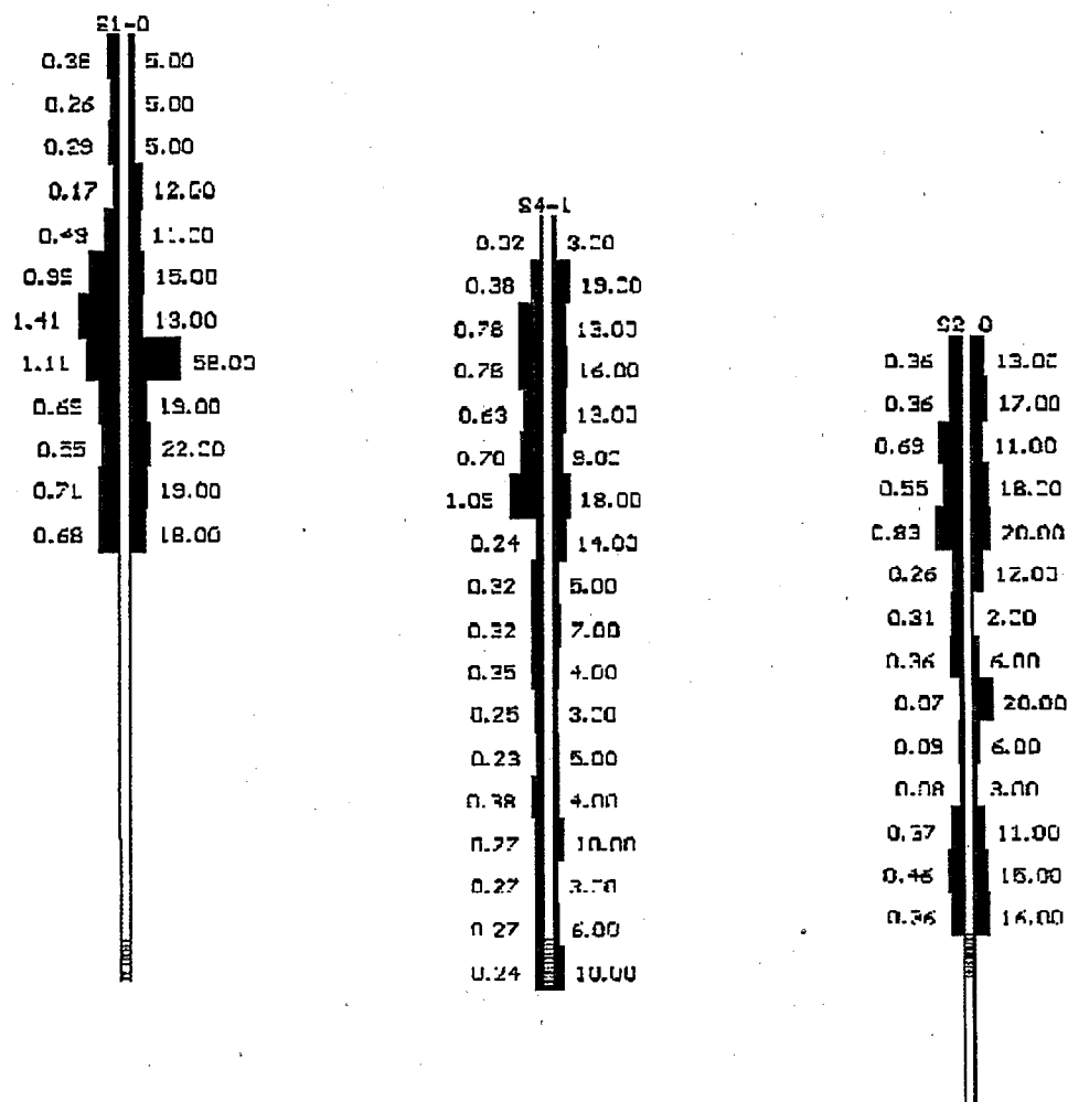
Figure 2.4.3c: Distribution of Sulfur and Neutralization Potential for Spoil in the Southern Hilltop Where a Dragline was Used (Sample intervals are five feet.)
