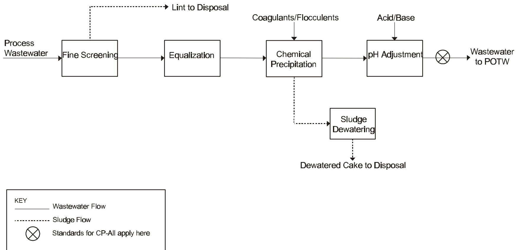
Figure 8-5. CP-All Option: Chemical Precipitation of Total Facility Process Wastewater
