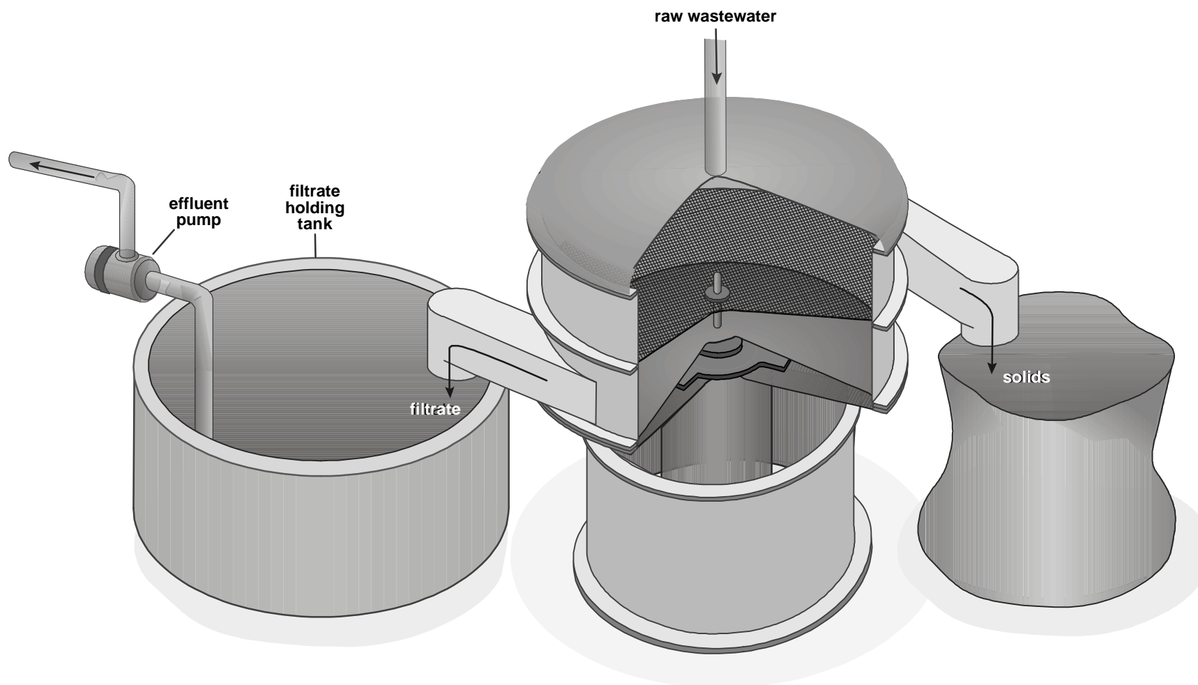
Figure 6-2. Shaker Screen
