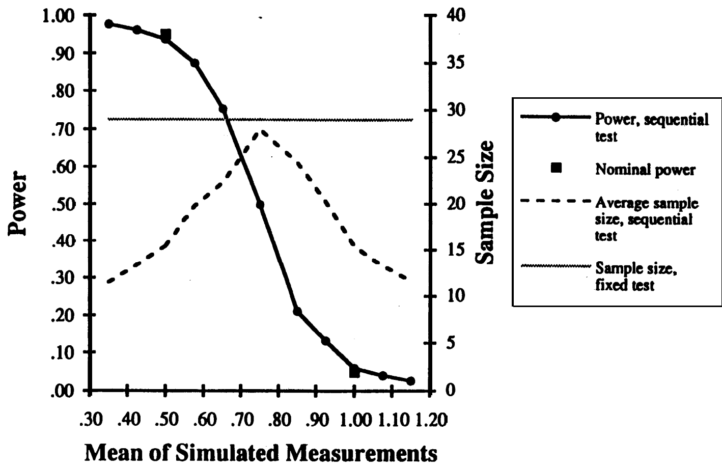
Figure 6 Power Curve and Average Sample Size for the Modified Sequential t-Test
