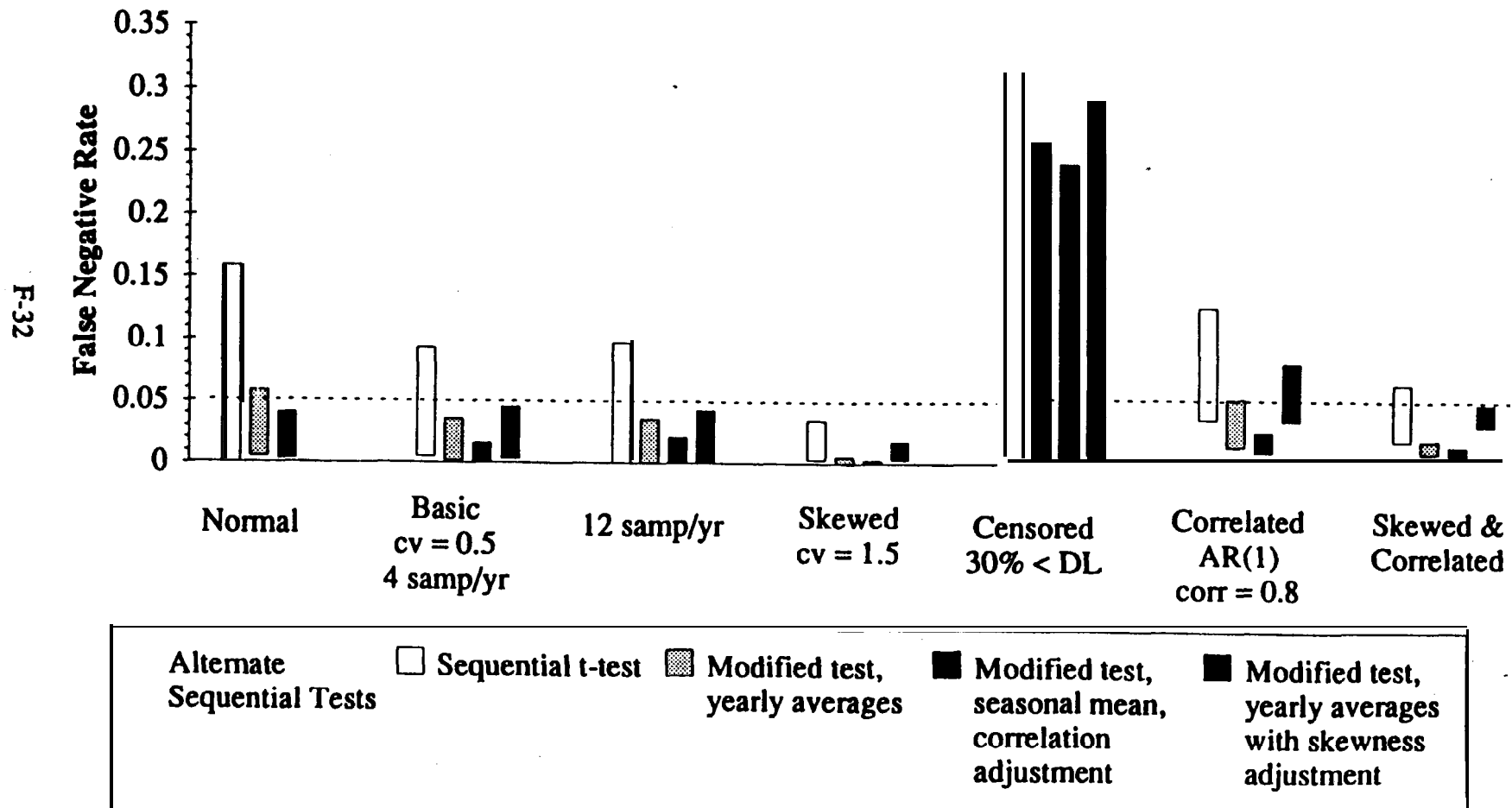
Figure 9 Range of False Negative Rates for Scale Factors from 1.6 to 4.8 for Four Sequential Tests, by Data Type
