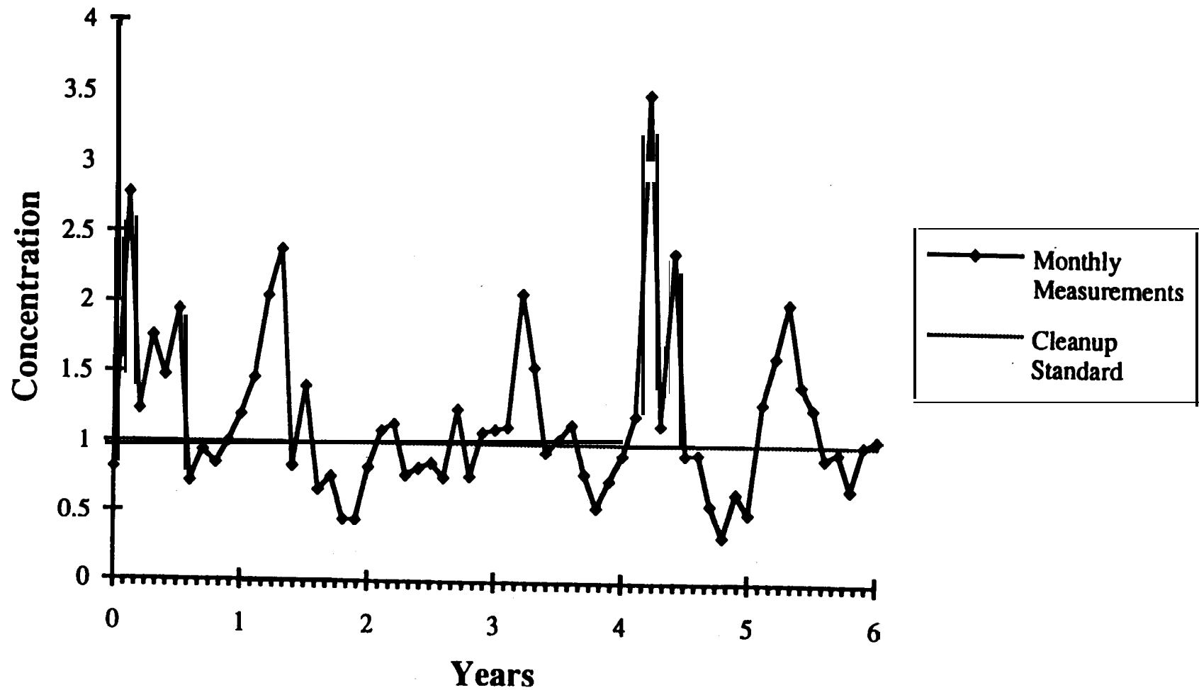
Figure 1 Example of Simulated Monthly Ground Water Data
