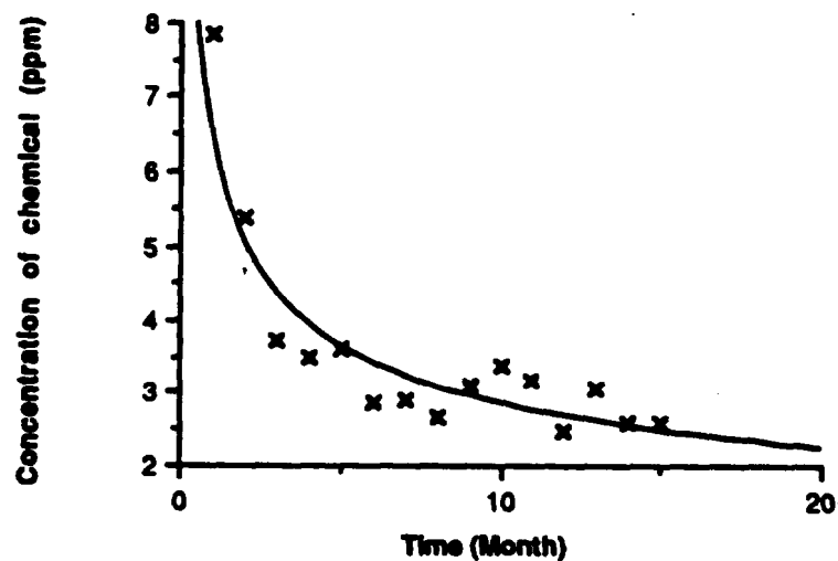
Figure 6.17 Examples of Nonlinear Relationships
