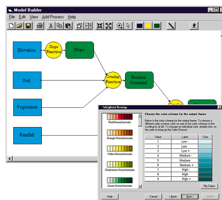
Figure 17 Screen capture of Spatial Analyst's ModelBuilder
