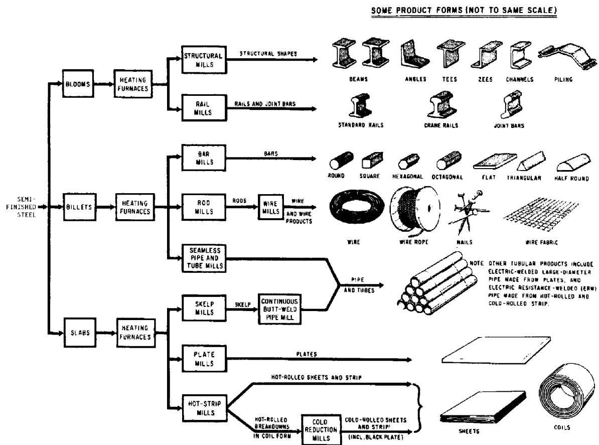
Figure 2-6. Steel Finishing Processes by Mill Type
