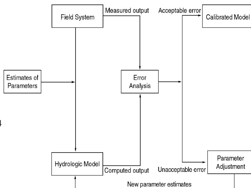
Figure 4. Calibration procedure of hydrological models.
