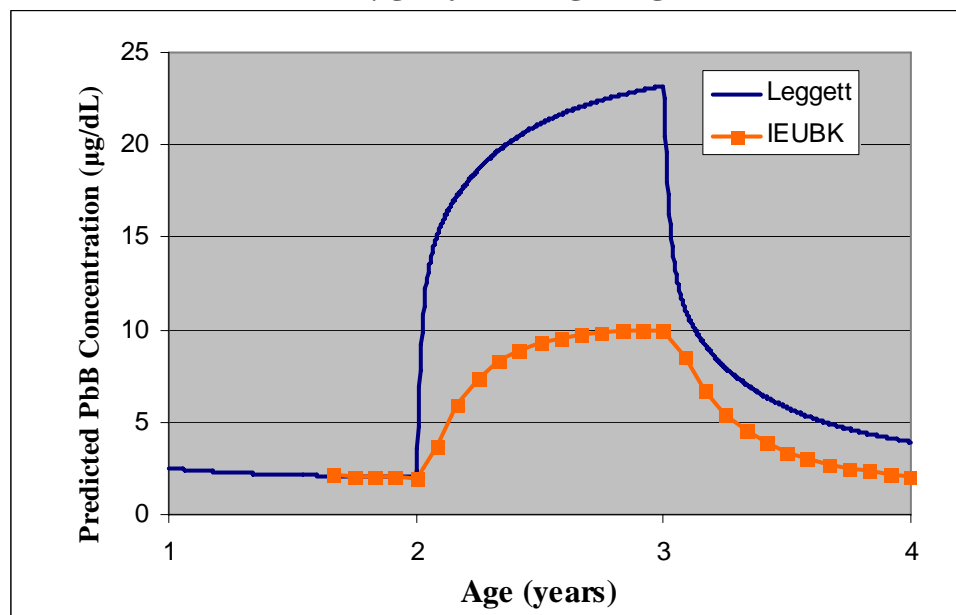
Exhibit J-2. FORTRAN Leggett Model Predicted PbB Response to a 1 Year Increase in Pb Intake of 100 \mu\text{g/day} Starting at Age 2
