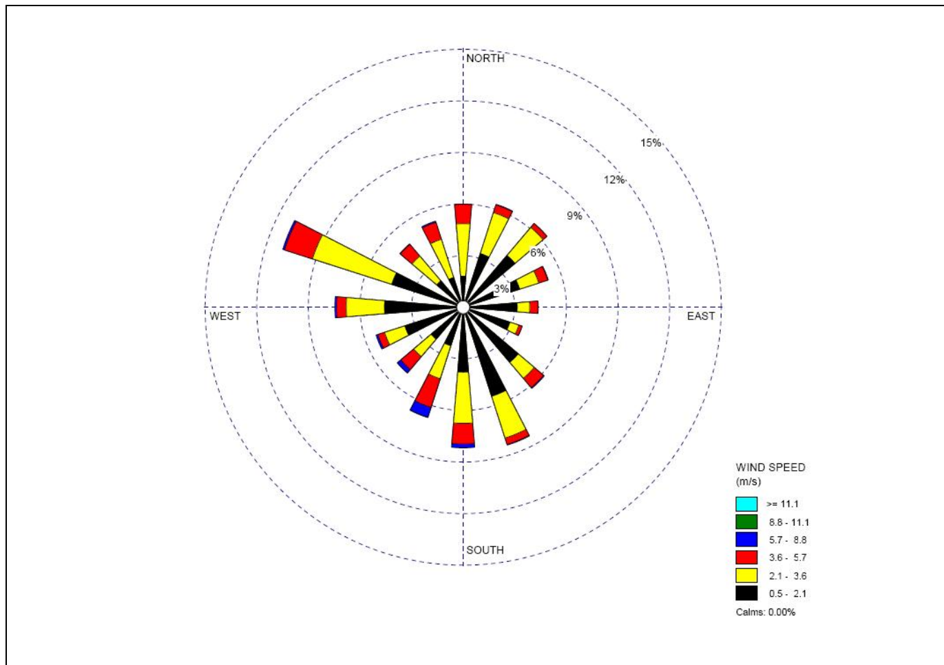
Exhibit D-4. Wind Rose of Meteorological Data used for Primary Pb Smelter Case Study (Direction from which Wind is Blowing)
