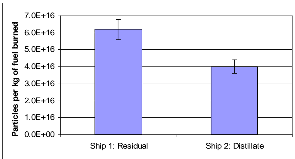
Figure 4-8 Exhaust Particle Concentration for Two Ships
