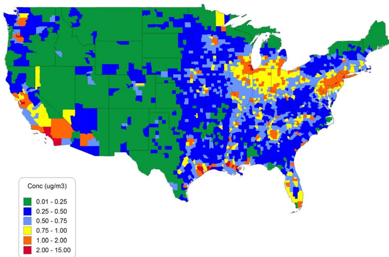
Figure 2-1 Estimated County Ambient Concentration of Diesel Particulate Matter
