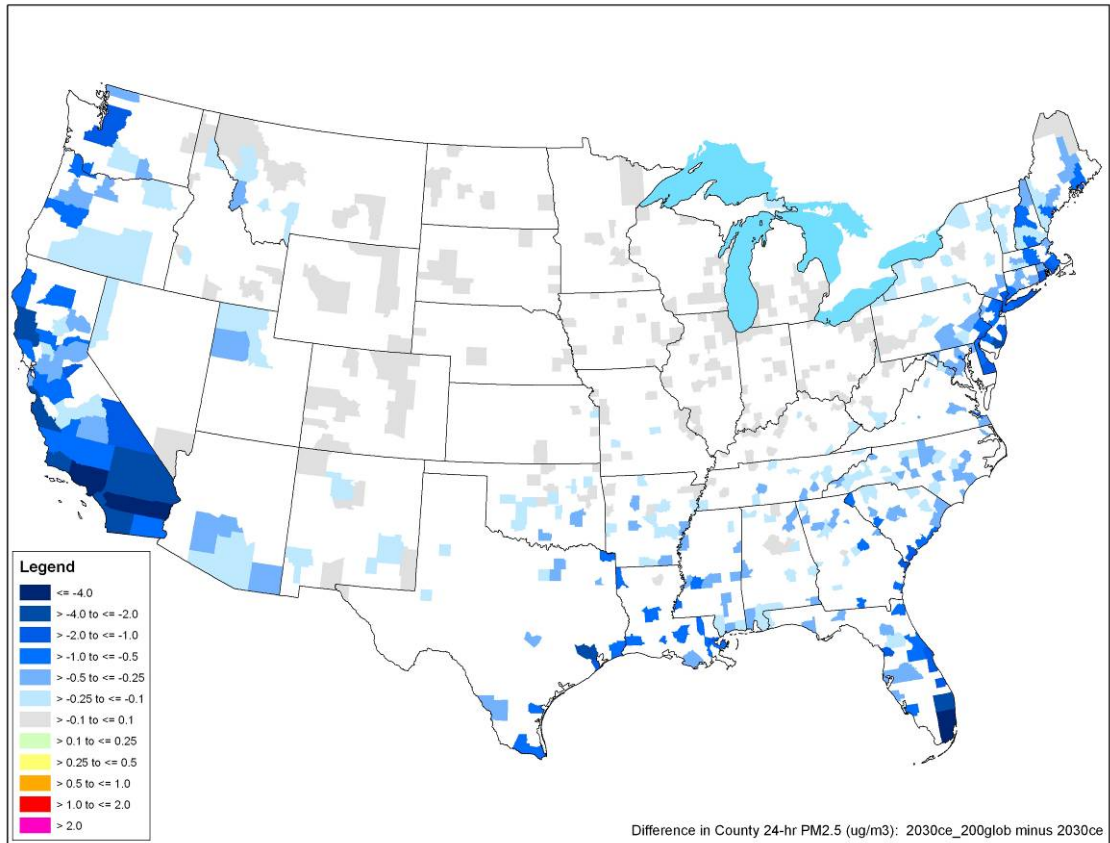
Figure 2-30 Impact of Category 3 Fuel and Engine Controls on Annual PM 2.5 Design Values (DV) in 2030 (units are \mu\text{g}/\text{m}^3 )
