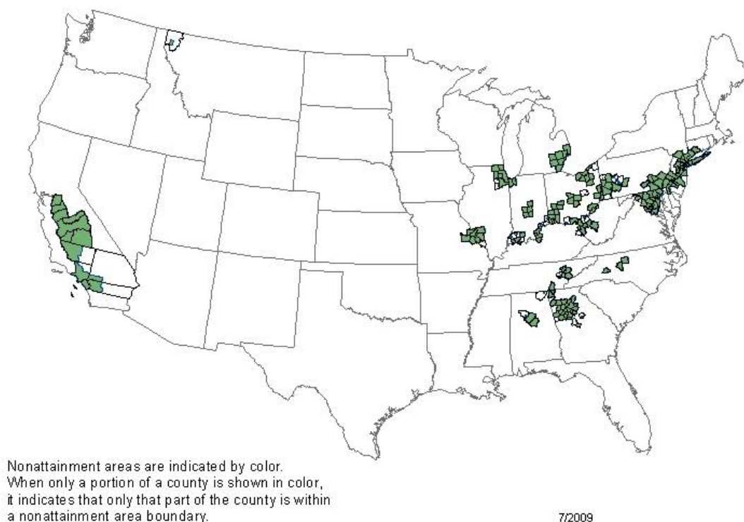
Figure 2-26 1997 Annual PM 2.5 Nonattainment Areas
