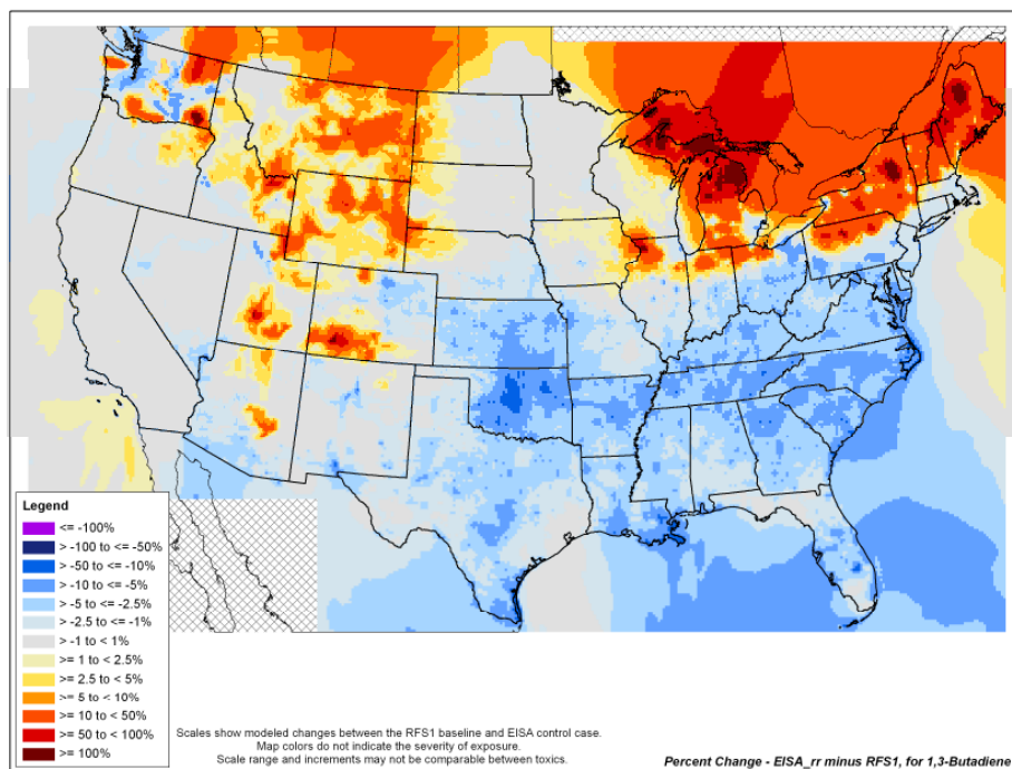
Figure III-13. 1,3-Butadiene Annual Percent Change in Concentration Between the RFS1 Mandate Reference Case and the RFS2 Control Case in 2022
