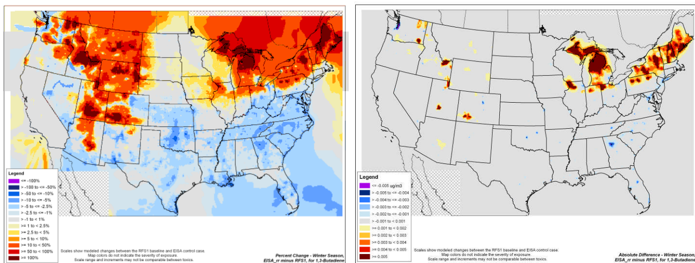
Figure III-16. Winter Changes in 1,3-Butadiene Ambient Concentrations Between the RFS1 Mandate Reference Case and the RFS2 Control Case in 2022: (a) Percent Changes and (b) Absolute Changes ( \mu\text{g}/\text{m}^3 )
