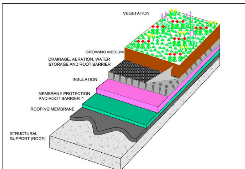
Figure 3A1-3. Green roof section.
