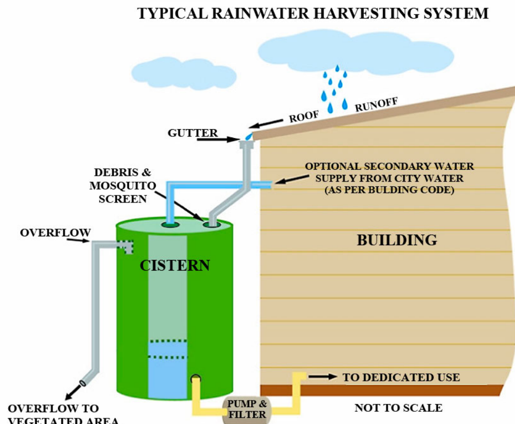
Figure 3A1-1. Typical rainwater harvesting system
