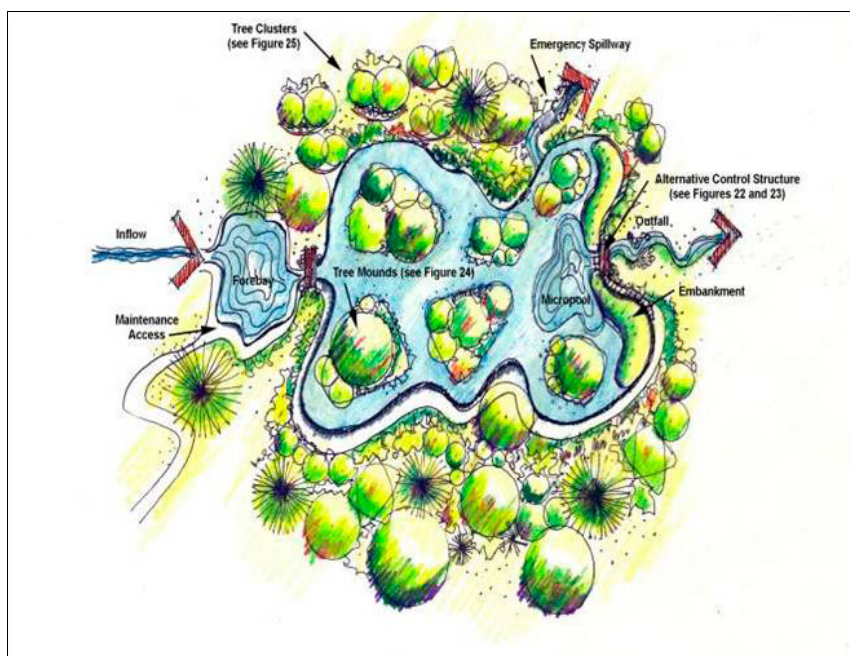
Figure 3A1-23. Plan View Constructed Wetland Basin.
