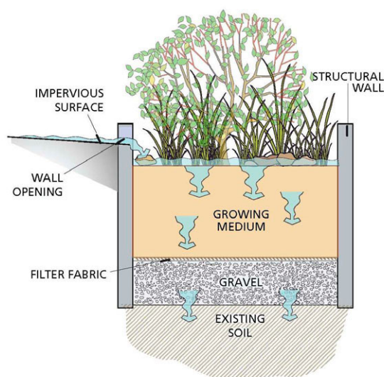
Figure 3A1-10. Infiltration planter box.
