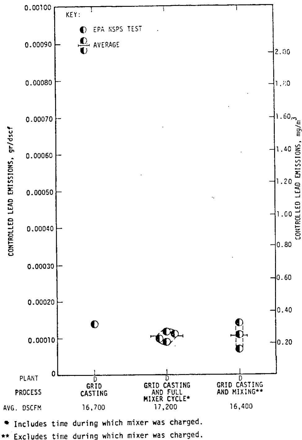
Figure 4-3. Controlled emissions from grid casting and from combined grid casting and mixing. a
