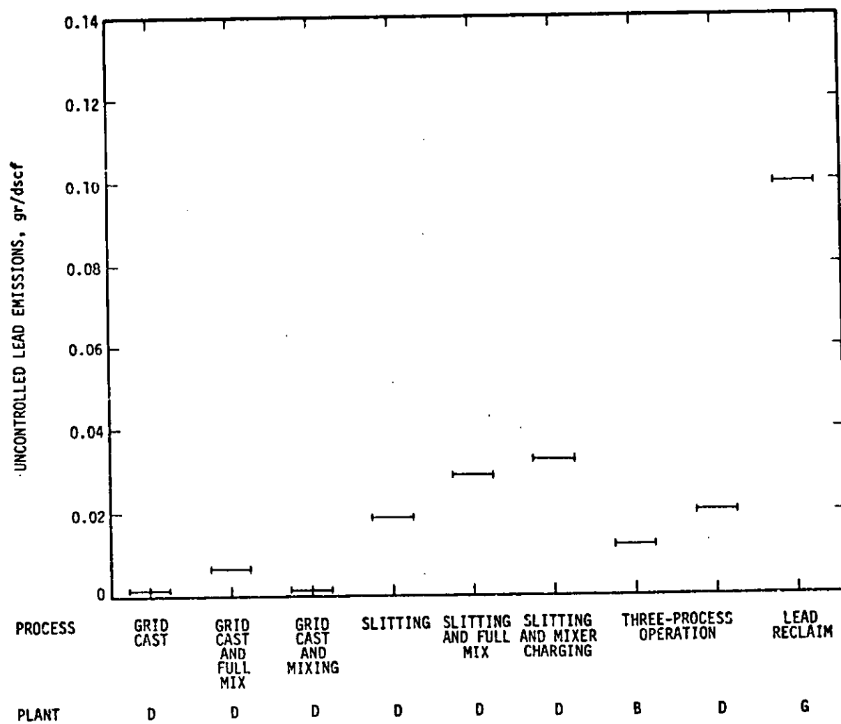
Figure 4-19. Average uncontrolled lead emissions from tested facilities (gr/dscf).
