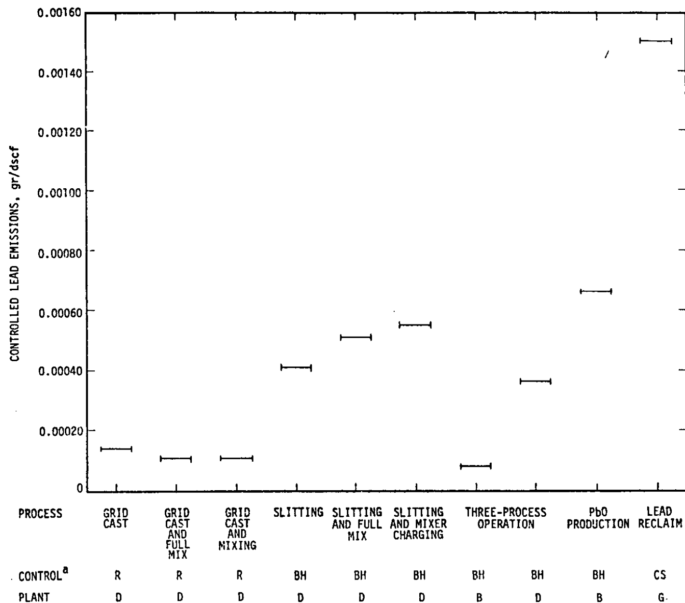
Figure 4-18. Average controlled lead emissions from tested facilities (gr/dscf).
