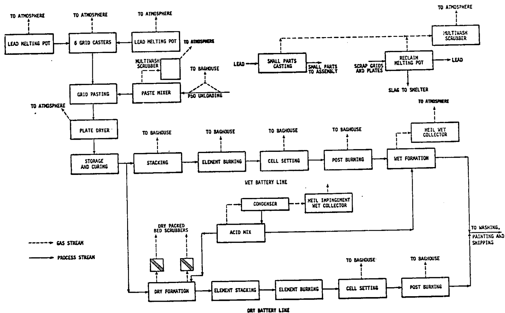
Figure C-3. Production flow diagram, Plant G.
