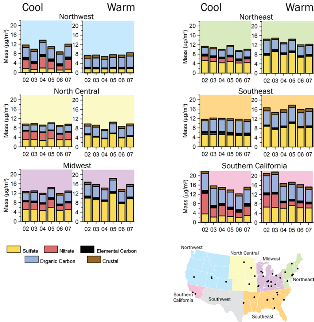
Figure 2-3. Regional and Seasonal Trends in Annual \text{PM}_{2.5} Composition from 2002 to 2007 Derived Using the SANDWICH Method. Data from the 42 monitoring locations shown on the map were stratified by region and season including cool months (October–April) and warm months (May–September)
