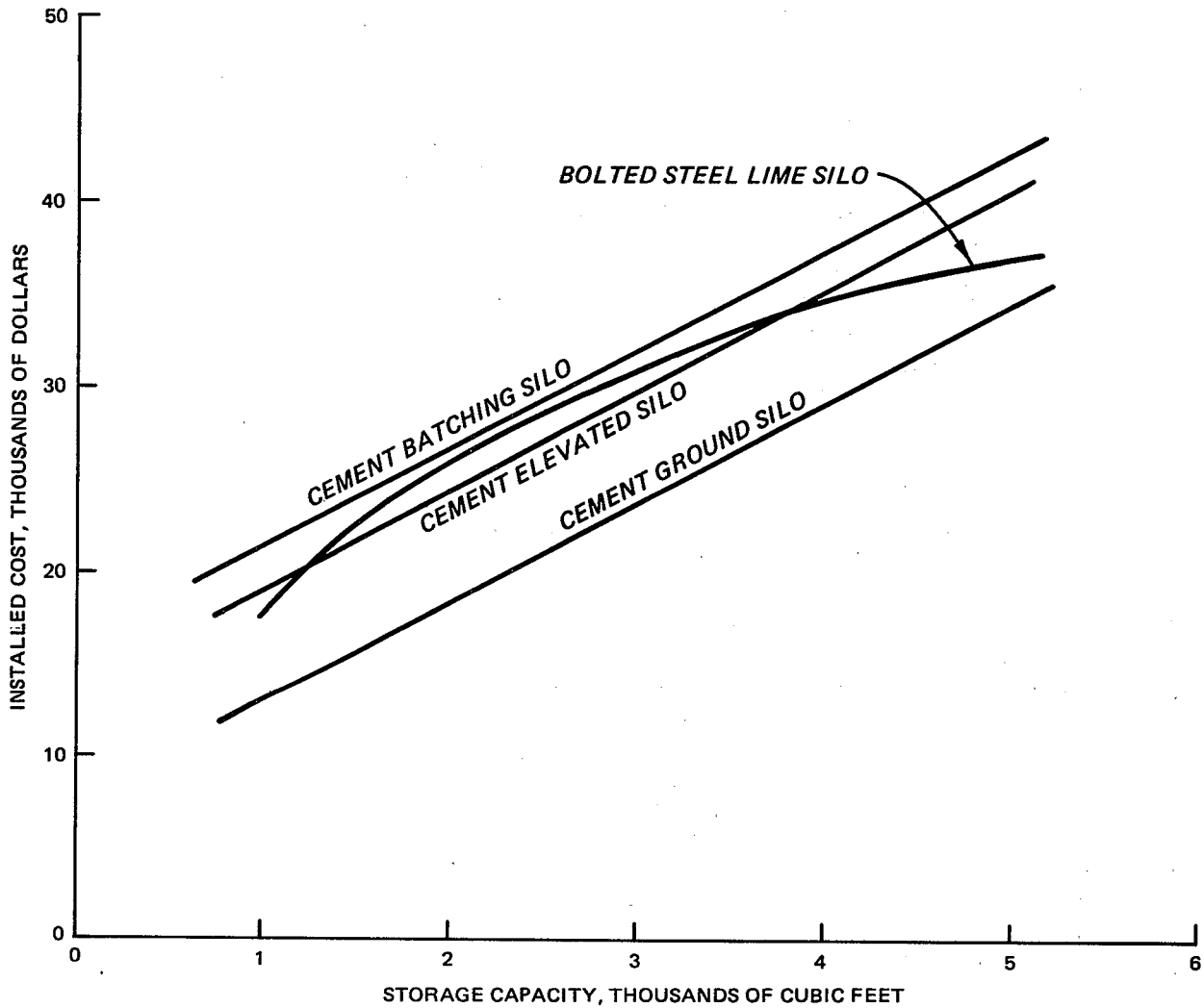
Figure B-1. Installed cost of dry chemical storage.
