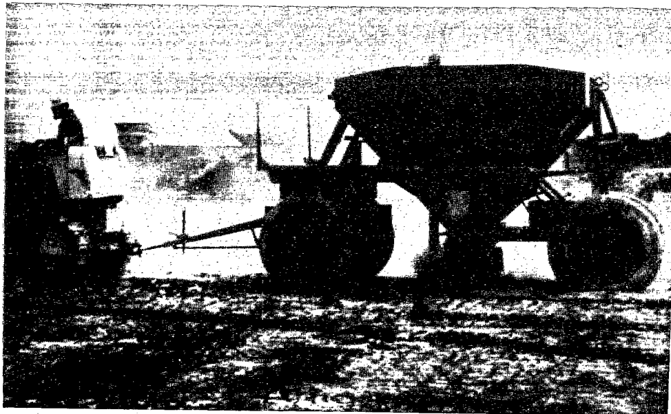
Figure 6-17. Adding stabilization/solidification reagent for area mixing (Courtesy Soil Recovery).
