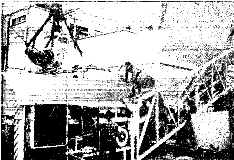
Figure B-24. Weigh batcher system for waste materials control (Courtesy Solid Tek).
