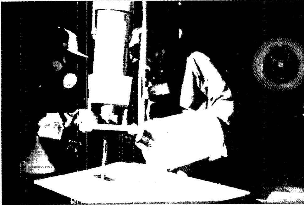
Figure 6-1. In-drum mixing using a top-entering propeller mixer.
