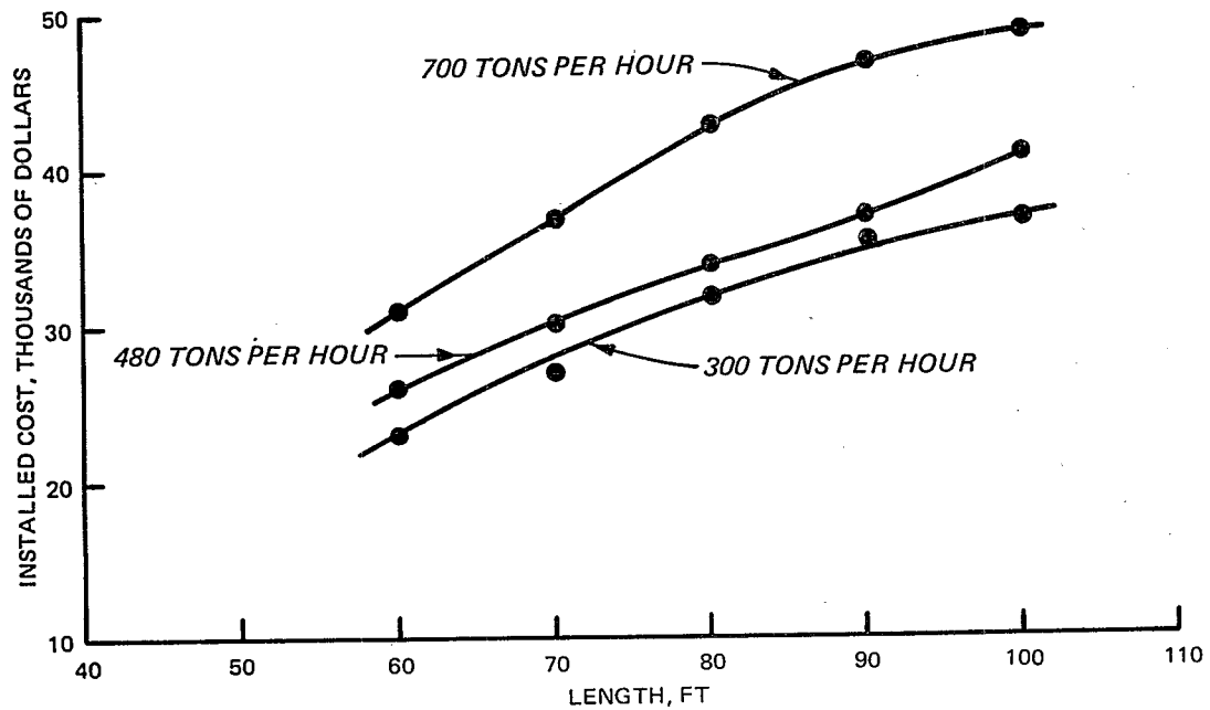
Figure B-8. Installed portable conveyor system costs.
