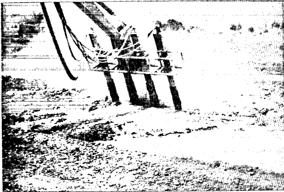
Figure 6-4. In-situ mixing by direct reagent injection (Courtesy ENRECO, Inc.).
