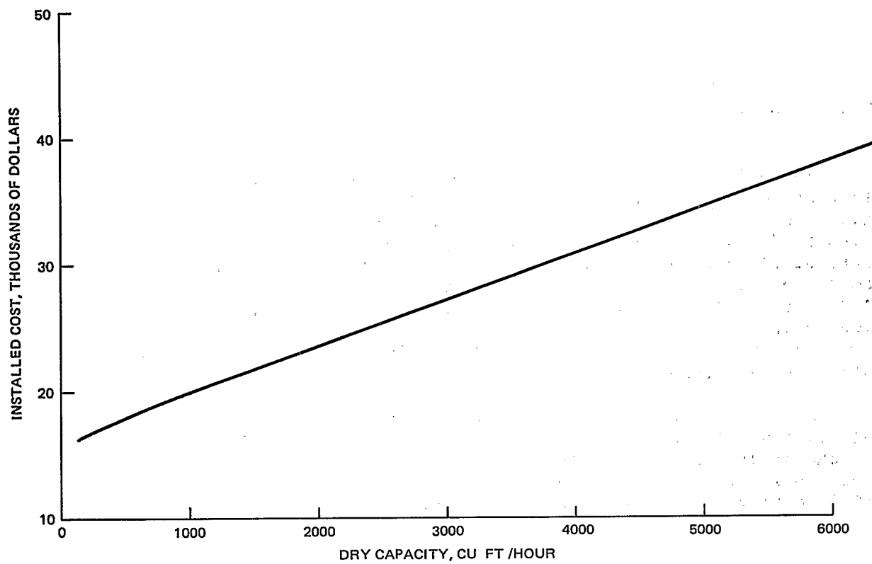
Figure B-22. Installed cost for rotor mixers.
