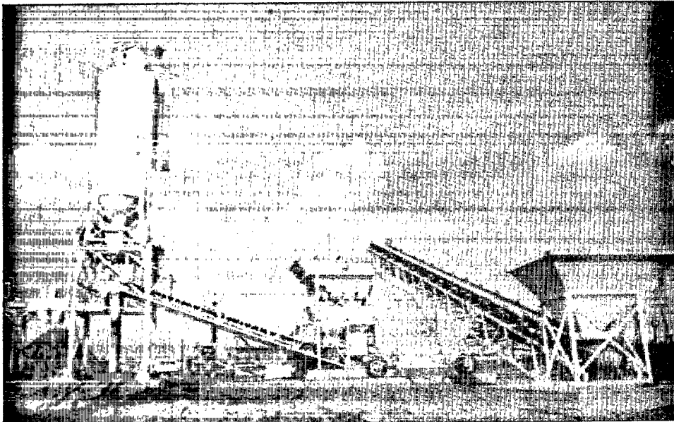
Figure B-11. Typical base stabilization plant.
