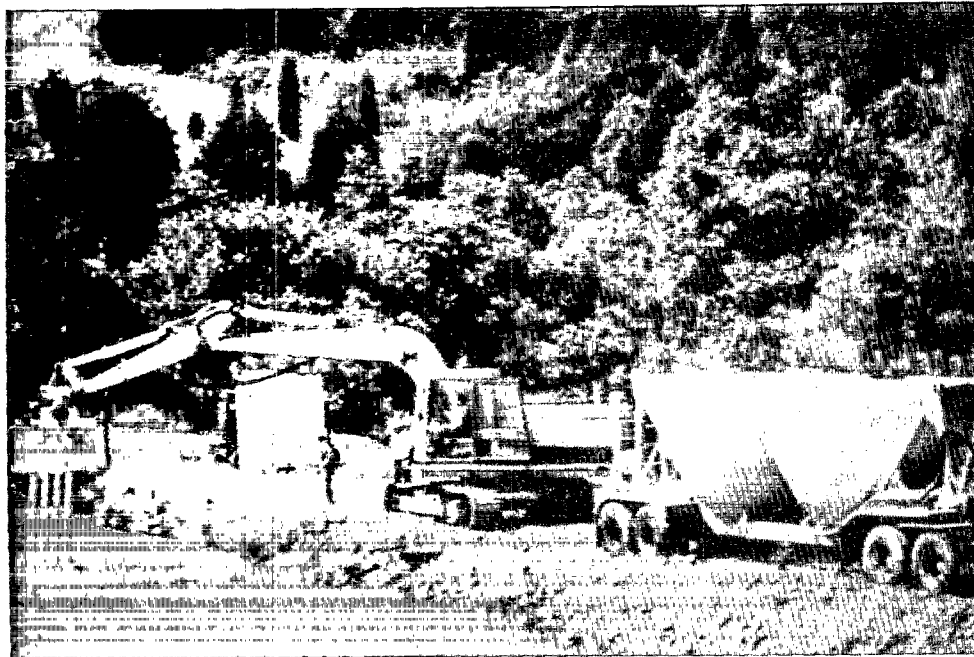
Figure 6-5. In-situ mixing equipment (Courtesy American Resources Corporation).
