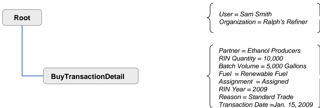
Figure E-30: Sample Structure of a Non-One-to-One Buy Transaction
