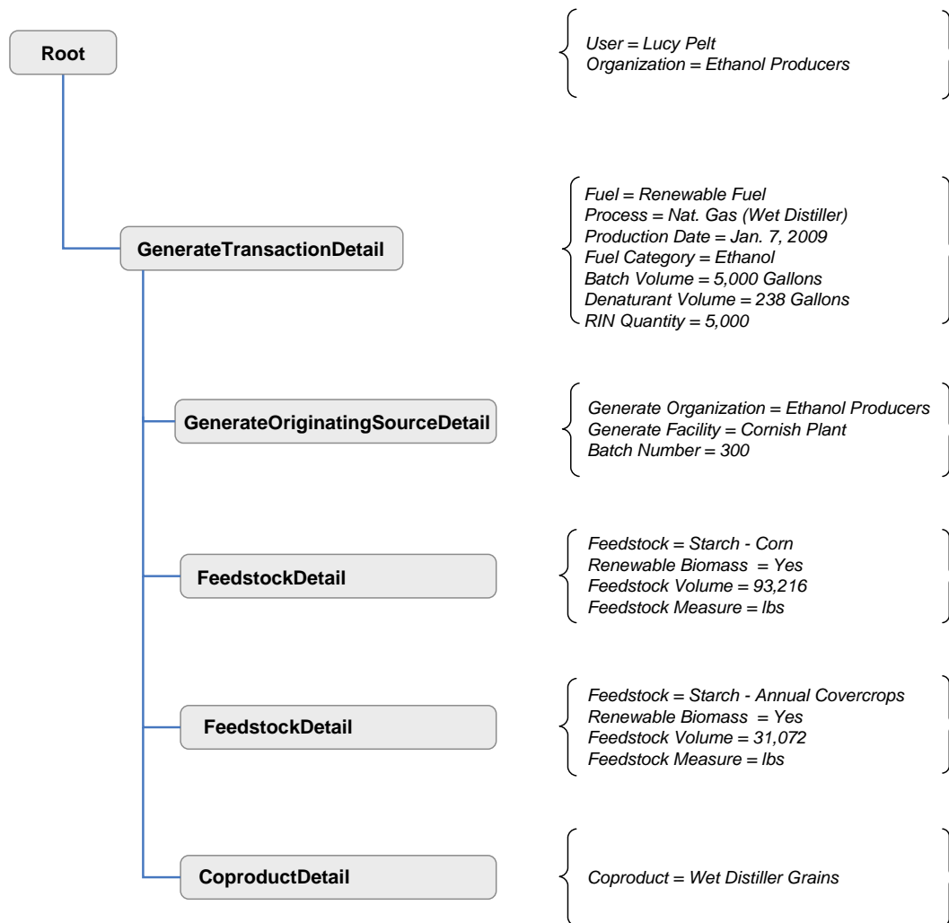
Figure E-1: General Structure of a Generate Submission
