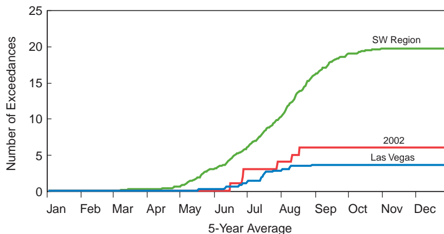
Figure 24. Cumulative exceedances—5-year average (97–01) (Las Vegas) compared to 2002 data and SW region average.
