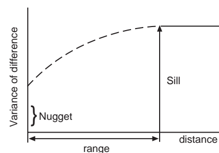
Figure 3. Schematic of a variogram.
