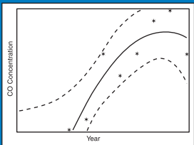
Trends in Monitored Concentrations of CO. . . . . S25
