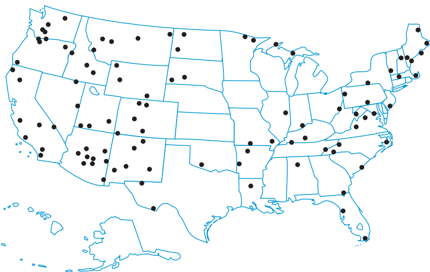
Figure 2. 98 IMPROVE locations.
