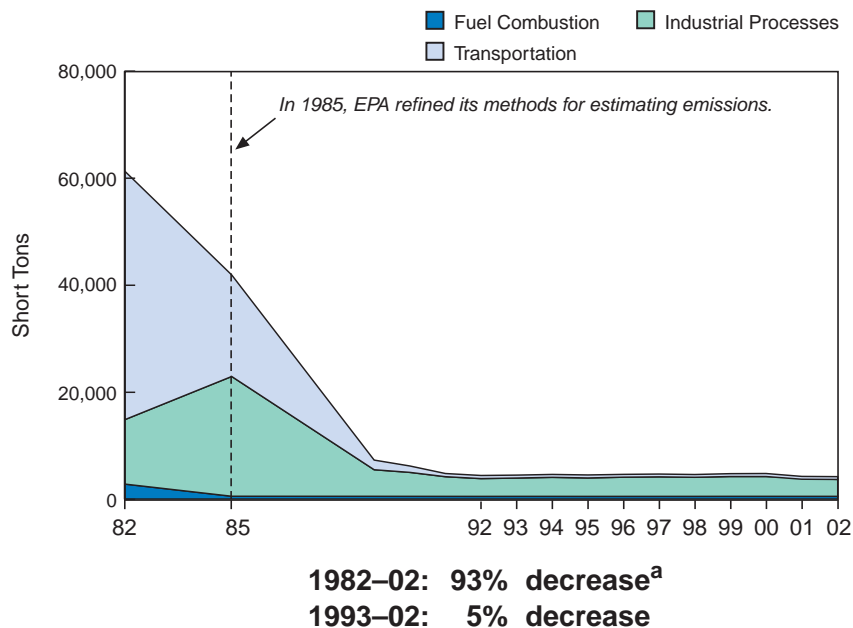
Figure 2-11. Pb emissions, 1982–2002.
