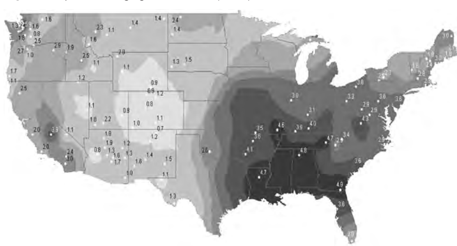
Figure 5. Spatial averaging of rural TCM ( k=1,8 ) concentrations.
