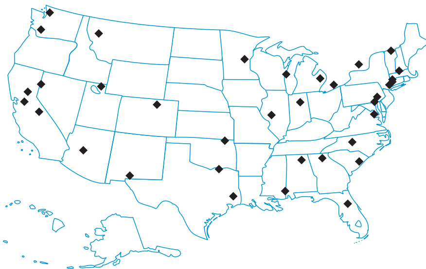
Figure 1. 35 STN locations.
