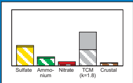
Chemical Speciation of PM 2.5 in Urban and Rural Areas. . . . . S13
