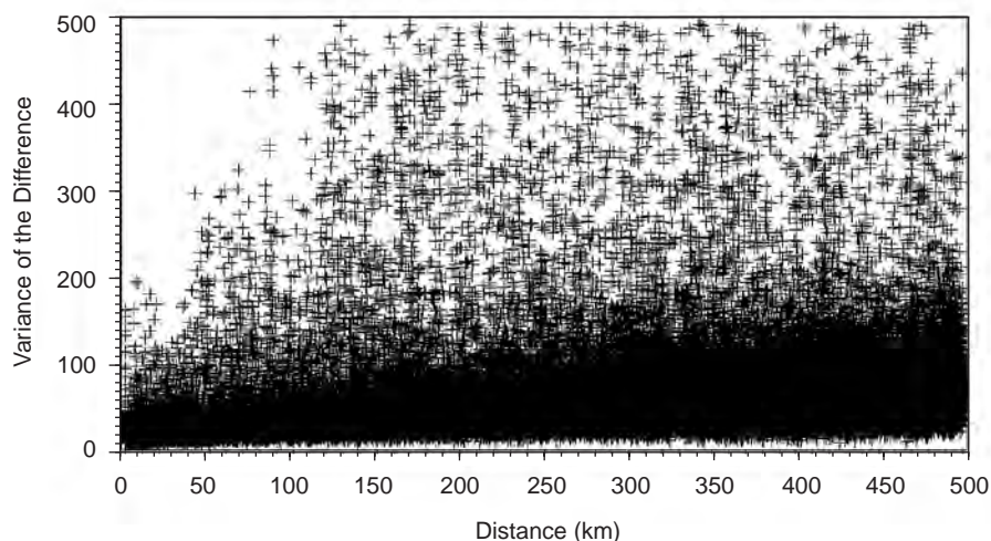
Figure 4. Variance of the difference vs. distance.
