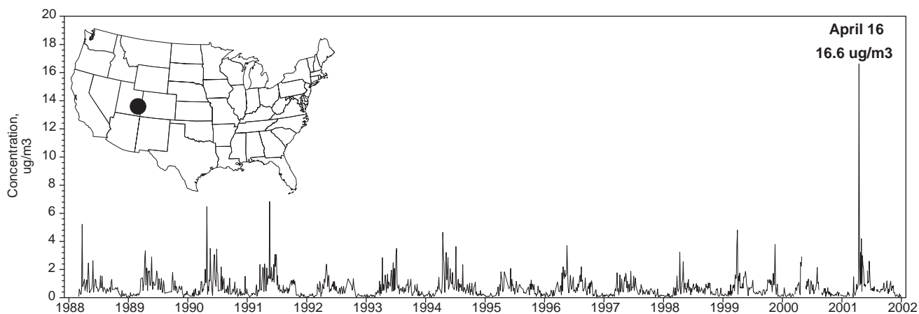
Figure 9. Historical PM 2.5 soil concentrations at Canyonlands National Park.
