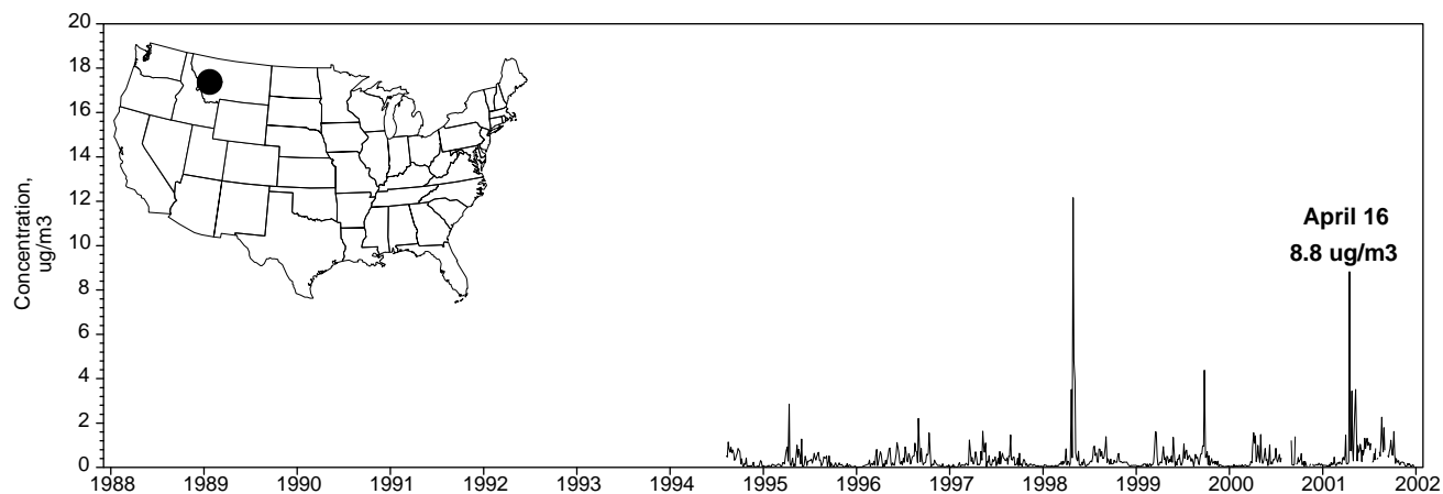
Figure 10. Historical PM 2.5 soil concentrations at Sula Wilderness Area.
