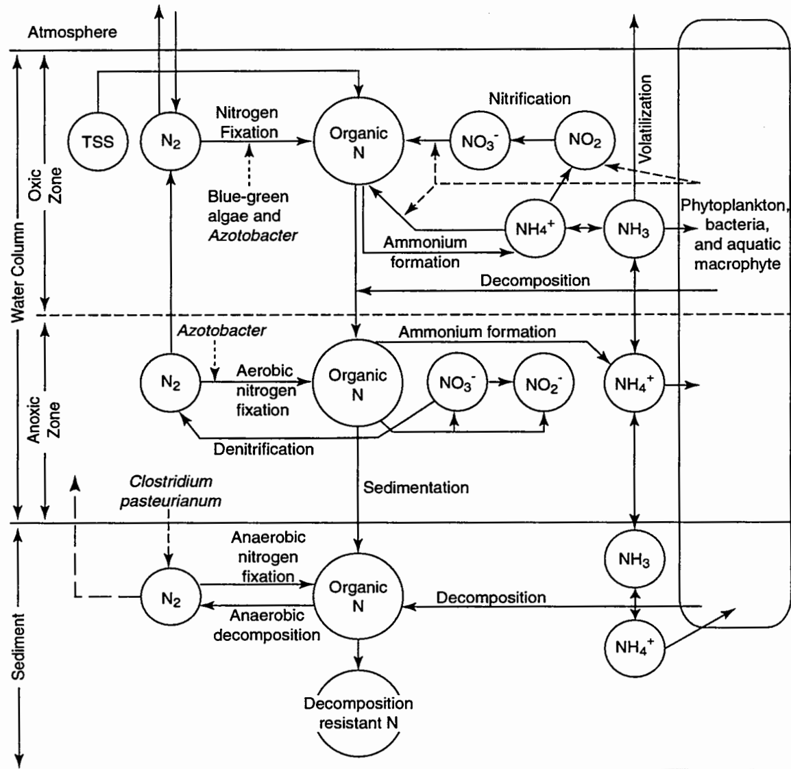
FIGURE 3-10 Nitrogen transformation processes in wetlands (Gearheart 1998, unpublished data).
