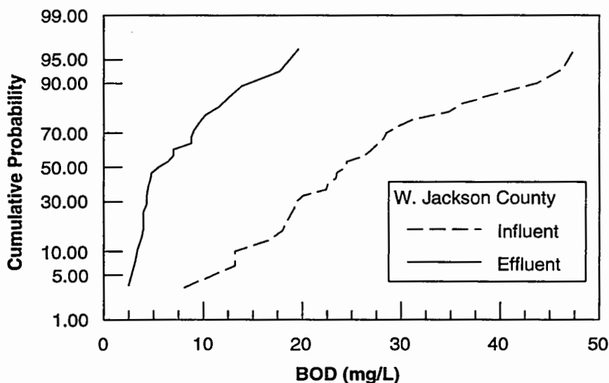
FIGURE 4-4 Influent and effluent monthly BOD cumulative probability values for West Jackson County, Mississippi.
