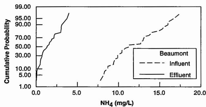
FIGURE 4-17 Ammonia nitrogen removal for Beaumont, Texas, through 8 cells with a total HRT of 17 days.
