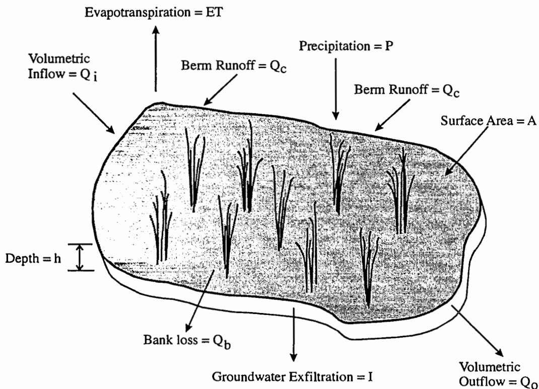
FIGURE 3-1 Components of overall wetland water mass balance (Kadlec 1993).
