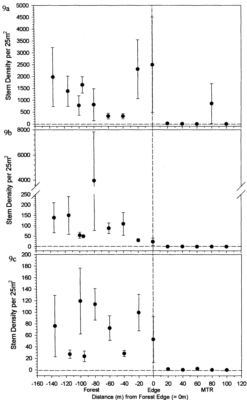
Figure 9a-9c. Mean stem density vs. distance from forest edge in three Mountain-top Removal sites (ages 6, 15, 15) and their paired forest remnants. Small woody plants are 1" (2.54cm) or smaller in diameter at base (9a). Medium woody plants are 1-3" (2.54-7.62cm) diameter at base (9b). Large woody plants are 3" (7.62cm) or larger diameter at base (9c). Forest edge is represented by vertical dashed line.
