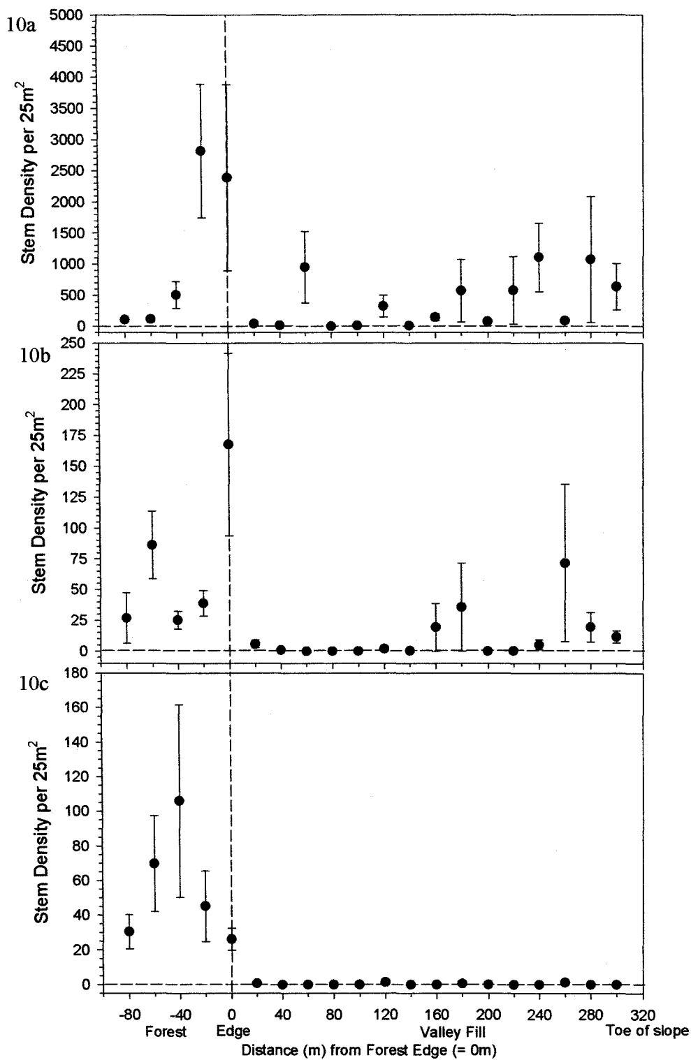
Figure 10a-10c. Mean stem density vs. distance from forest edge in three Valley Fill sites (ages 14, 17, 19) and their paired forest remnants. Small woody plants are 1" (2.54cm) or smaller in diameter at base (10a). Medium woody plants are 1-3" (2.54-7.62cm) diameter at base (10b). Large woody plants are 3" (7.62cm) or larger diameter at base (10c). Forest edge is represented by vertical dashed line.
