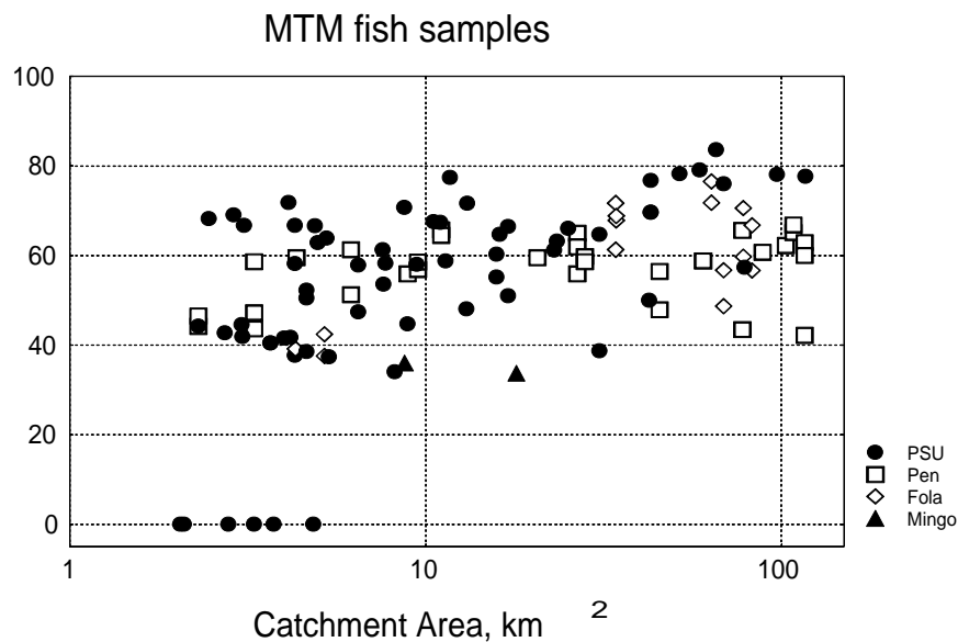
Figure 4-2. Calculated Fish IBI and watershed catchment area, all MTM fish samples from sites with catchment > 2km 2 . Symbols identify sampling organizations: PSU=Penn State; Pen = Pen Coal (REIC); Fola = Fola Coal (Potesta); Mingo = Mingo-Logan Coal (BMI).
