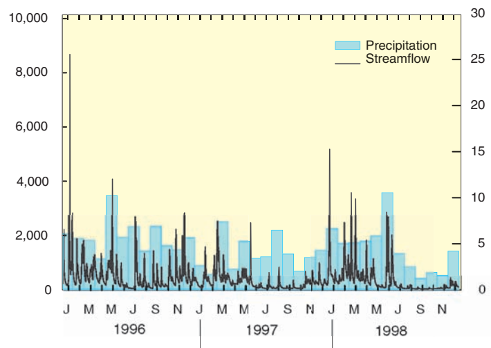
Figure 3. After a major flood in January 1996, streamflow from Williams River at Dyer, W. Va., and precipitation from Richwood, W. Va., were normal throughout the study period. The long-term average annual streamflow at Williams River at Dyer, W. Va. is 336 cubic feet per second. Long-term average precipitation at the Richwood, W. Va. location is 48 inches per year.
