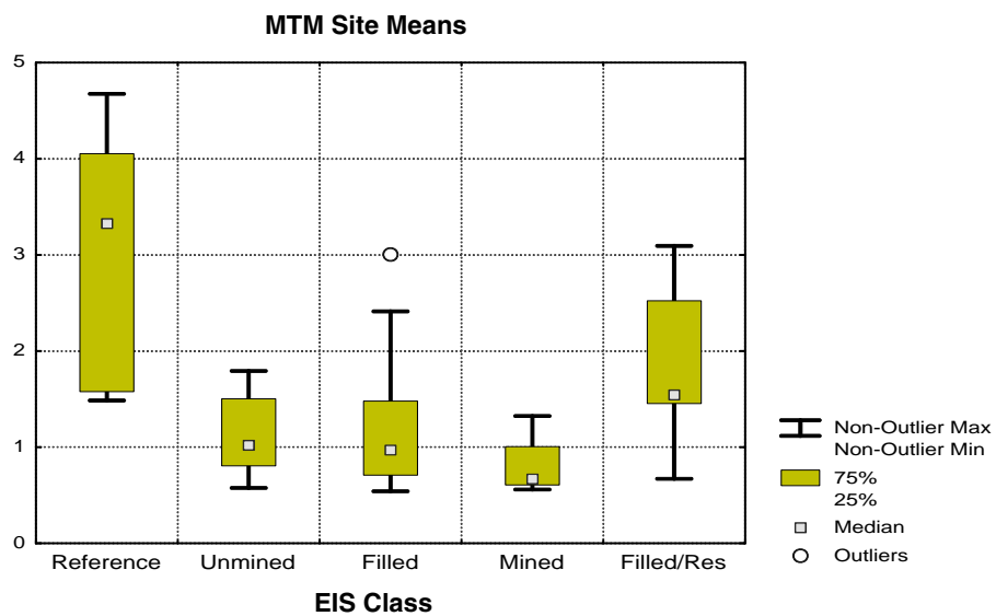
Figure B-7. Box plot of the Number of Intolerant Species among EIS classes and regional reference sites. This metric was adjusted to a catchment area of 100 km 2 .
