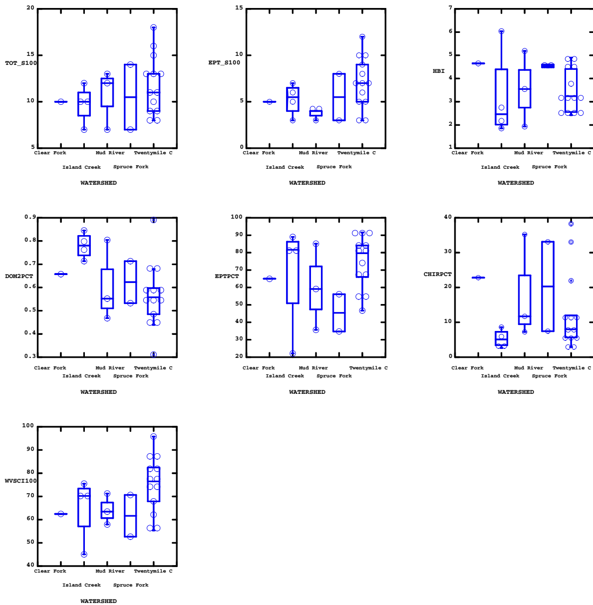
Figure C-12. Box plots of the WSCI and its component metrics versus watershed for Filled sites in the autumn 1999 season. Circles represent site scores.
