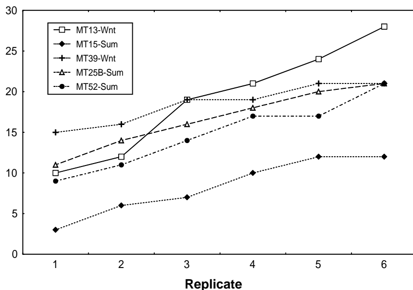
Figure E-1. Cumulative number of families identified in successive Surber samplers from 5 MTM sites.
