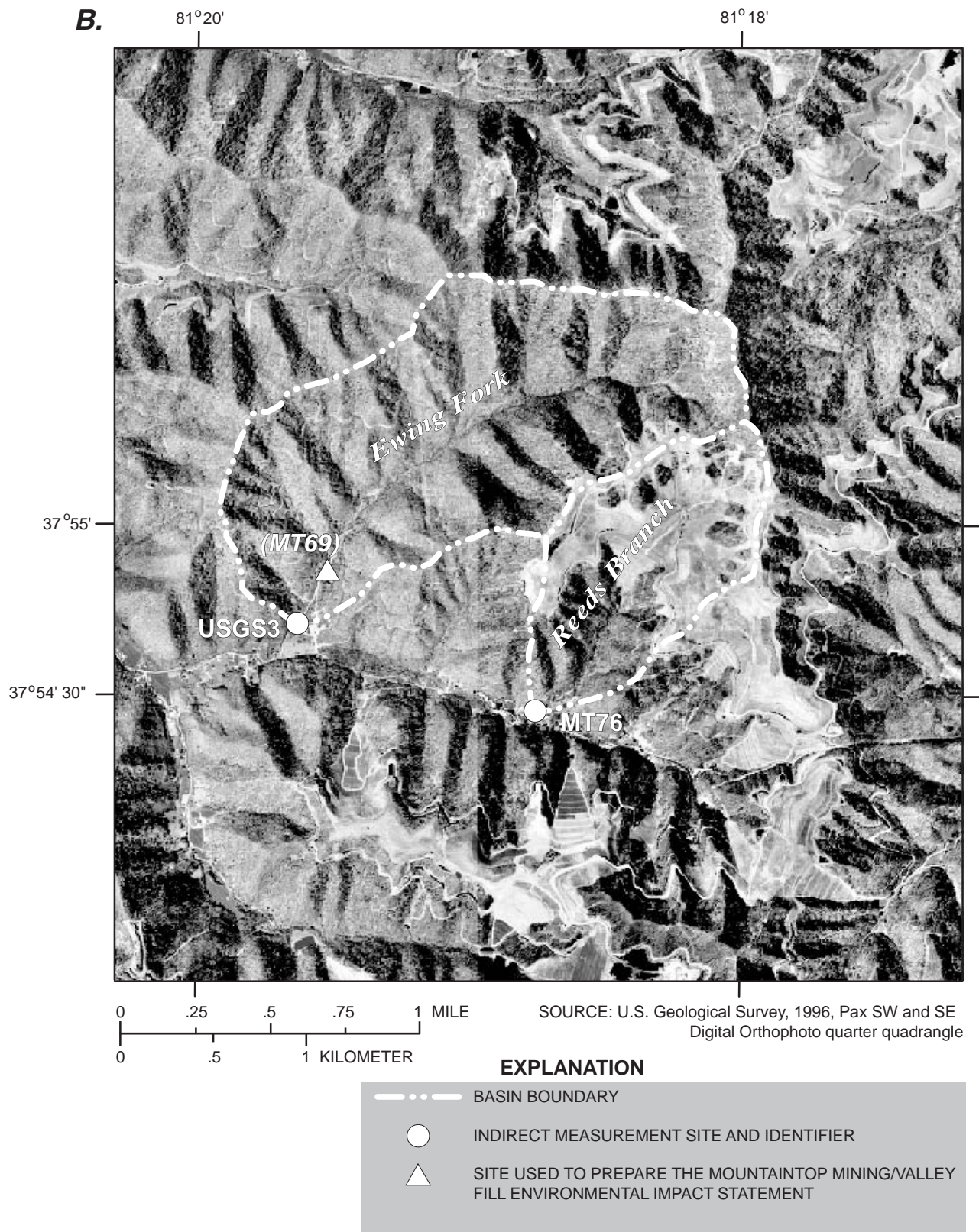
Figure 1. Study-area location of the (A) Coal River Basin, including (B) Ewing Fork and Reeds Branch (the northern basins), and (C) Unnamed Tributary to Lick Run, Unnamed Tributary to Clear Fork, Unnamed Tributary to Buffalo Fork, and Buffalo Fork (the southern basins), Coal River Basin, mountaintop coal-mining region, southern West Virginia— Continued .
