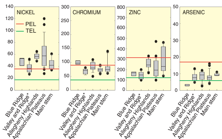
Figure 16. Some trace element concentrations in stream-bed sediment exceeded Environment Canada's effects-based criteria at several sites in the basin. Probable effects levels (PEL) are those concentrations at which harmful effects to aquatic life are thought to be likely, and were exceeded most frequently in the Allegheny Highlands and other Appalachian Plateaus streams. Threshold effects levels (TEL) were exceeded at all sites by nickel and chromium. *Valley and Ridge sites include transition zones between provinces.
