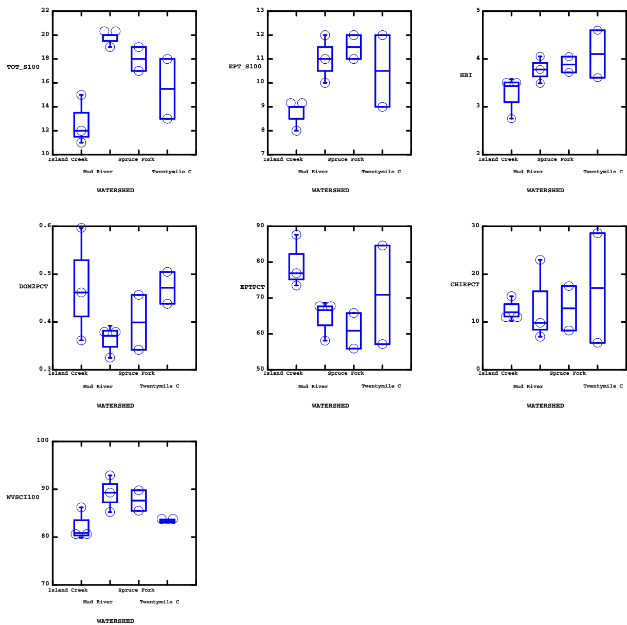
Figure C-10. Box plots of the WSCI and its component metrics versus watershed for unmined sites in the spring 2000 season.
