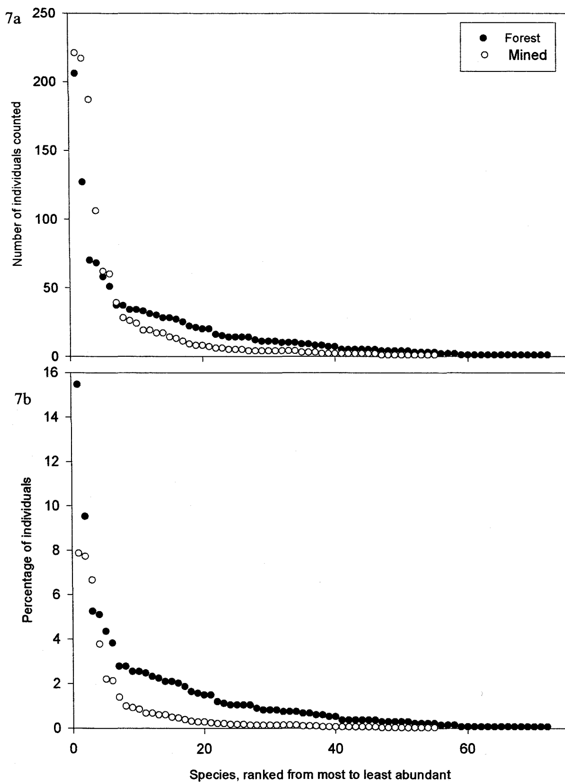
Figure 7a and 7b. Figure 7a illustrates the species abundance distribution, while Figure 7b shows the percent species abundance. Based on 1332 forest points and 2808 mined points. Contour mines excluded.
