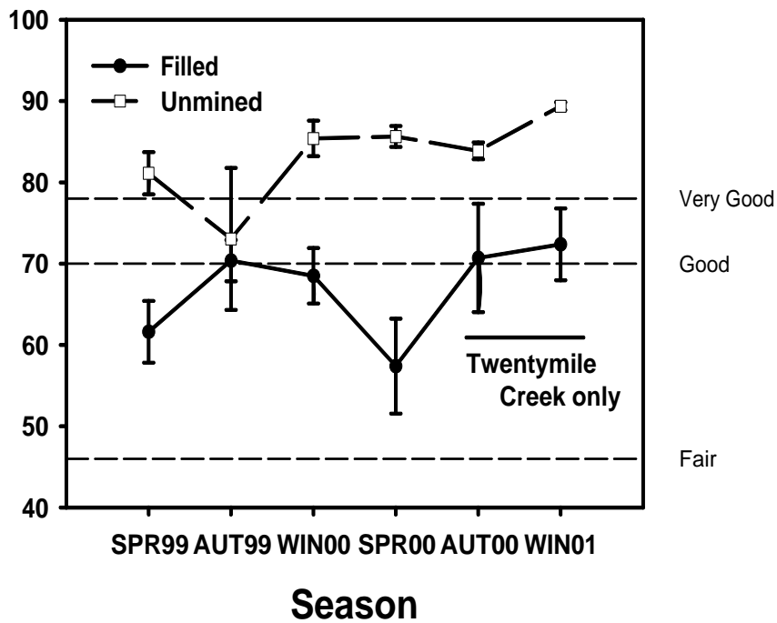
Figure 5-1. Mean WVSCI scores in the Unmined and Filled EIS classes versus sampling season. Error bars are 1 SE. Data for autumn 2000 and winter 2001 only used private organization data for the Twentymile Creek Watershed. The condition categories are based on Green et al. (2000 Draft).
