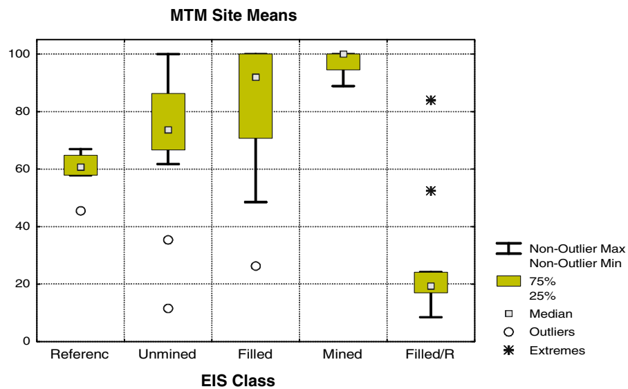
Figure B-10. Box plot of the Percent Tolerant Fish among EIS classes and regional reference sites.
