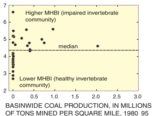
Figure 8. Only sites with little recent coal production had healthy invertebrate communities as measured by low (favorable) scores on the Modified Hilsenhoff Biotic Index, although not all impaired sites were in areas of high coal production.
