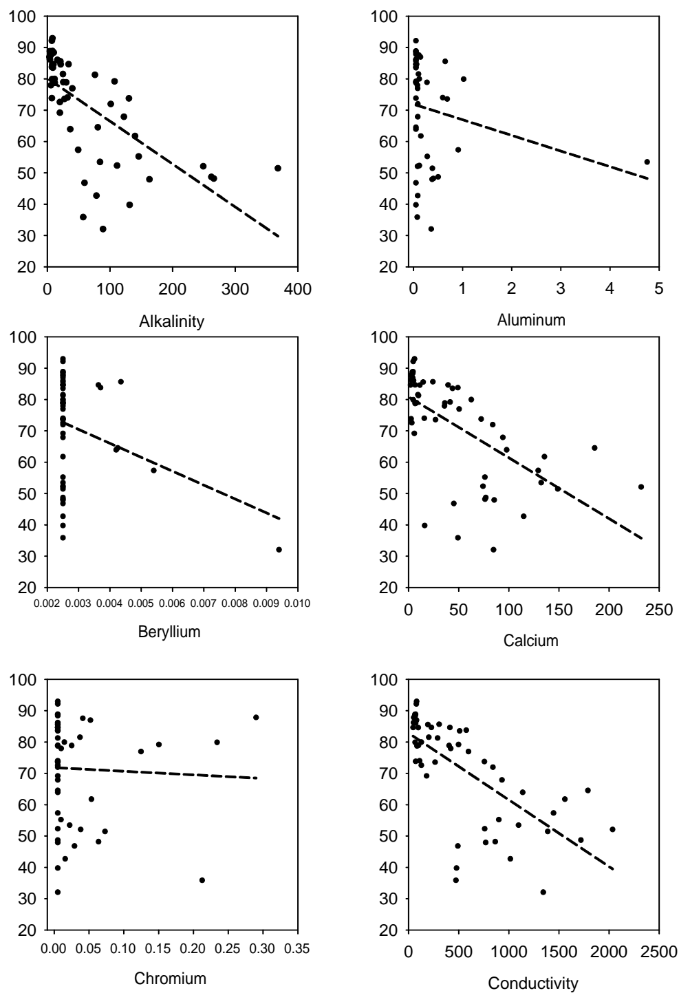
Figure D-1. The WVSCI, rarefied to 100 organisms, versus water quality parameters. Dashed line represents best fit line using linear regression.
