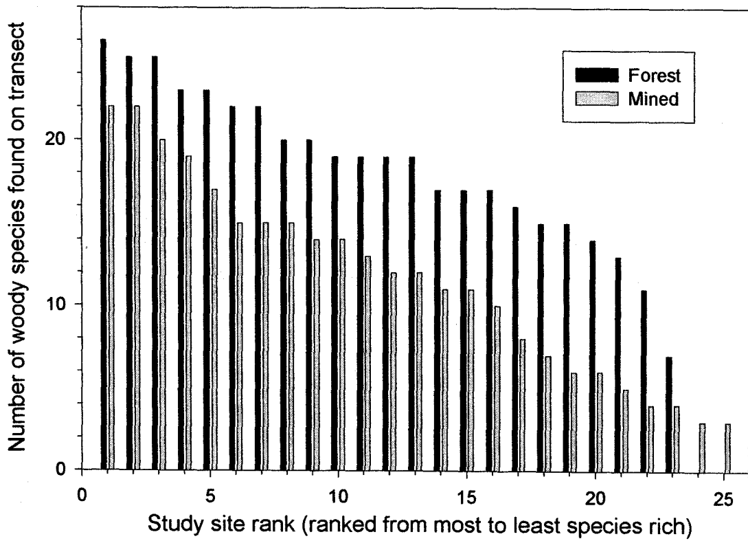
Figure 4. Woody species richness on all study sites. Sites are ranked not in pairs, but in decreasing species richness. Contour mine data not included.
