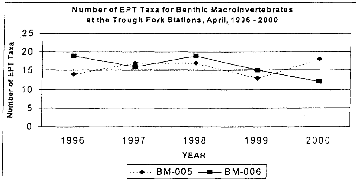
FIGURE 7. Number of EPT taxa of benthic macroinvertebrates collected in April at the upstream (BM-005) and the downstream (BM-006) Trough Fork stations. Pen Coal Corporation, May 2000.
