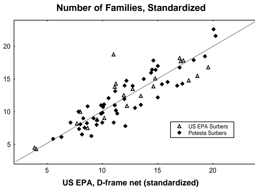
Figure E-5. Number of taxa in standardized Surber samples (vertical) compared to standardized D-frame samples (horizontal). As in Figures E-2-4.
