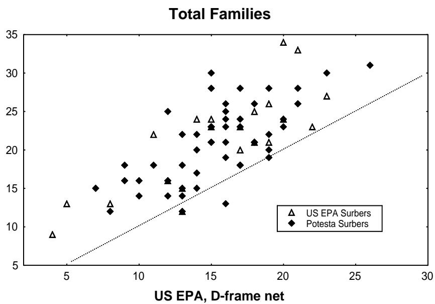
Figure E-4. Total families per site, from composite of 6 Surbers (cumulative), compared to EPA D-frame results. As in Figures E-2 and E-3.
