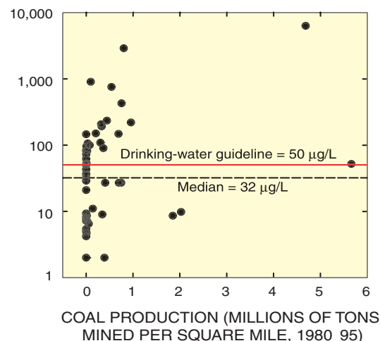
Figure 6. Concentrations of manganese in about half of the streams draining heavily mined basins were less than the study median.
