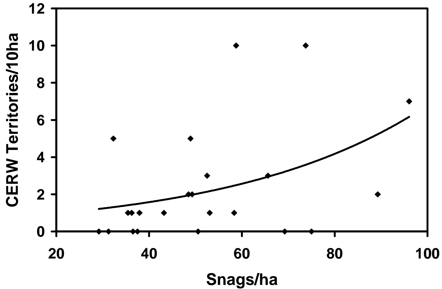
Figure 18. Relationship between Cerulean Warbler (CERW) territory density and snag density (standing dead trees >8 cm dbh).
