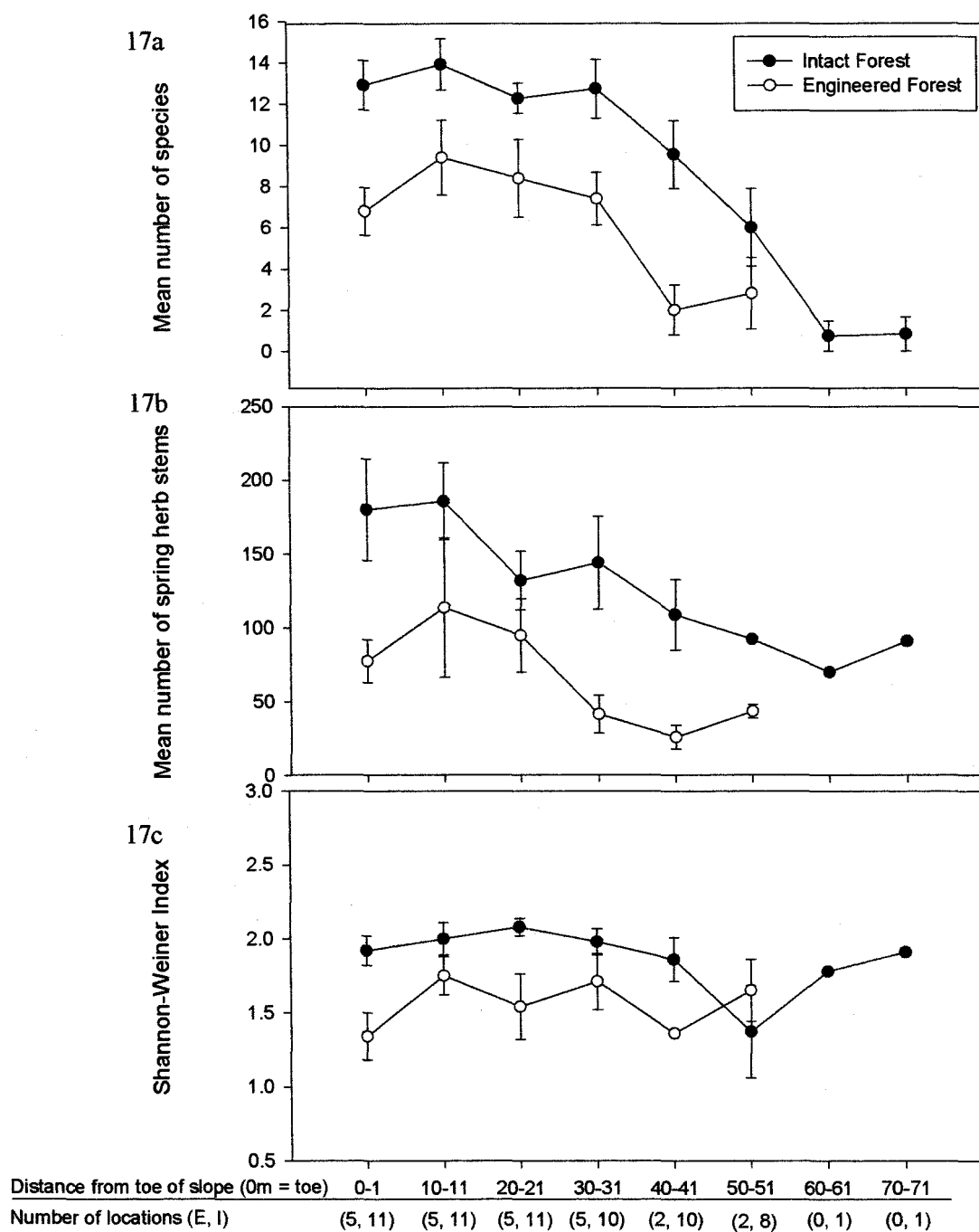
Figures 17a-17c. Mean number of spring herb species (17a), stems (17b), and estimate of biodiversity (H) (17c) for spring understory herbs in engineered forested and intact forested sites vs. distance from toe of slope. Two-way ANOVA results: treatment effect in 17a p=0.0001 , 17b p=0.0016 , 17c p=0.0030 ; distance effect 17a p=0.0001 , 17b p=0.125 , 17c p=0.0989 ; treatment and distance effect 17a p=0.26 , 17b p=0.9 , 17c p=0.3680 .
