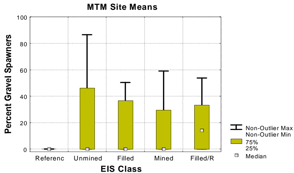
Figure B-5. Box plot of the Percent Gravel Spawners among EIS classes and regional reference sites.
