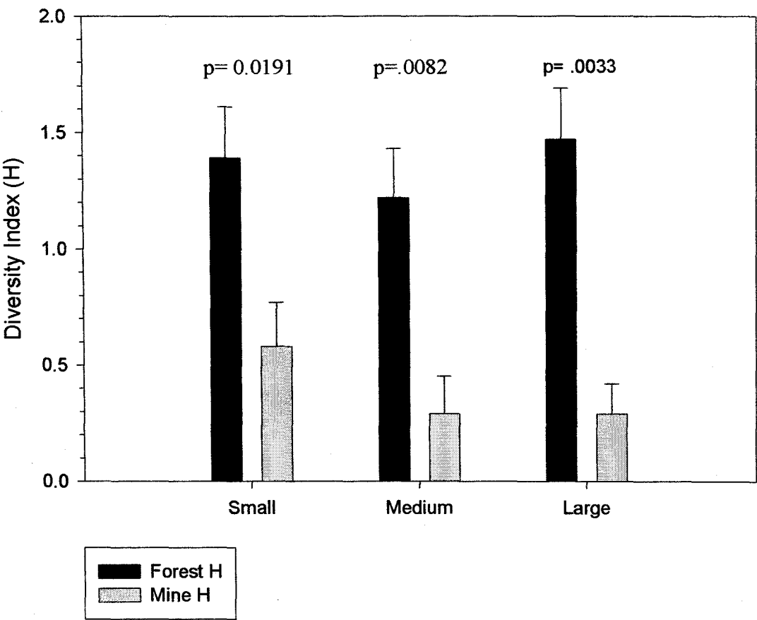
Figure 15. Shannon-Weiner diversity Index (H) for woody trees in all three size classes. Comparison of mined lands to forest remnants (contour mines excluded). A paired t test was performed with df= 8 , t (small) = 2.92, t (medium) = 3.49, t (large) = 4.13.
