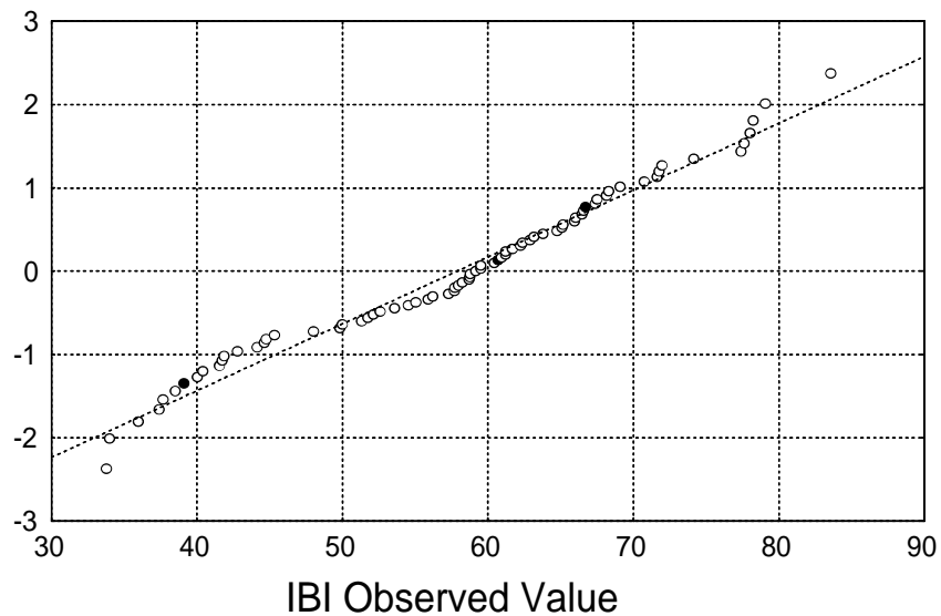
Figure 4-4. Normal probability plot of IBI scores from EIS classes.
