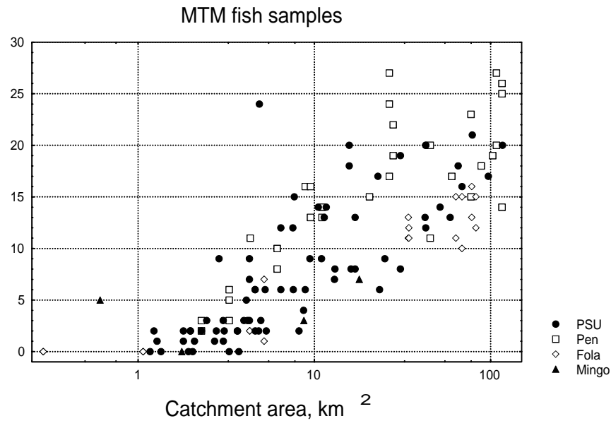
Figure 4-1. Number of fish species captured versus stream catchment area. Symbols identify sampling organizations: PSU=Penn State; Pen = Pen Coal (REIC); Fola = Fola Coal (Potesta); Mingo = Mingo-Logan Coal (BMI).
