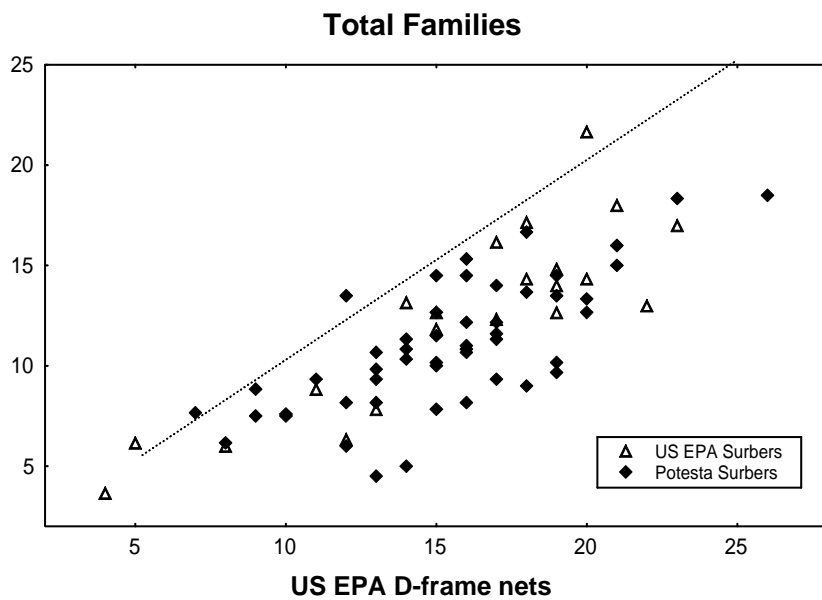
Figure E-3. Number of families per site, averaged over 6 Surbers (vertical), against total numbers from D-frame samples. See Figure E-2 caption.
