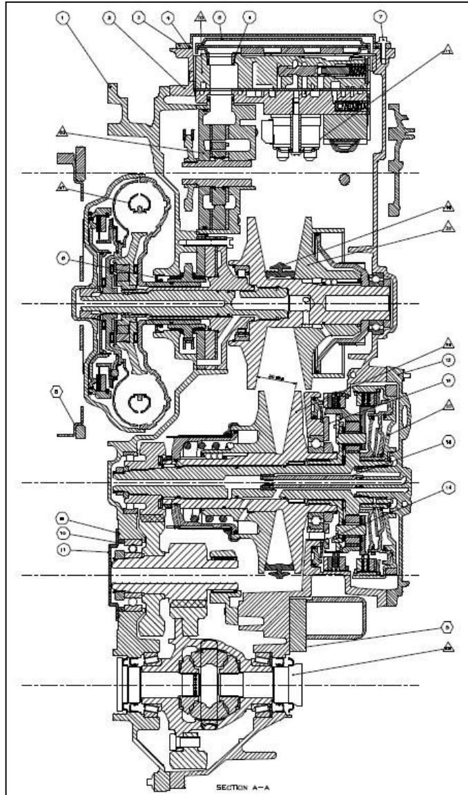
Figure 5-27: Typical transverse CVT arrangement
