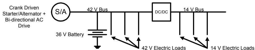
Figure 5-22: Conventional, Dual Voltage System
