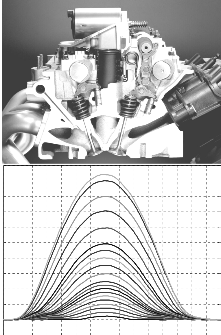
Figure 5-3: BMW “Valvetronic” continuously variable inlet valve lift system and valve lift profiles available with it
