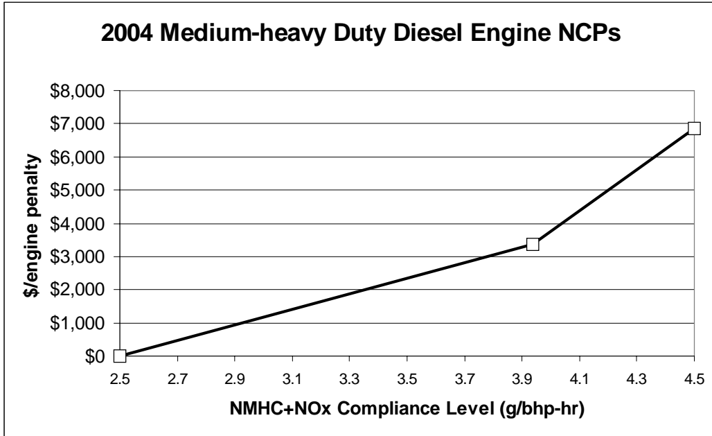
Figure 4-2: Medium-heavy Penalty Curve
