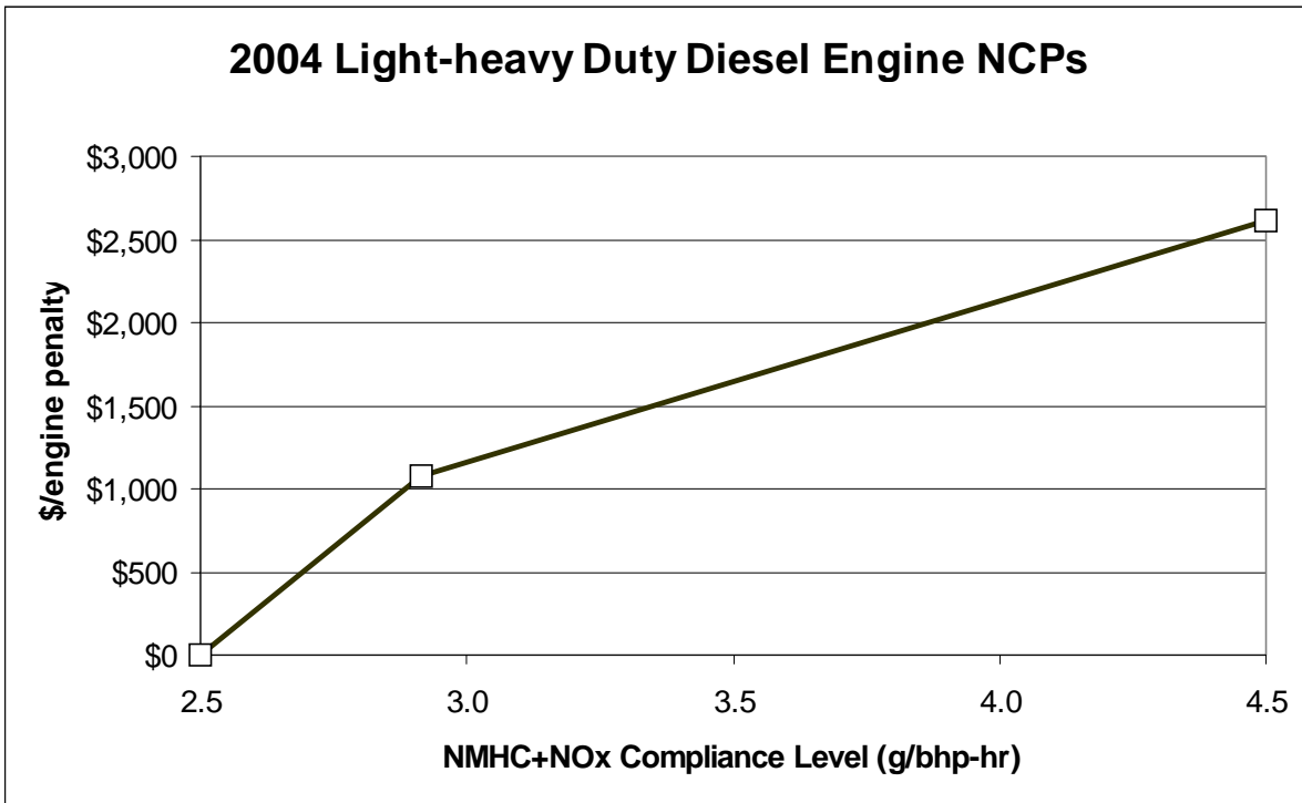
Figure 4-1: Light-heavy Penalty Curve
