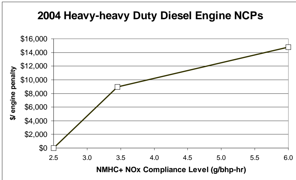
Figure 4-3: Heavy-heavy Penalty Curve
