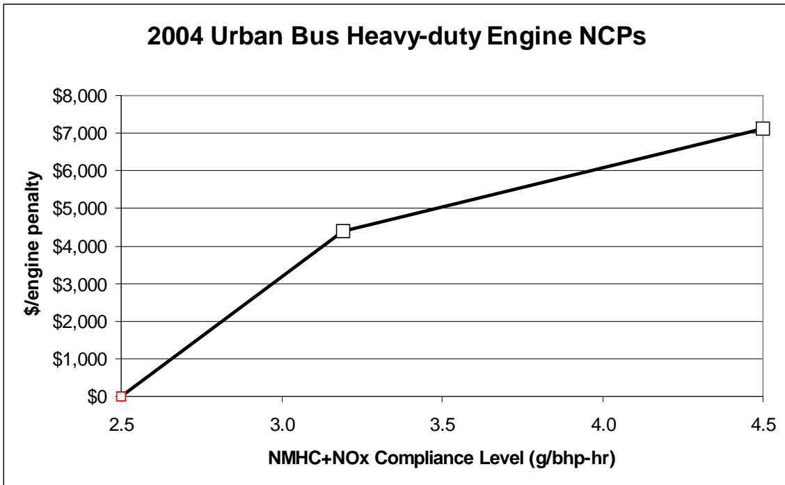
Figure 4-4: Urban Bus Penalty Curve
