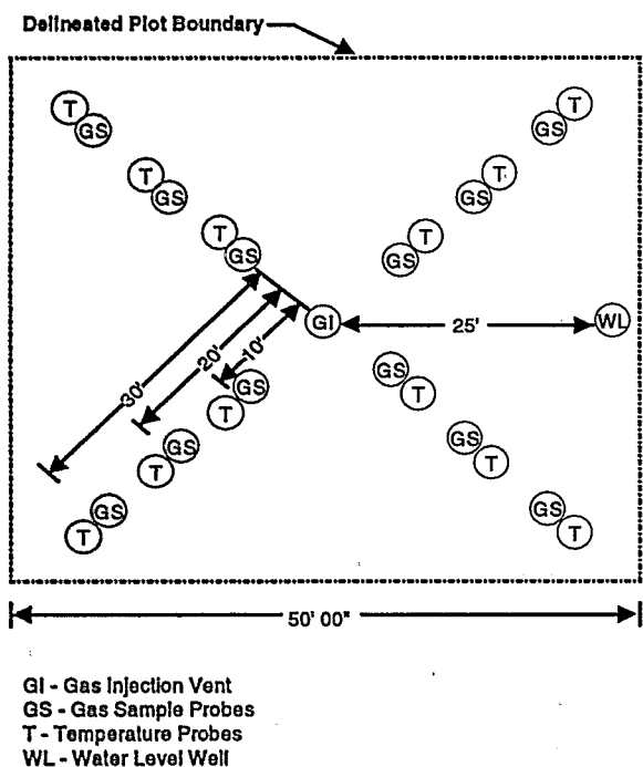
Figure 1. Layout of bioventing installation on experimental plot.
