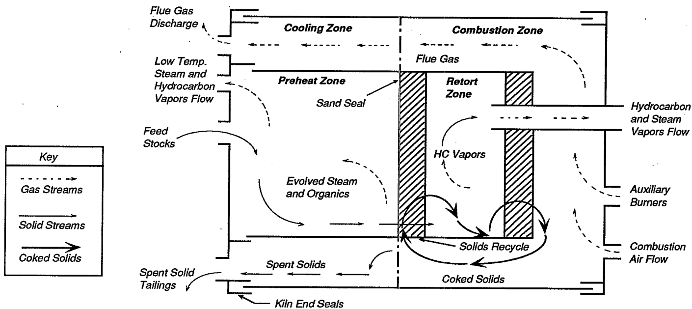
Figure 1. Simplified sectional diagram showing the four internal zones.
