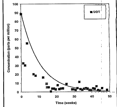
Figure 2. Typical DDT Destruction Rate at the SMC Tampa Site
