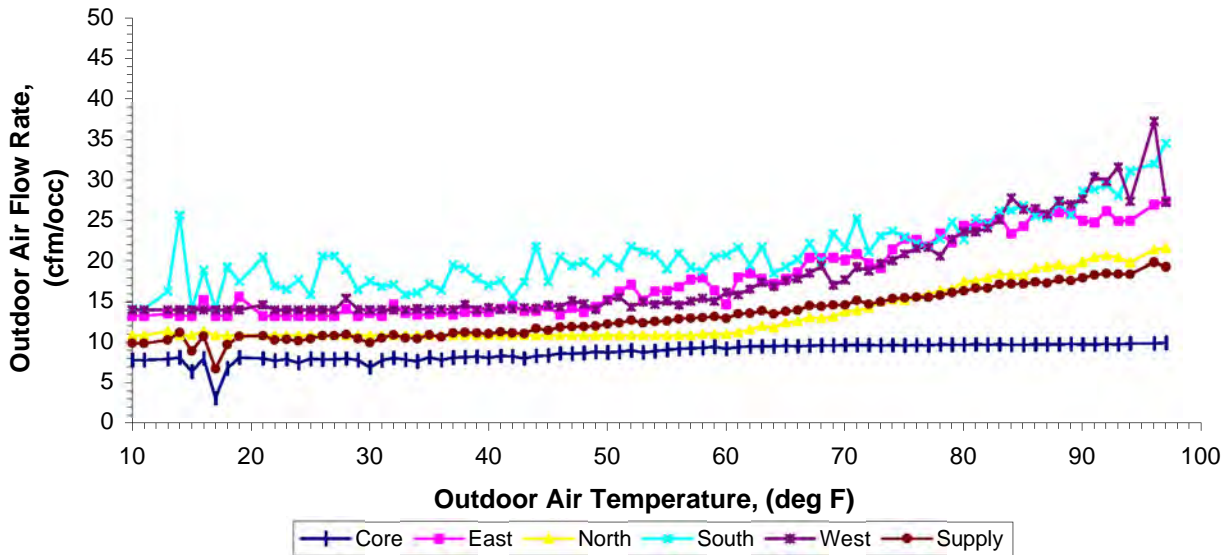
Exhibit 12b Comparison of Zone Level Outdoor Air Flow Rates for VAV (FOAF) System w/ VAV Boxes at 30%
