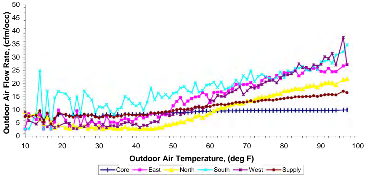
Exhibit 12a Comparison of Zone Level Outdoor Air Flow Rates for VAV (FOAF) System w/ VAV Boxes at 0%
