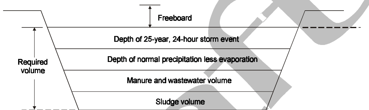
Figure 1 Cross Section of Animal Waste Storage Pond
