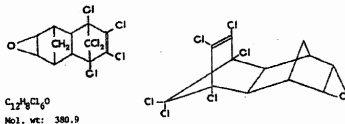
Figure 2-2. Dieldrin Chemical Structure
