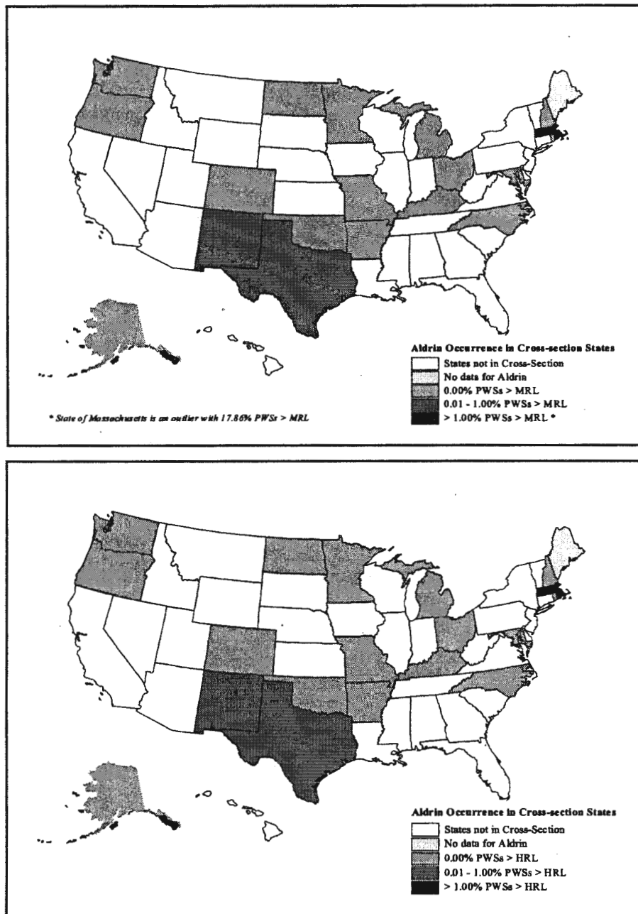
Figure 4-3. Round 2 Cross-Section States With PWSs With Detections of Aldrin (Any PWSs With Results Greater than the Minimum Reporting Level [MRL]; Above) and Concentrations Greater than the Health Reference Level (HRL; Below)
