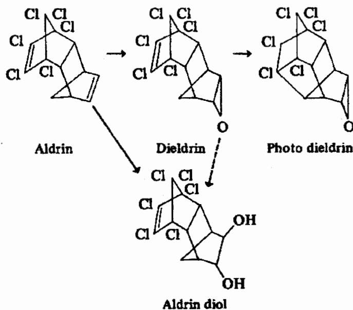
Figure 3-1. Biodegradation Pathways for Aldrin and Dieldrin, With Particular Reference to Oceanic Conditions (Verschuieren, 1983)
