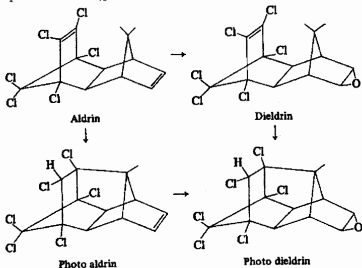
Figure 3-2. Photochemical Transformations (Principally Atmospheric) Reported for Aldrin and Dieldrin (Verschuieren, 1983)
