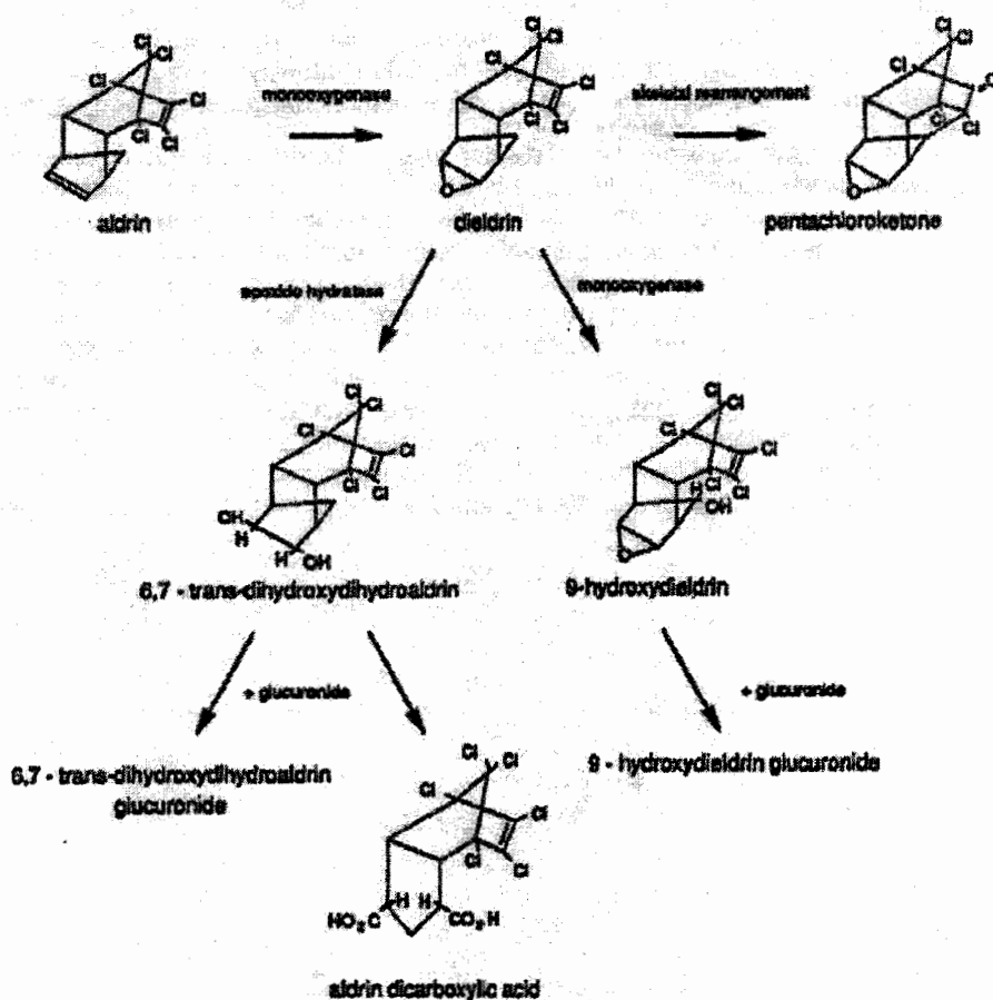
Figure 6-3. Proposed Principal Metabolic Pathways for Aldrin and Dieldrin (from ATSDR, 1993, as Adapted from USEPA, 1987)
