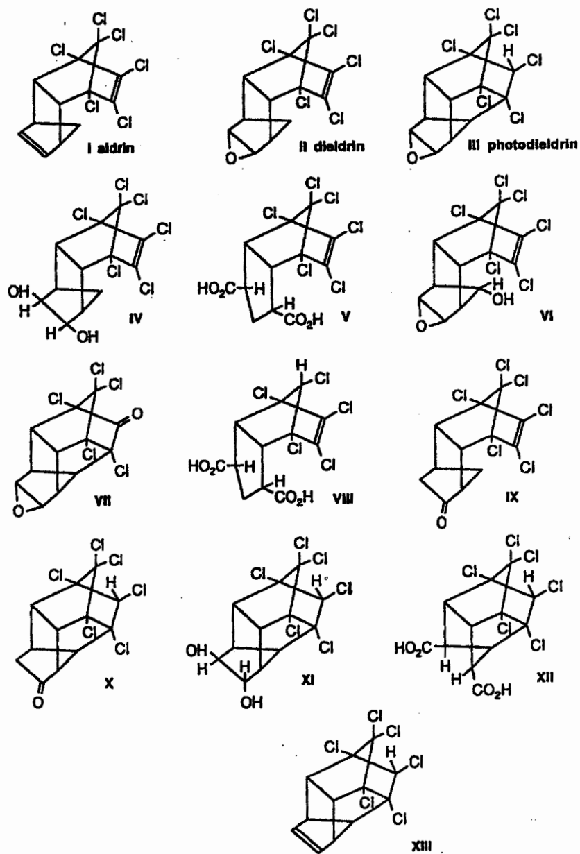
Figure 6-2. Metabolites of Aldrin and Dieldrin (from IPCS, 1989). For the Identity (Trivial Chemical Names) of These Compounds, See Table 6-3
