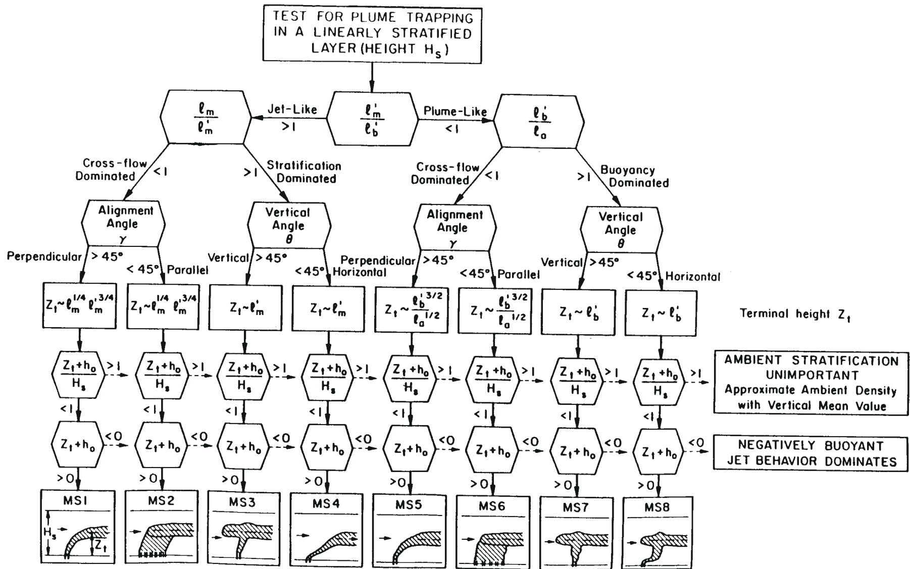
Figure 8-16. CORMIX2 sub-classification: assessment of density stratification and flow classes for internally trapped multipoint discharges.
