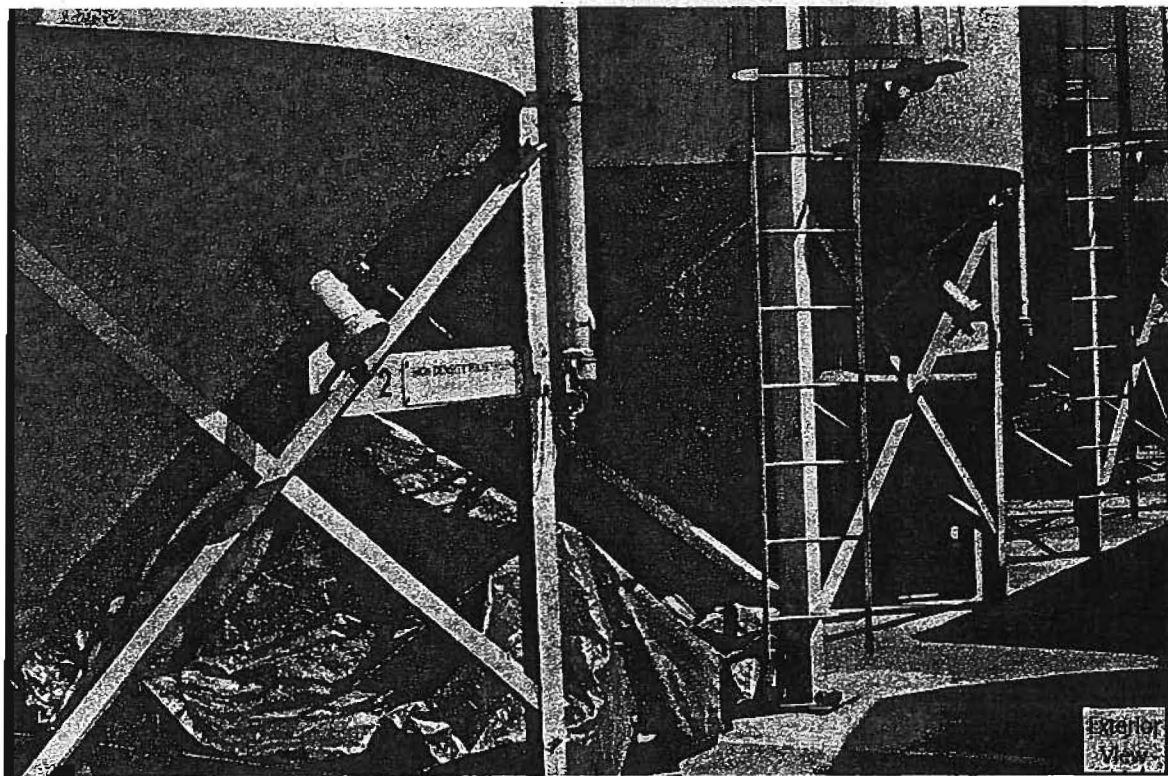
Figure 24. A Pneumatic Transfer Tube Used To Transfer Plastic Pellets from Bulk Trucks to Bulk-Storage Hoppers at Company A.
