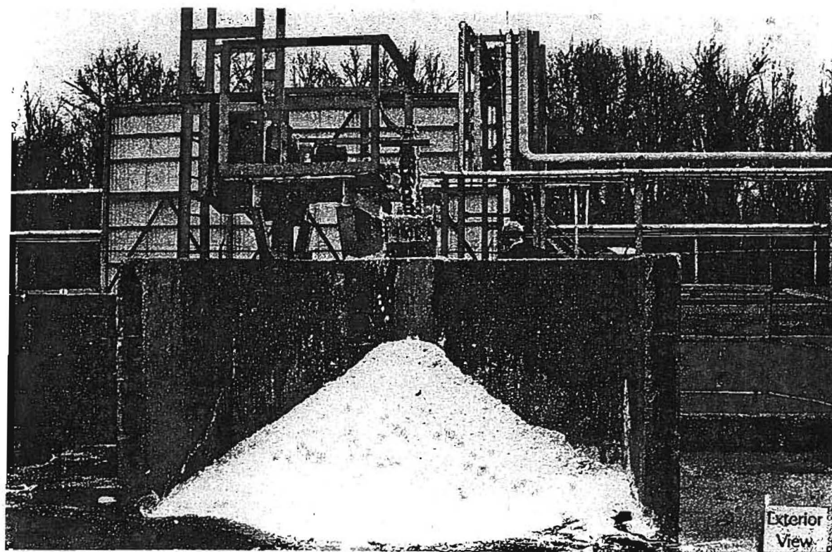
Figure 11. Pellets in the First Fixed Skimmer Containment Area at Company F.
