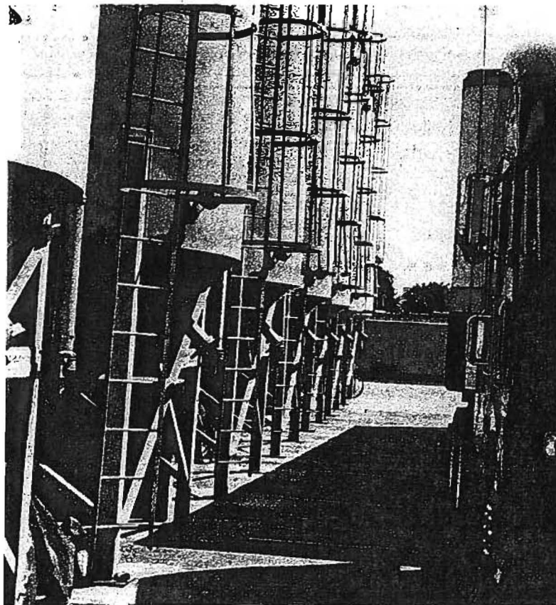
Figure 23. Primary Bulk-Storage Hoppers (Silos) at Company A.
