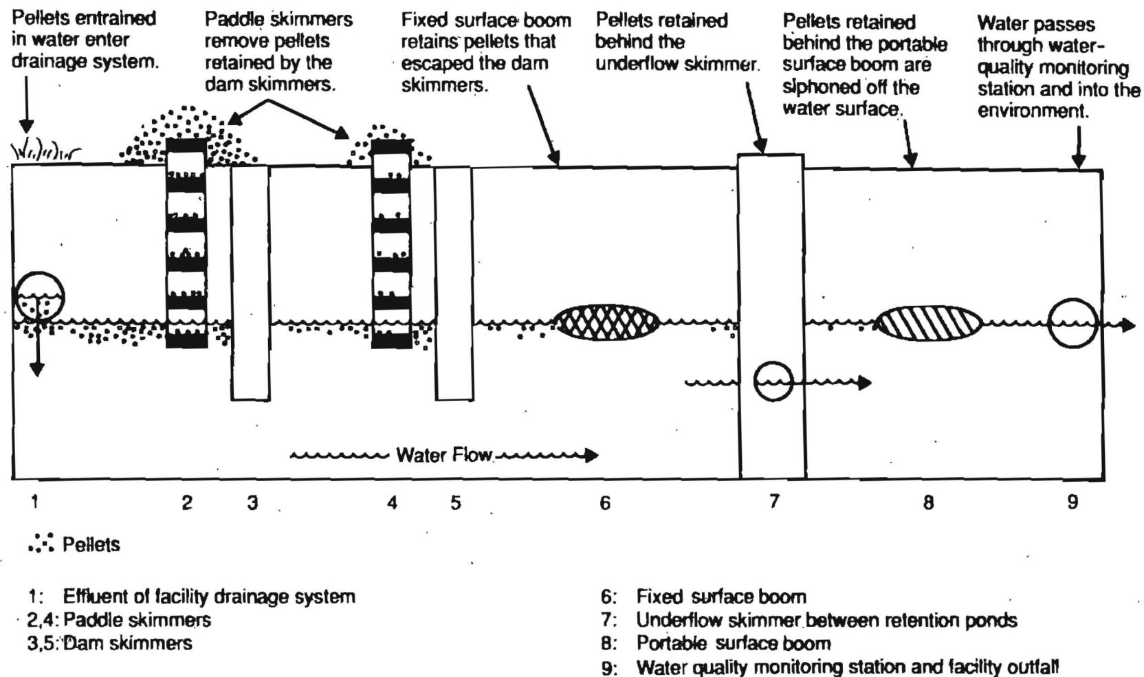
Figure 8. Basic Design of the Company F Pellet Containment System (Side View).
