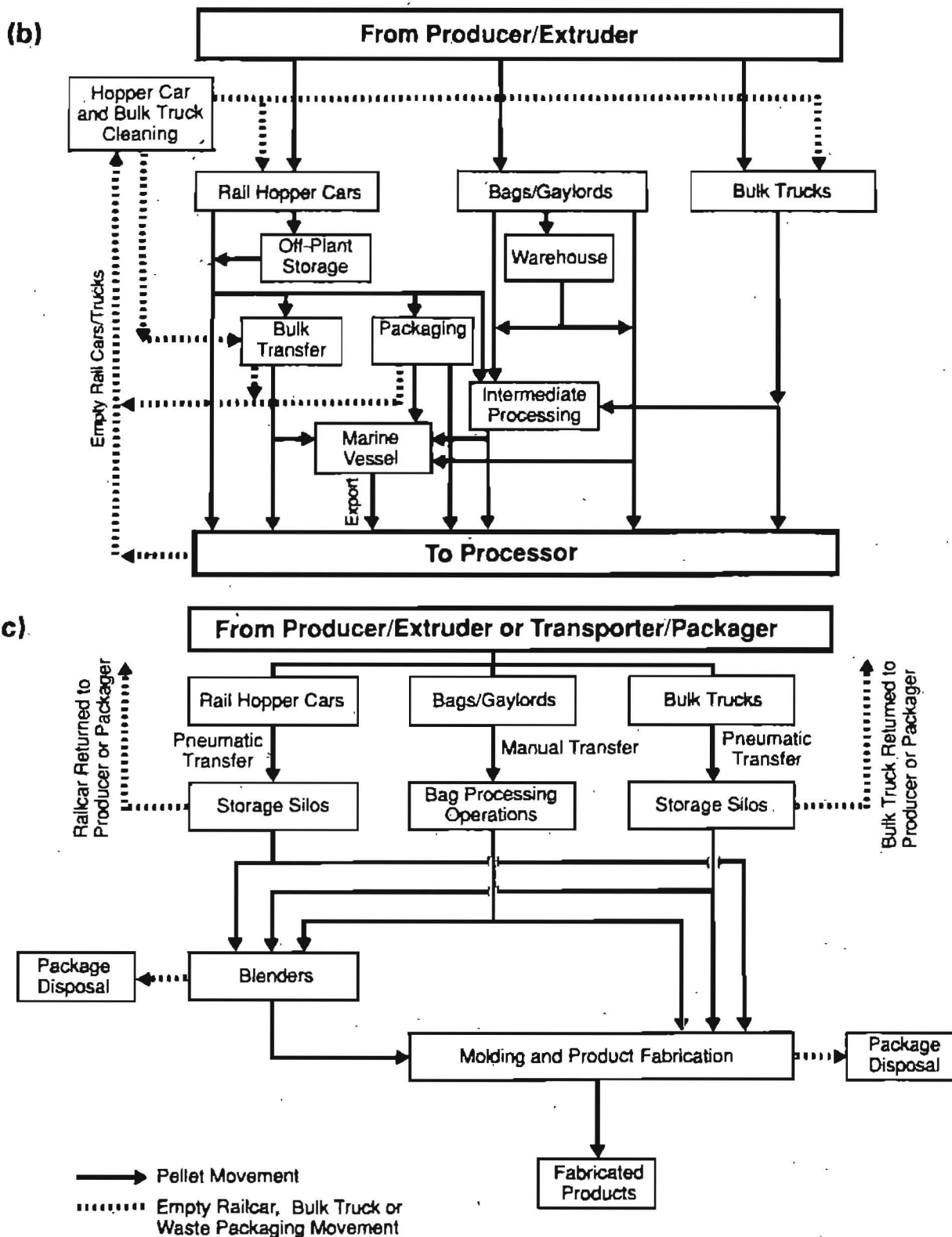
Figure 6. Pellet Flow through Plastics Industry Sectors. (continued) (b) Pellet Transporters/Packagers, (c) Pellet Processors.
