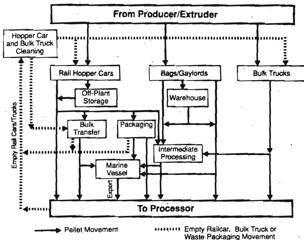
Figure 6. [Repeated] Pellet Flow through Plastics Industry Sectors. (b) Pellet Transporters/Packagers.
