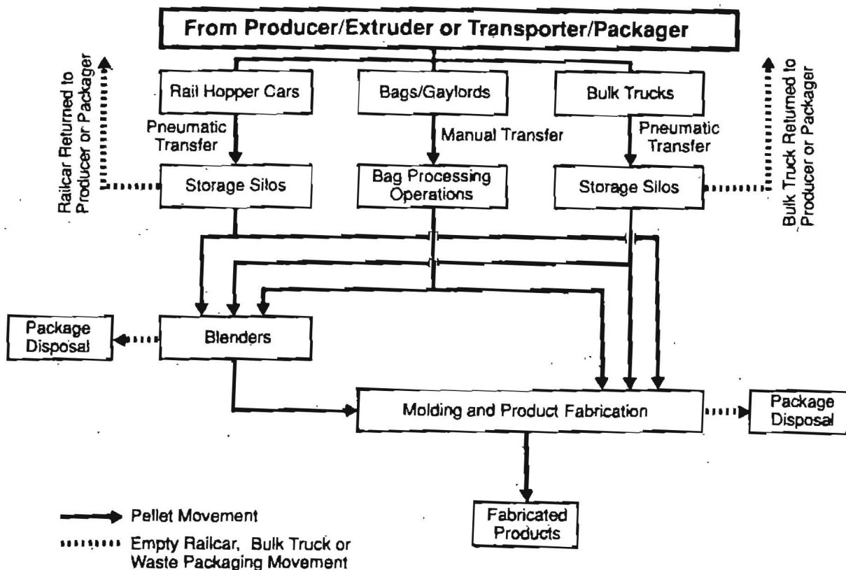
Figure 6. [Repeated] Pellet Flow through Plastics Industry Sectors. (c) Pellet Processors.
