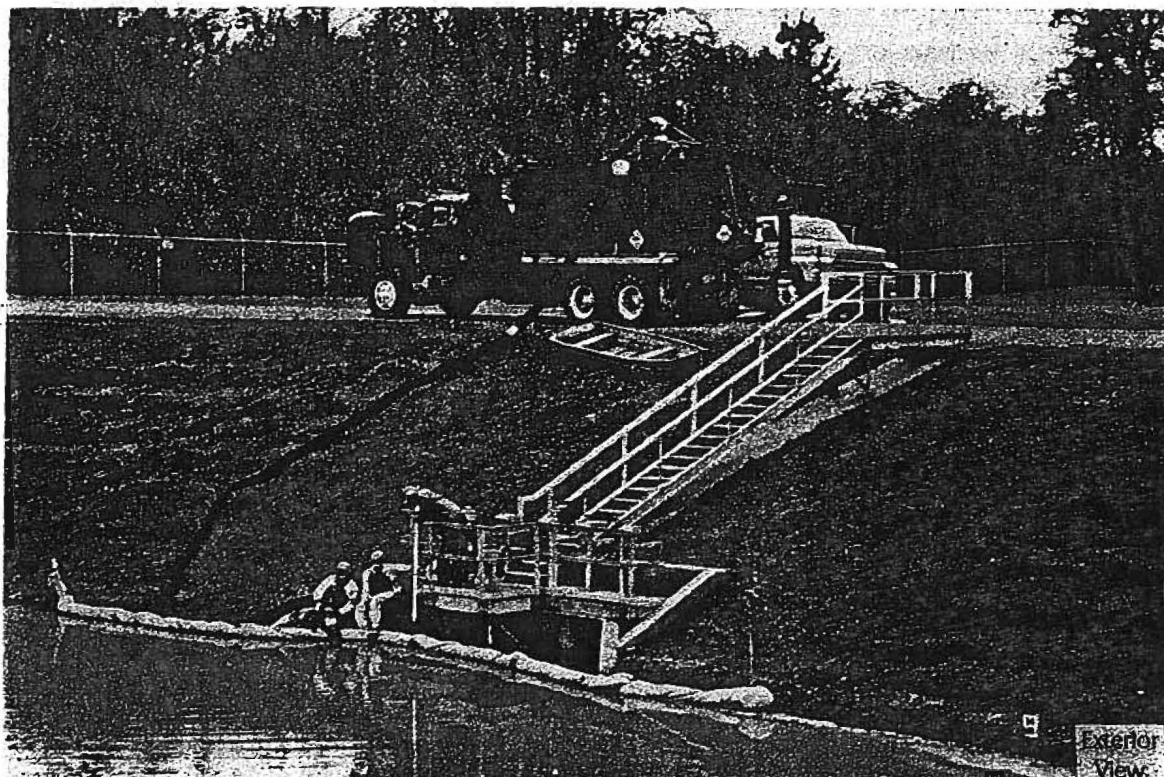
Figure 12. Portable Boom and Manual Pellet Recovery from the Company F Containment System.
