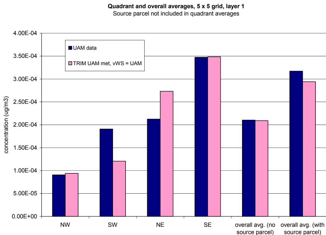
Figure 3-4 Quadrant Averages, Layer 1, 5 x 5 Grid
