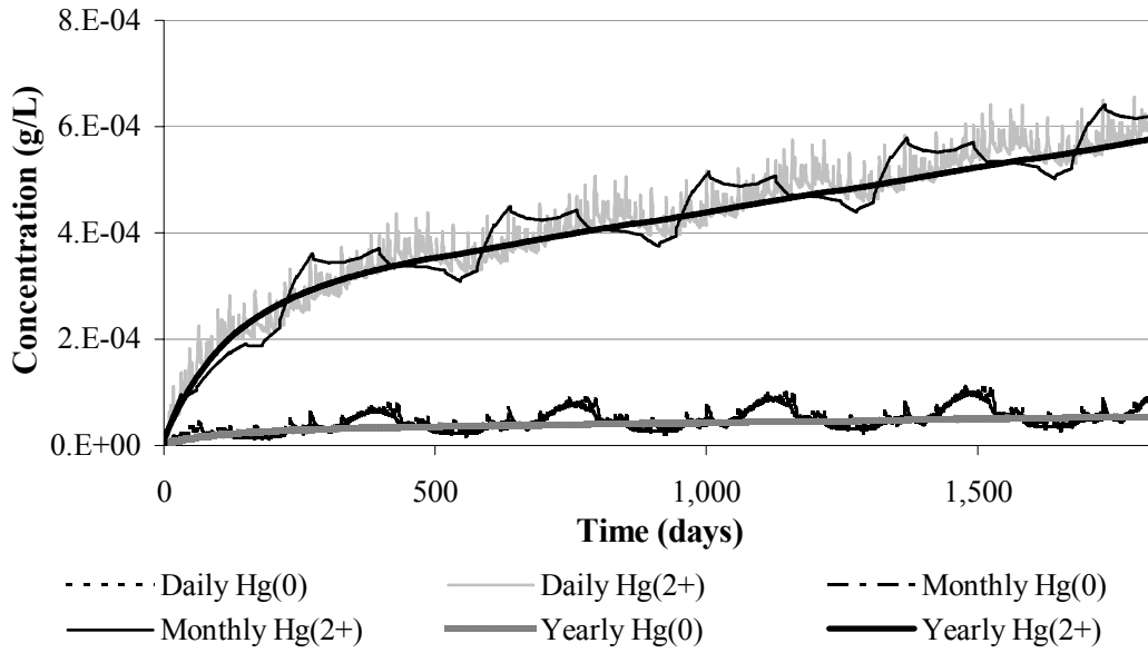
Figure 4-17 Mercury Concentrations in Surface Water
