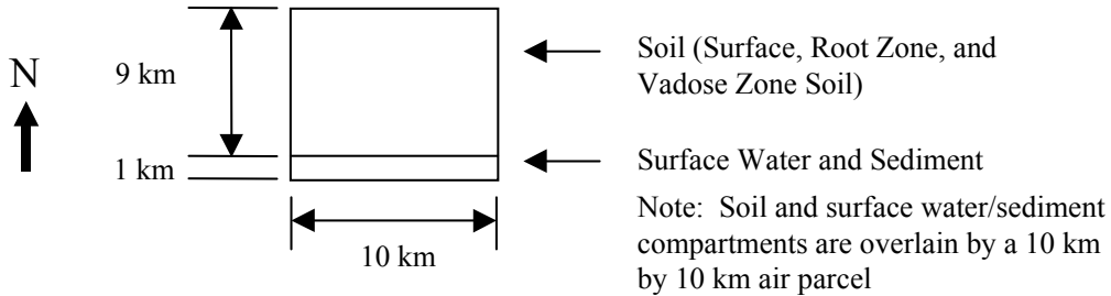
Figure 4-8 Modeling Configuration for the Biotic Complexity Evaluation With Mercury Horizontal Dimensions
