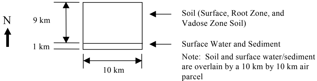
Figure 4-6 Modeling Configuration for the Biotic Complexity Analysis with Benzo(a)pyrene Horizontal Dimensions
