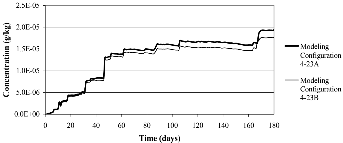
Figure 4-24 Benzo(a)pyrene Concentration in Surface Soil at Target Parcels of Modeling Configurations 4-23A and 4-23B
