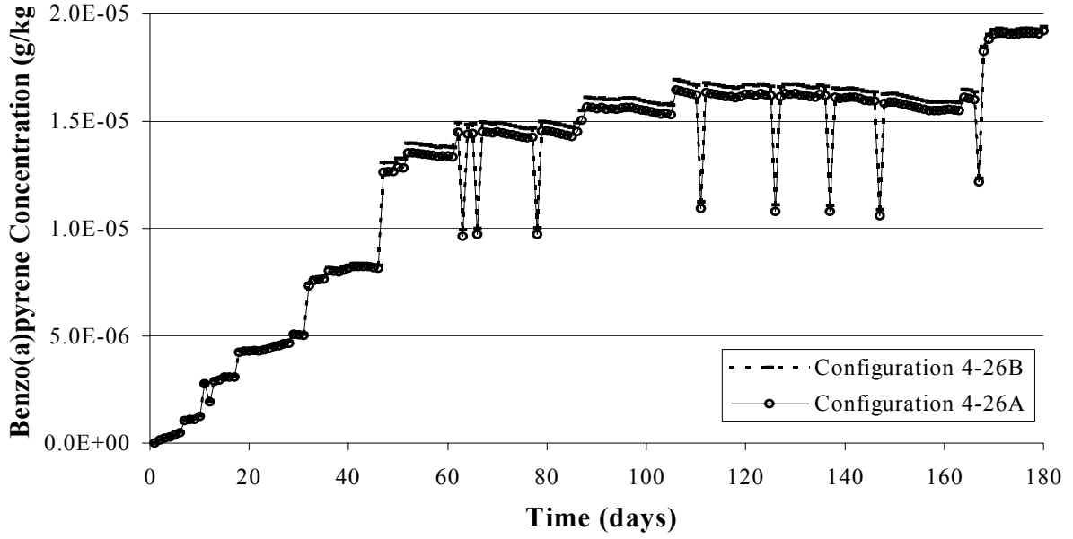
Figure 4-27 Surface Soil Concentrations in the Target Parcels of Modeling Configurations 4-26A and 4-26B
