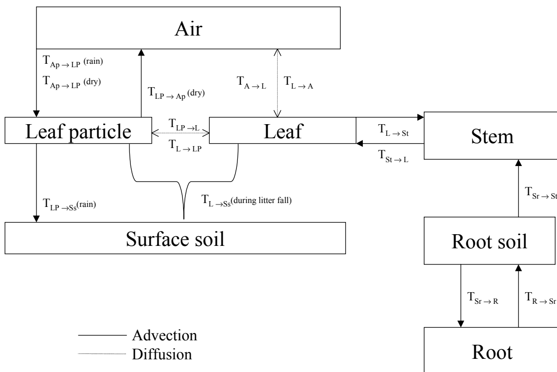
Figure 3-6 Schematic of the Plant Module
