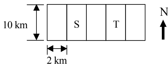
Figure 4-12 Modeling Configuration B
