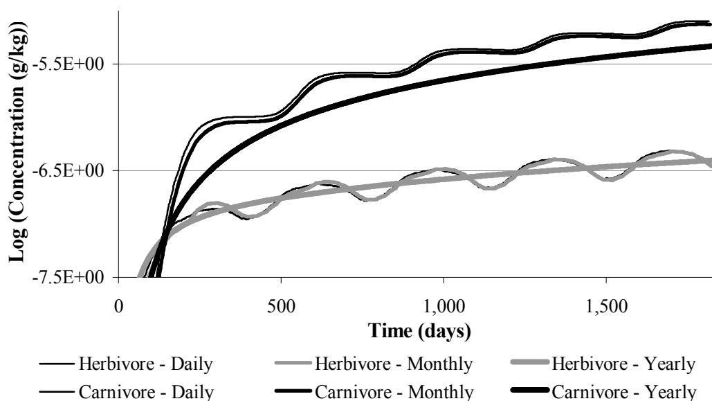
Figure 4-19 Methylmercury Concentrations in Water Column Herbivore and Carnivore Fish
