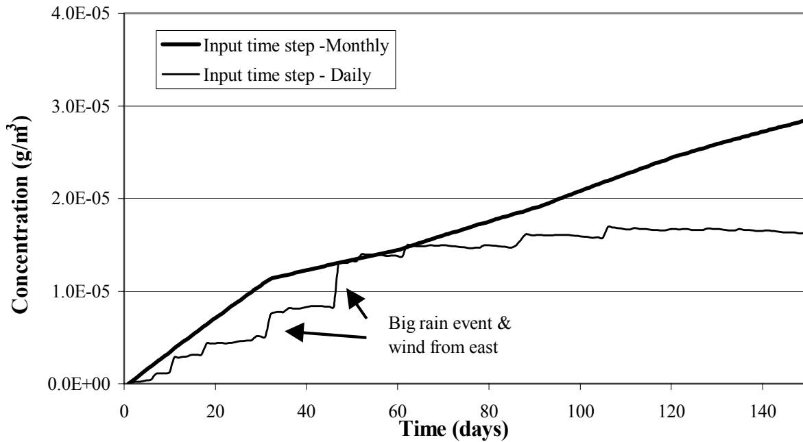
Figure 4-16 Benzo(a)pyrene Surface Soil Concentrations for Modeling Configuration C-Target Location
