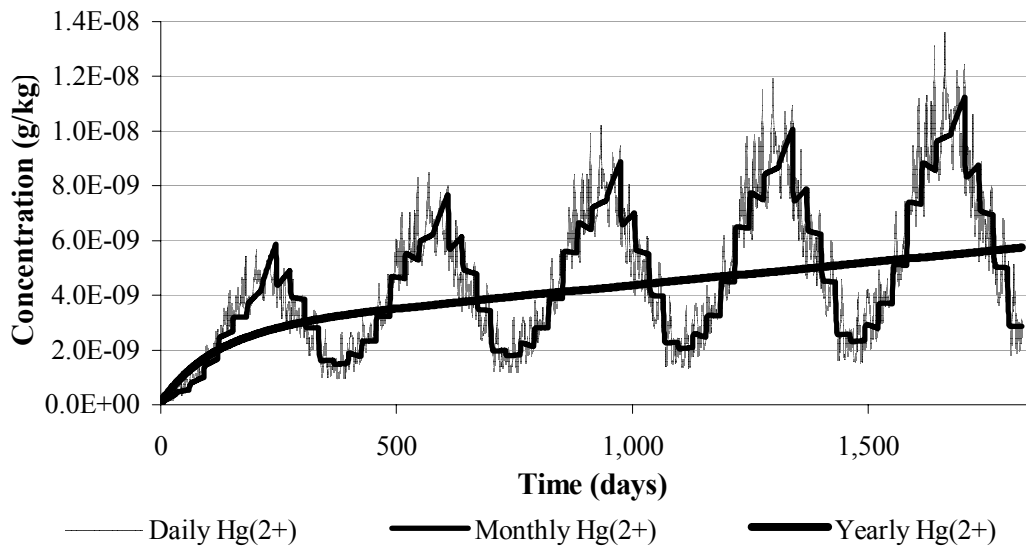
Figure 4-18 Divalent Mercury Concentrations in the Water Column Herbivore Compartment
