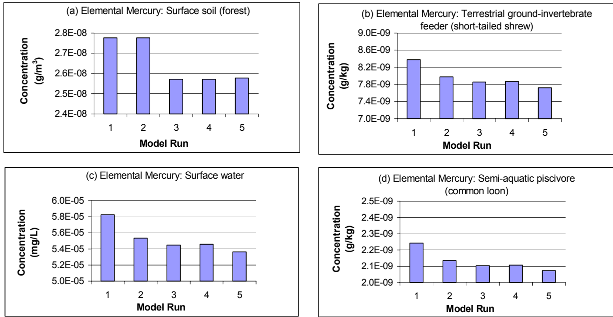
Figure 4-9 Elemental Mercury Concentrations in Selected Compartments After Five Years
