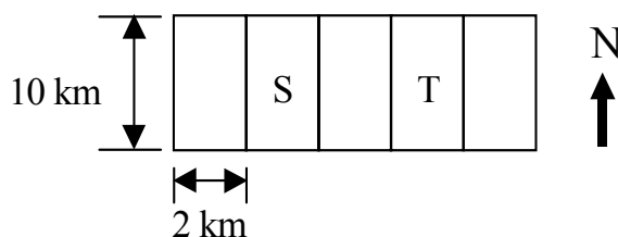
Figure 4-20 Modeling Configuration for the Evaluation of Effects of Distance From Source
