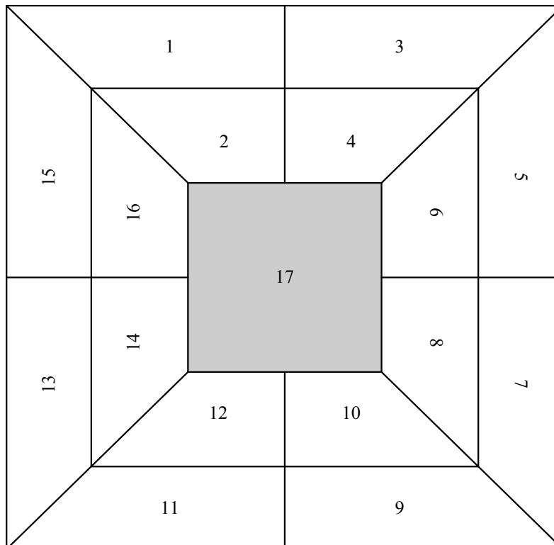
Figure 4-2 Example of Approximated Polar Grid Layout (the shaded parcel is the source location)
