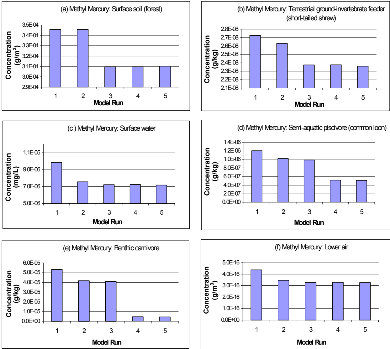
Figure 4-11 Methylmercury Concentrations in Selected Compartments After Five Years
