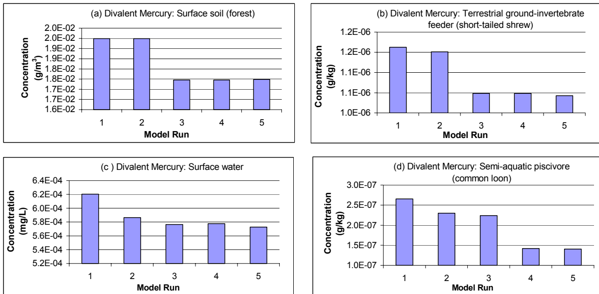
Figure 4-10 Divalent Mercury Concentrations in Selected Compartments After Five Years
