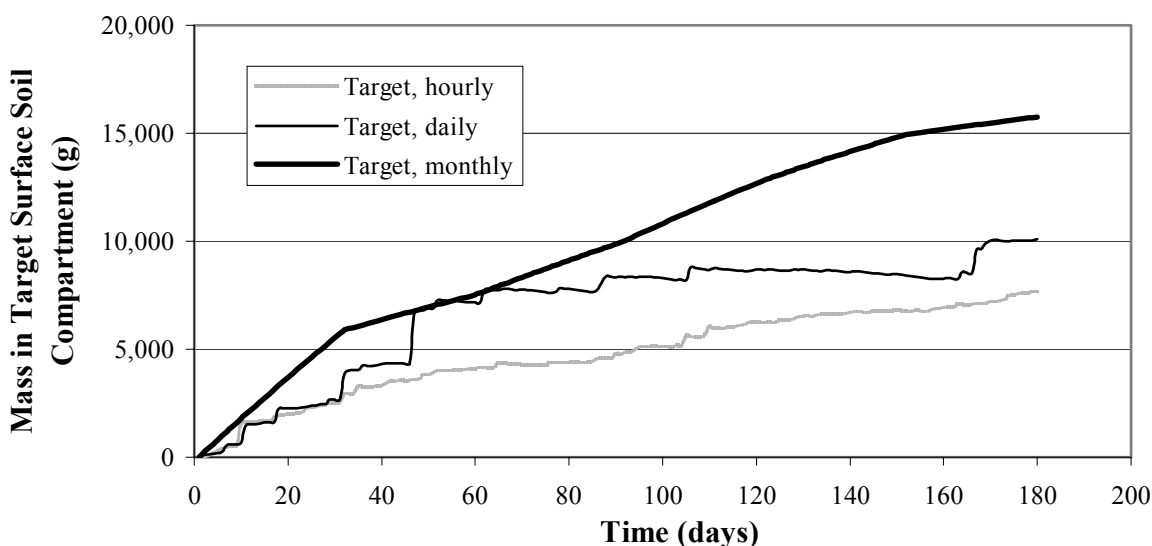
Figure 4-14 Benzo(a)pyrene Mass in Target Surface Soil Parcel, Modeling Configuration B
