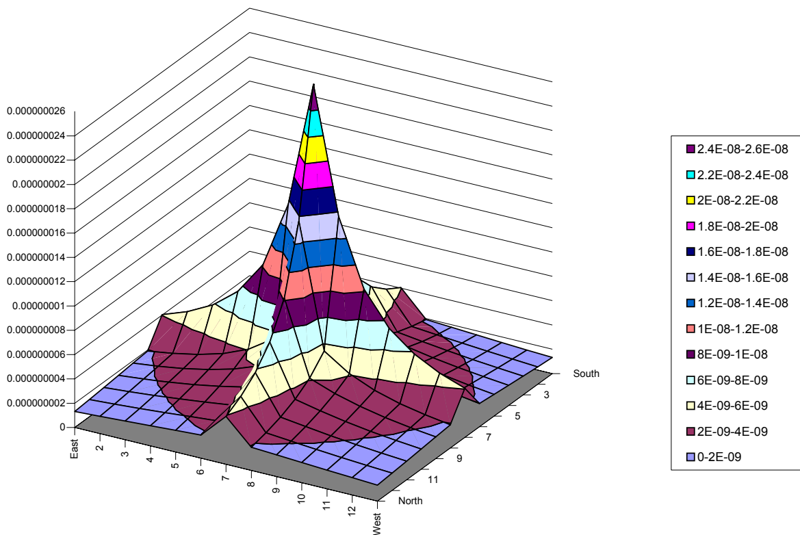
Figure 4-3 Monthly Air Concentrations ( g/m^3 ), Controlled Meteorology Data
