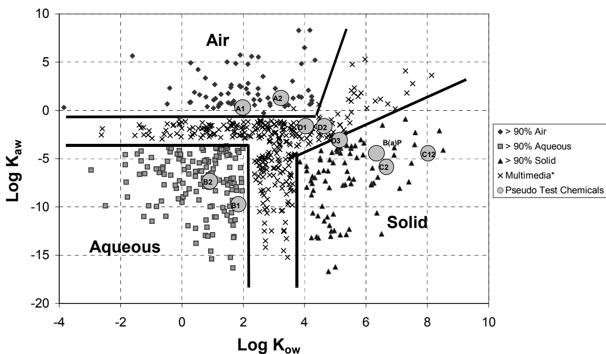
Figure 3-1 Single-Medium and Multimedia Chemical Regions for 500 Hypothetical Chemicals
