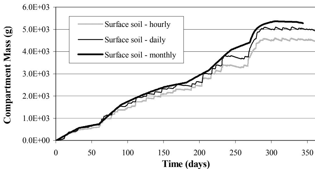
Figure 4-13 Benzo(a)pyrene Mass in Surface Soil Compartment for Various Input Averaging Times
