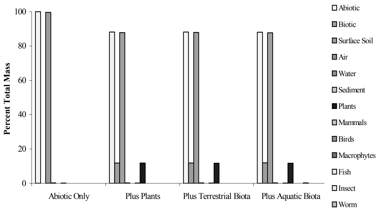
Figure 4-7 Benzo(a)pyrene Mass in Biotic and Abiotic Compartments
