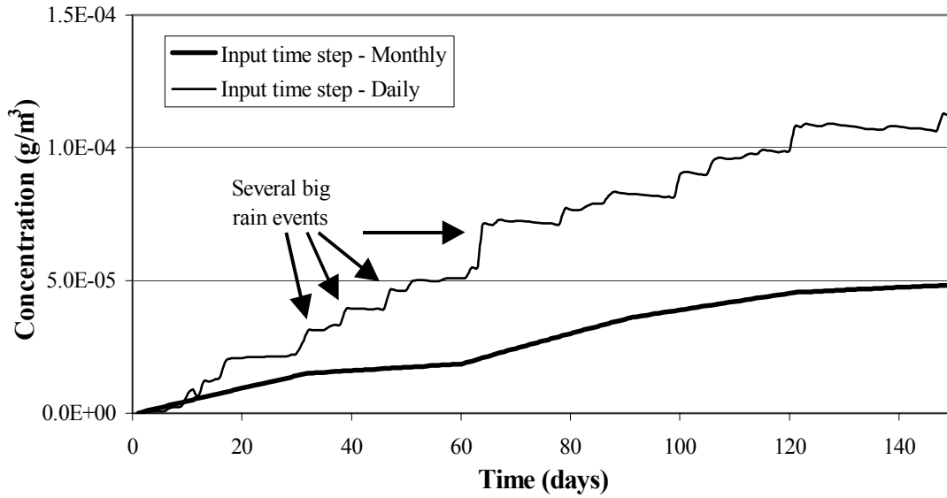
Figure 4-16 Benzo(a)pyrene Surface Soil Concentrations for Modeling Configuration C-Target Location
