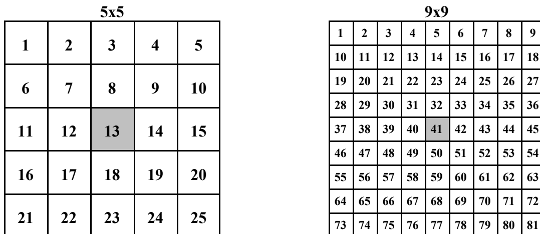
Figure 3-2 Grid Configurations (source parcels are shaded)
