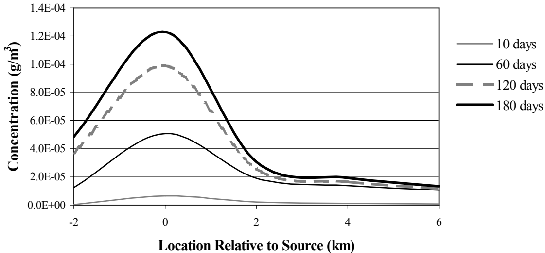
Figure 4-21 Benzo(a)pyrene Concentrations in Surface Soil for Evaluation of Effects of Distance from Source a
