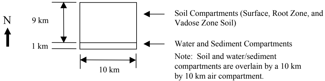
Figure 3-7 Modeling Configuration for Evaluation of Concentrations and Flows through Terrestrial Wildlife Horizontal Compartment Dimensions
