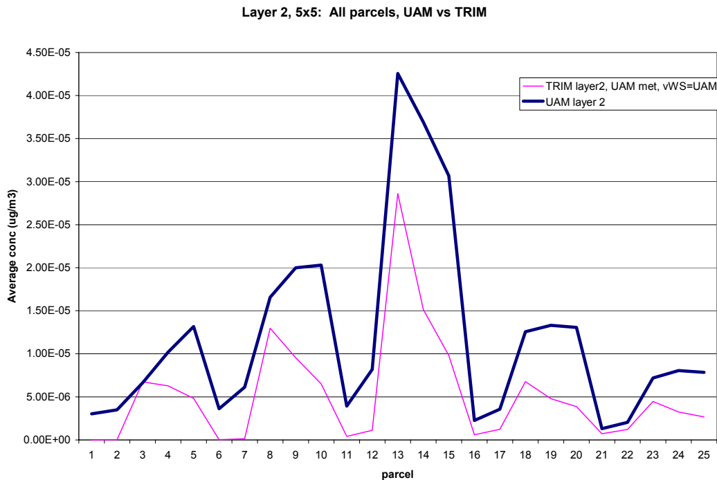
Figure 3-5 TRIM.FaTE and UAM Concentrations, Layer 2, 5 x 5 Grid
