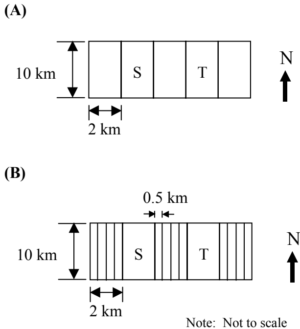
Figure 4-23 Modeling Configurations for Evaluation of the Effects of Horizontal Parcel Dimensions
