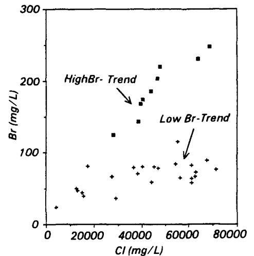
Figure 4. Plot of bromide versus chloride from brines collected for this study for Frio Formation. Note two different populations of data. High Br trend from central and south Texas regions suggests leakage of brine from deeper geopressed sediments. The low Br trend from northern Houston embayment region results from halite dissolution.
