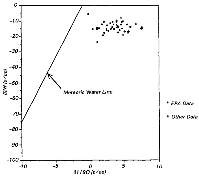
Figure 6. Hydrogen versus oxygen isotopic composition of Frio waters collected for this study. Global meteoric water line from Craig (1961).
