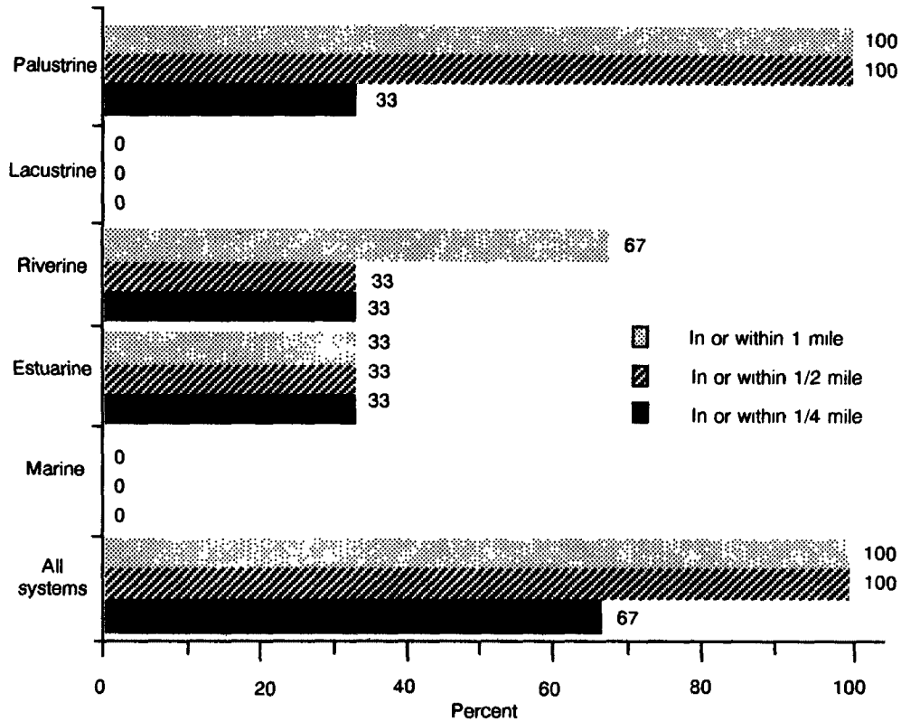
Figure 3. Proximity of 3 Delaware sanitary landfills to either closest wetland or deepwater habitat.
