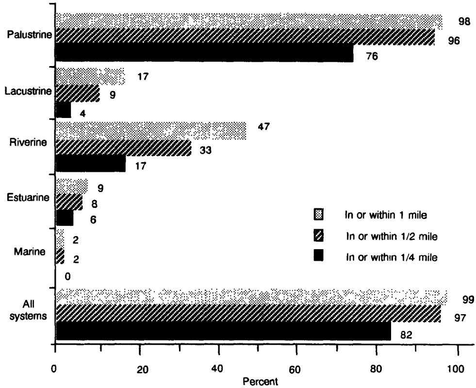
Figure 3. Proximity of 110 New York sanitary landfills to either closest wetland or deepwater habitat.
