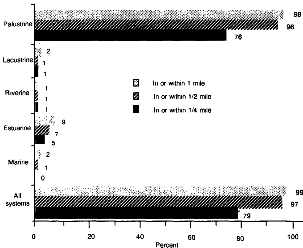
Figure 1. Proximity of 110 New York sanitary landfills to wetlands.
