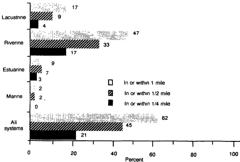
Figure 2. Proximity of 110 New York sanitary landfills to deepwater habitats.
