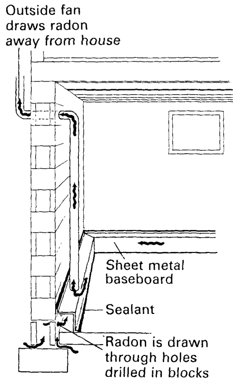
Baseboard Approach
