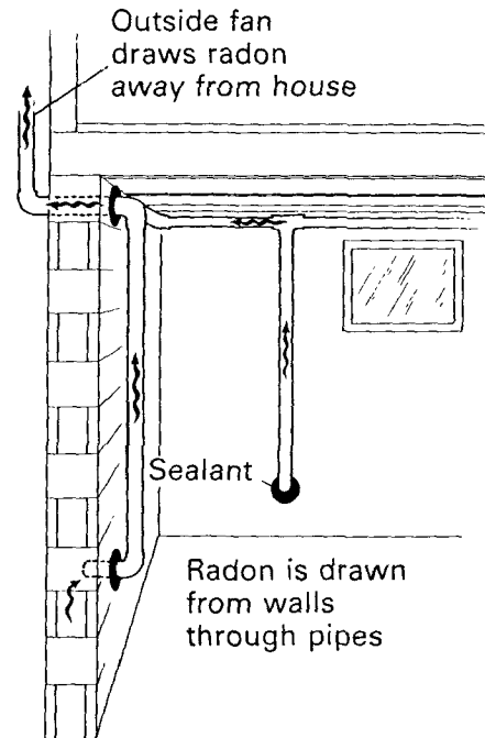
Pipe-in-Wall Approach
