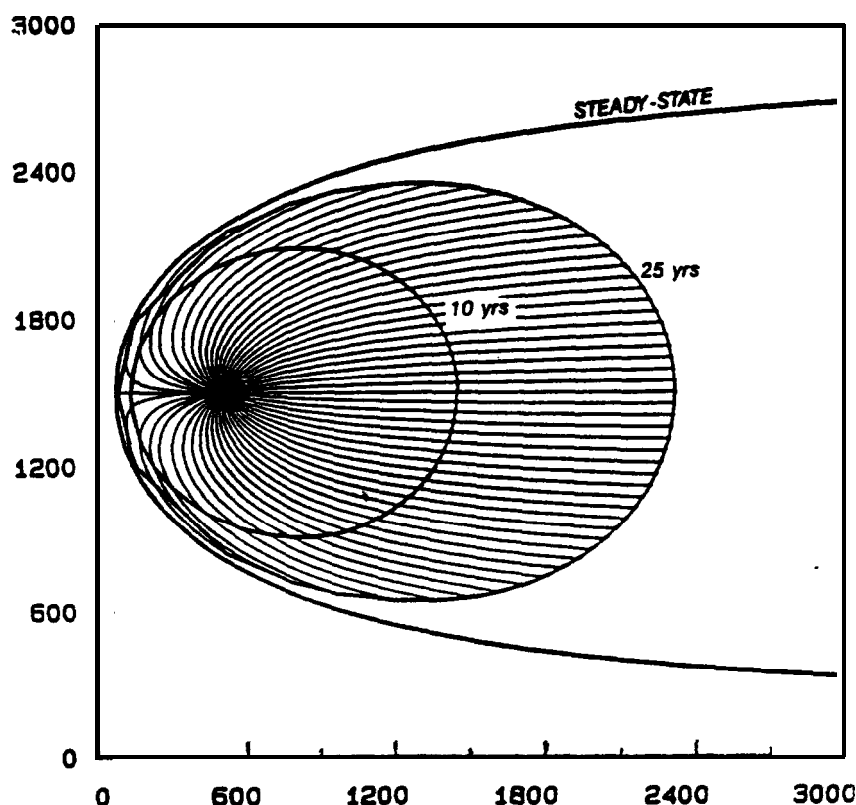
Figure 2-14. Example of steady-state, and 10-year and 25-year time-related capture zones delineated using reverse particle tracking (from Blandford and Huyakom, 1989).
