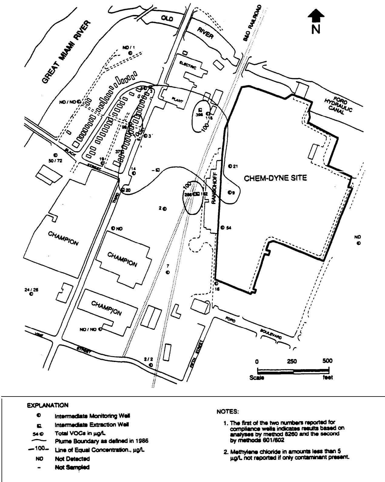
Figure 5-8. Concentration of VOCs in the intermediate interval in December 1992 at the Chem-Dyne site (from Papadopoulos & Assoc., 1993).
