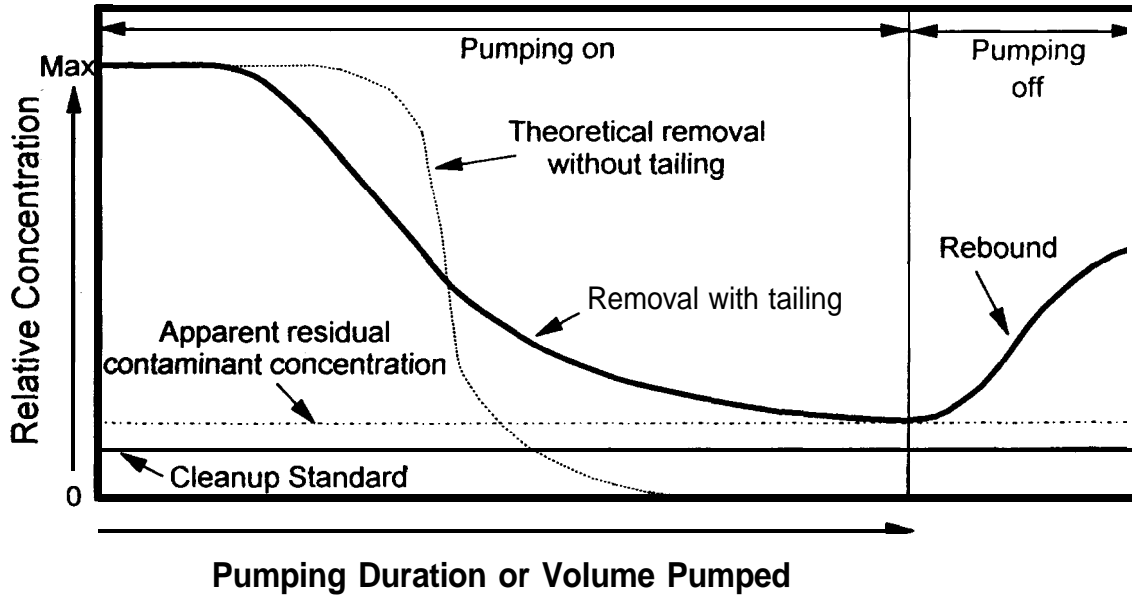
Figure 1-3. Concentration versus pumping duration or volume showing tailing and rebound effects (modified from Keeiy, 1989).
