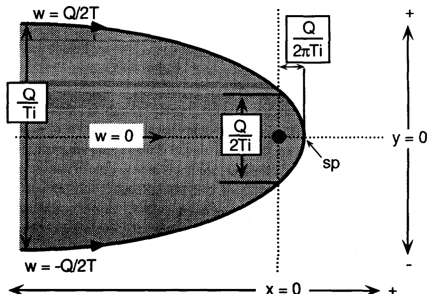
Figure 2-12. Equations for the dividing streamlines ( w=Q/2T ) that separate the capture zone of a single well from the rest of an isotropic, confined aquifer with a uniform regional hydraulic gradient (modified from Gorelick et al., 1993). Note that T =transmissivity ( L^2/T ), Q =pump rate ( L^3/T ), and i =initial uniform hydraulic gradient).
