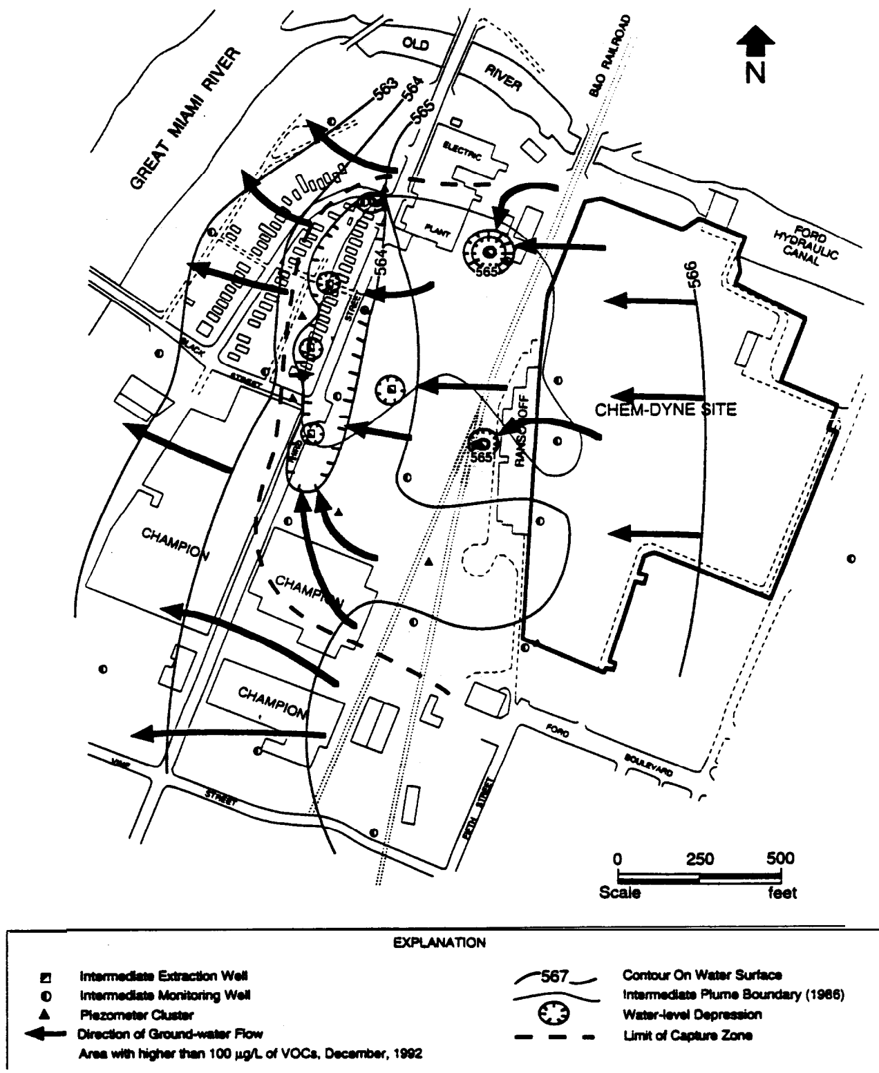
Figure 5-4. Average potentiometric surface and direction of ground-water flow in the intermediate interval in 1992 at the Chem-Dyne site (from Papadopolulos & Assoc., 1993).
