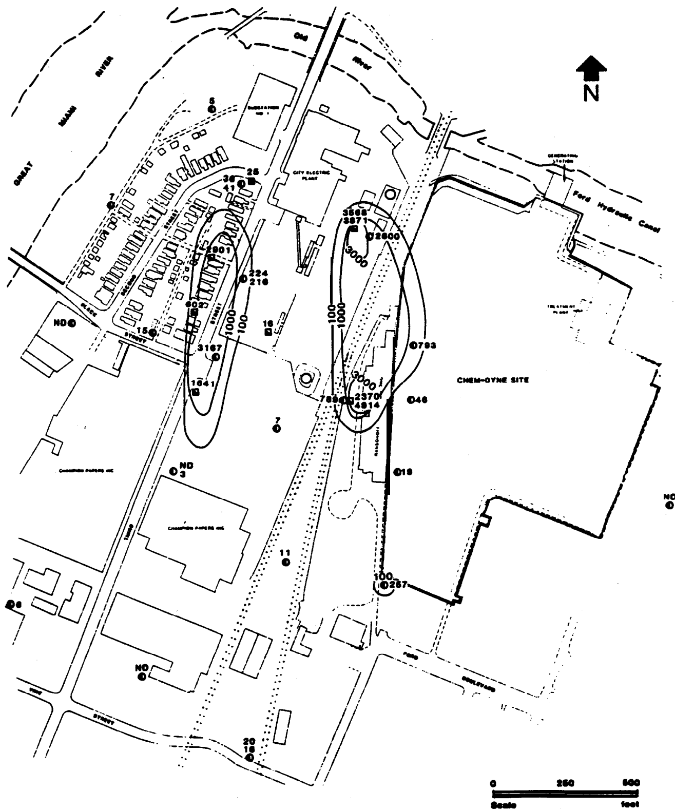
Figure 5-10. Concentrations of VOCs in \mu\text{g/L} in the intermediate interval during October/November 1987 (from Papadopoulos & Assoc., 1988).
