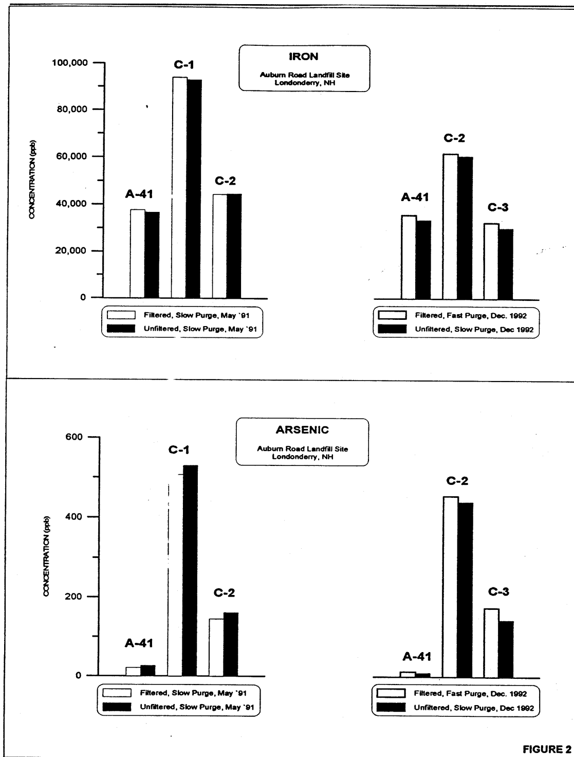
Figure 2. Comparison of filtered vs. unfiltered, slow purge and filtered, fast purge unfiltered, slow purge in different wells for iron (top) and arsenic (bottom).
