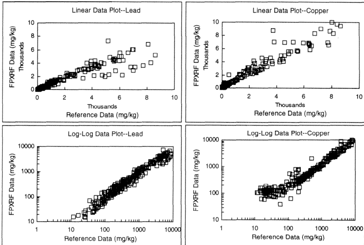
Figure 2-2. Linear and Log-log Data Plots--X-MET 920-P and 940 Analyzers: These graphs illustrate the linear relationship between the X-MET 920-P and 940 analyzer data and the reference data. The linear data plots illustrate the concentration dependence of this relationship with increased scatter at higher concentrations. The log-log plots eliminate this concentration effect. Scatter is relatively constant over the entire plot.
